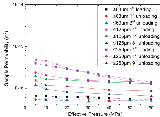
Figure 8. Comparison of the effect of pressure cycling on the same thickness (0.6 mm here) of gouges with coarse grains ( \leq 125\ \mu\text{m} and \leq 250\ \mu\text{m} here) with that of fine-grained gouge ( \leq 63\ \mu\text{m} , dashed line) as the baseline. Square, circle, and triangle symbols represent data after the first loading process, the first unloading process, and the final unloading process when they reach steady status, respectively.
