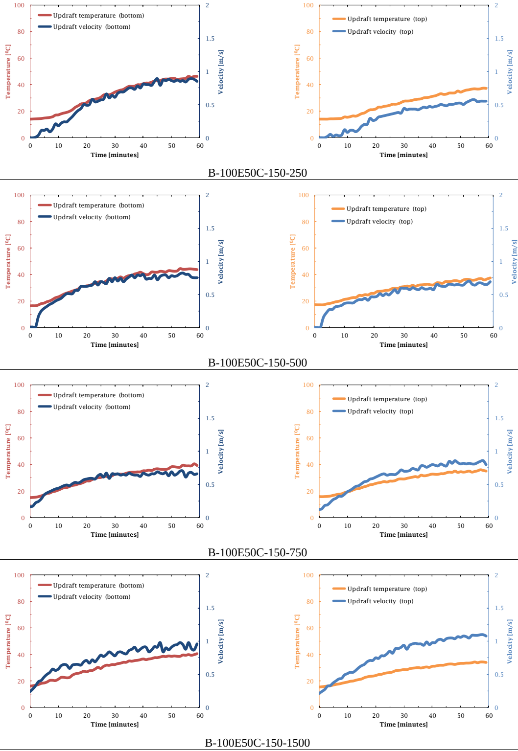
Fig. 5.24 Experimental results for the 9 th measurement group of collector type B.
