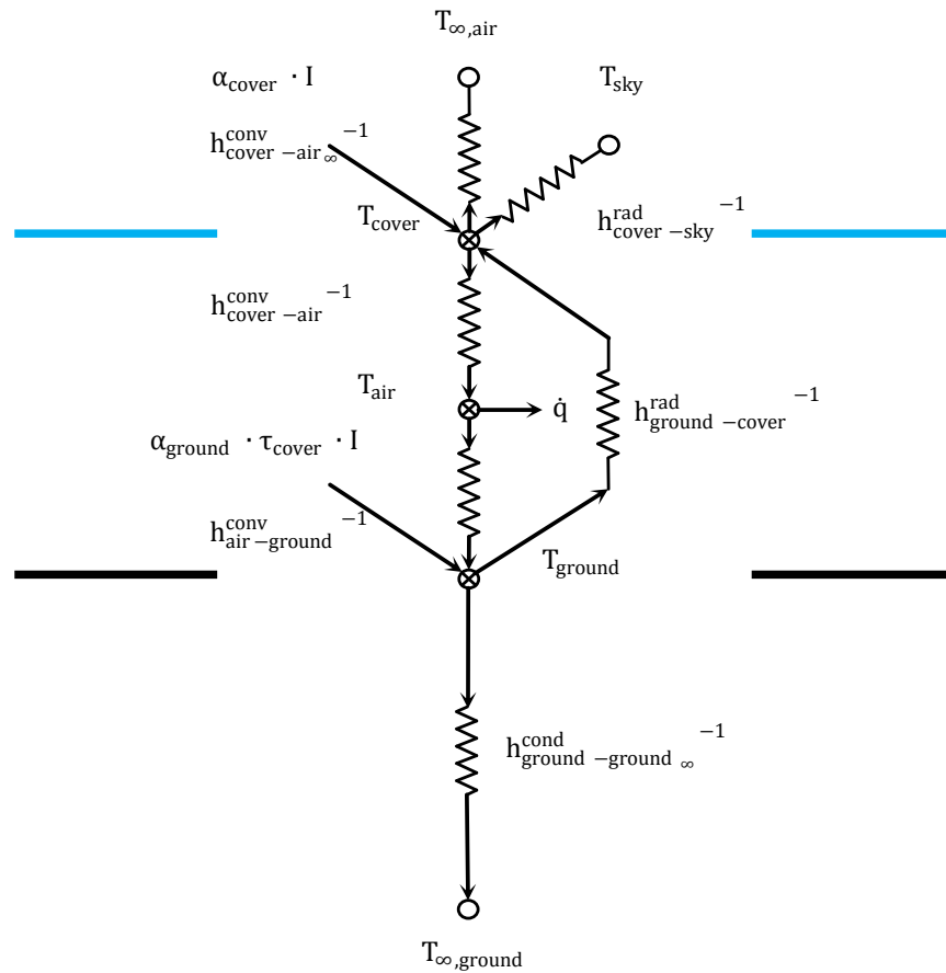
Fig. 3.15 A schematic drawing of thermal network model of Manzanares SUPG which shows the complex heat transfer process at the solar collector.
