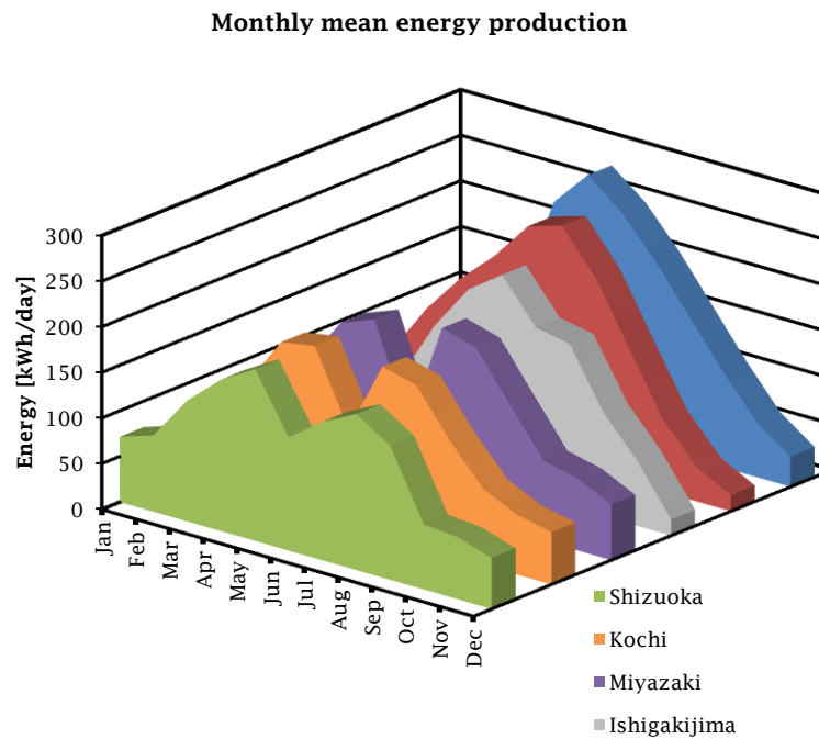
Fig. 7.2 Calculated monthly mean energy production in Japan.
