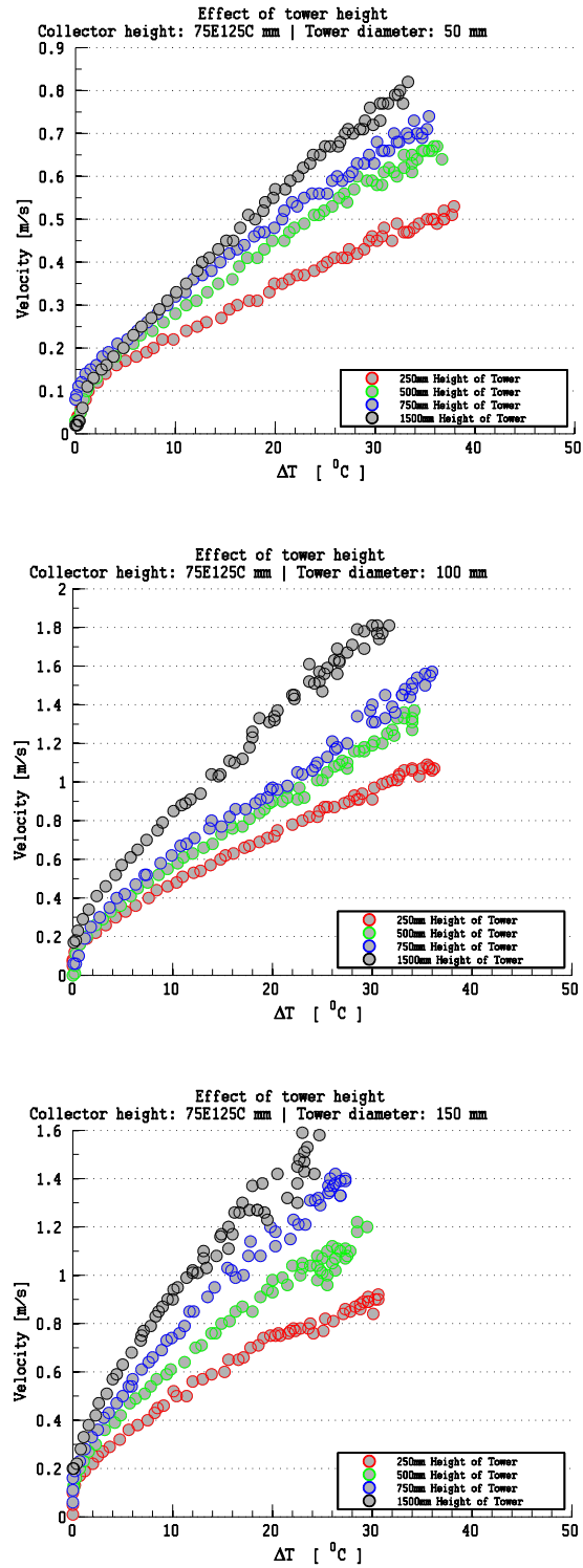
Fig. 6.5 Effects of tower height to the updraft velocity in collector type A.
