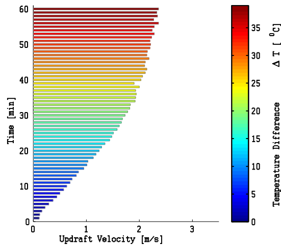
Fig. 6.10 Effects of straight guide walls to the updraft velocity in optimum configuration.
