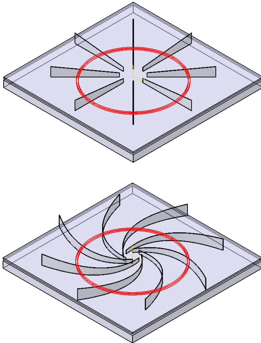
Fig. 5.4 Design of Guide Walls.
