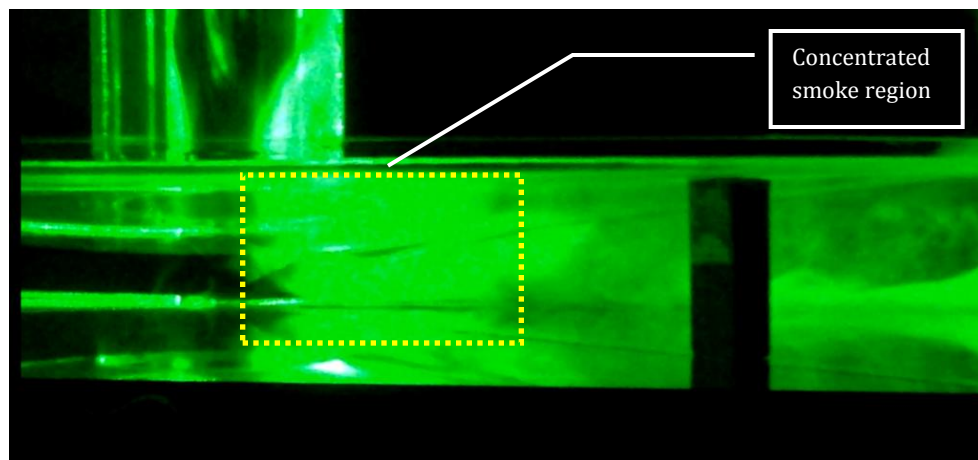
(b) Collector type B
