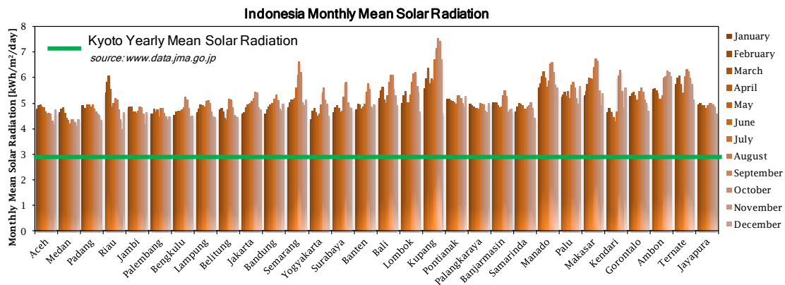
Fig. 1.4 Comparison of Indonesia monthly mean solar radiation with Kyoto yearly mean solar radiation. Data for Indonesia solar radiation are retrieved from [11] and for Kyoto solar radiation is obtained from http://data.jma.go.jp .
