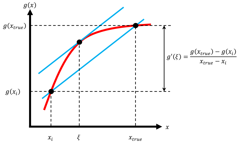
Fig. 4.1 Graphical depiction of the mean value theorem.
