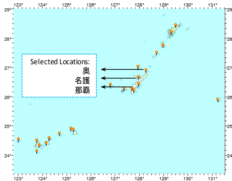
Fig. 7.4 A map of southern part of Japan showing three selected locations for daily power assessment of a 1:20 scale model Manzanares SUPG.
