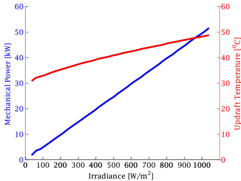
(b) Updraft temperature and mechanical power vs Irradiance
