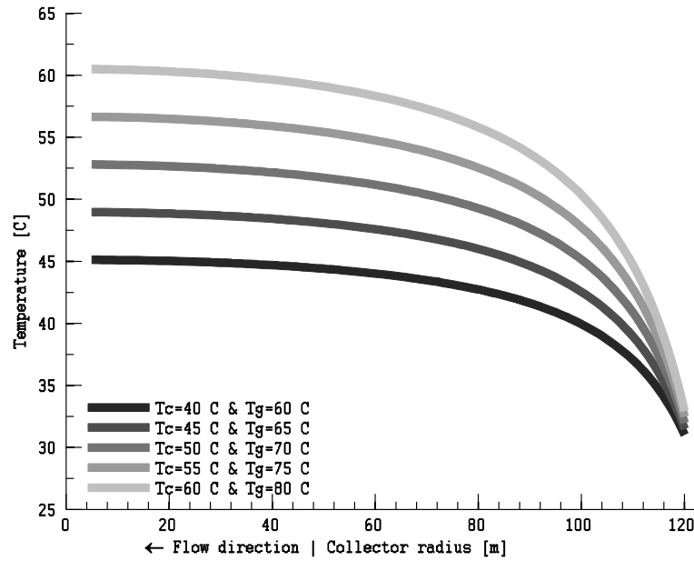
Fig. 3.8 Temperature profile of the airflow from Eq. (3.18). Values of T_c and T_g can be arbitrarily selected as long as T_g > T_c . In this work they have been selected with constant difference for the sake of simulation.
