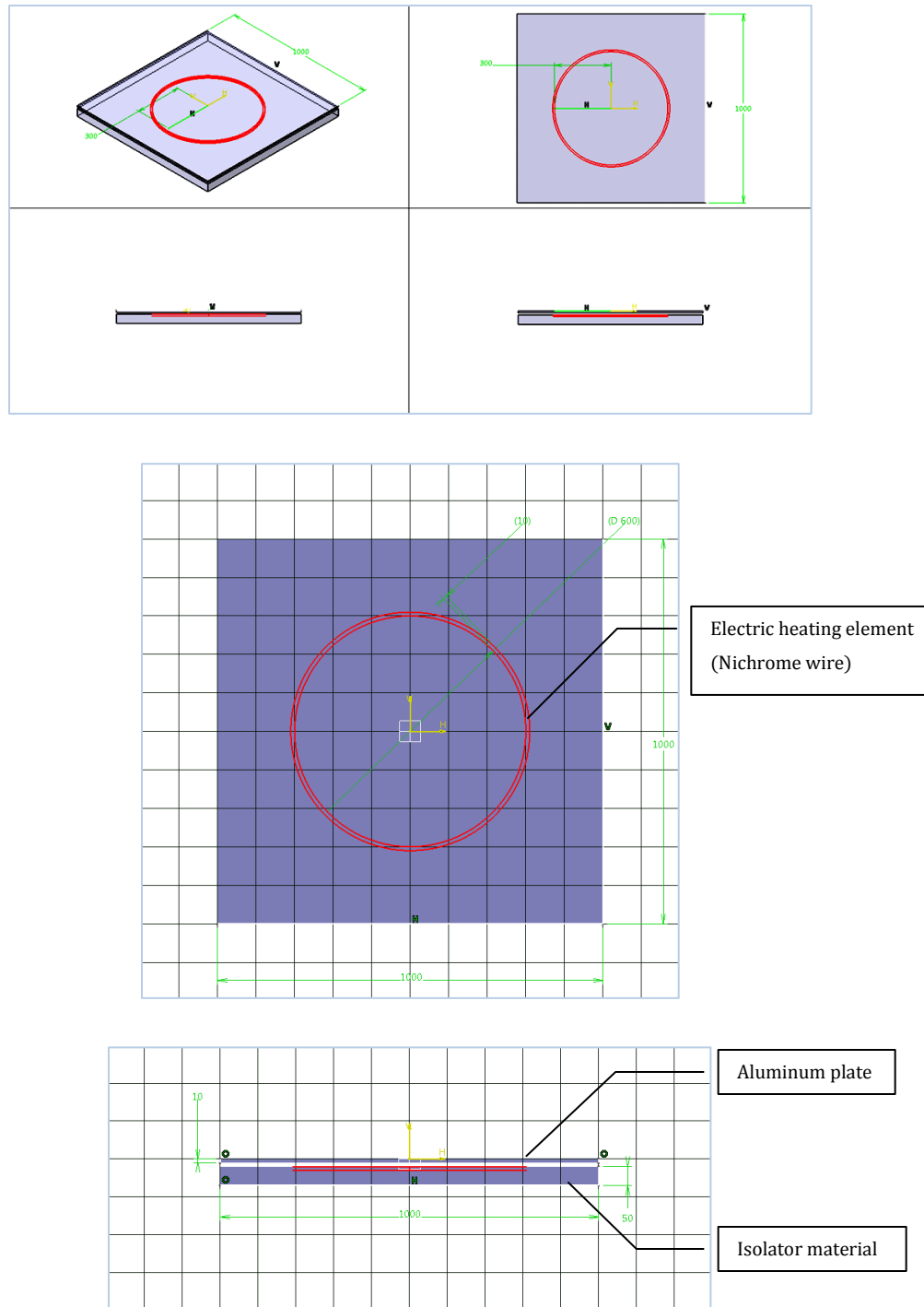
Fig. 5.1 Design of heating system.
