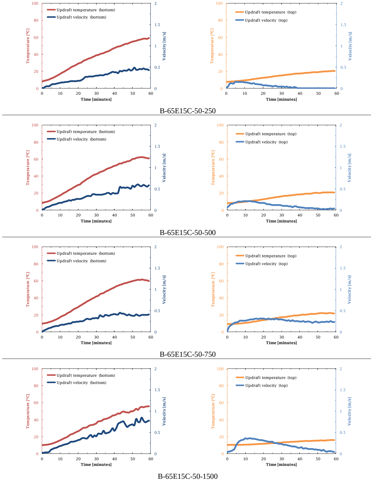
Fig. 5.16 Experimental results for the 1 st measurement group of collector type B.
