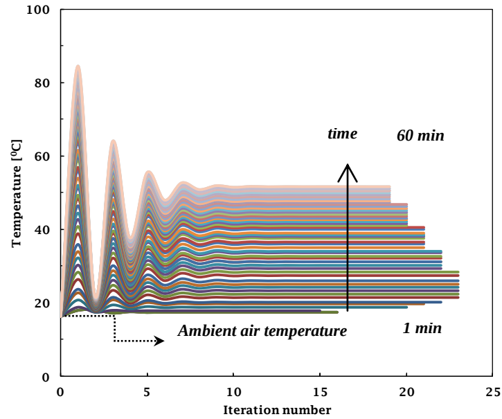
(a) Updraft temperature for each iteration number
