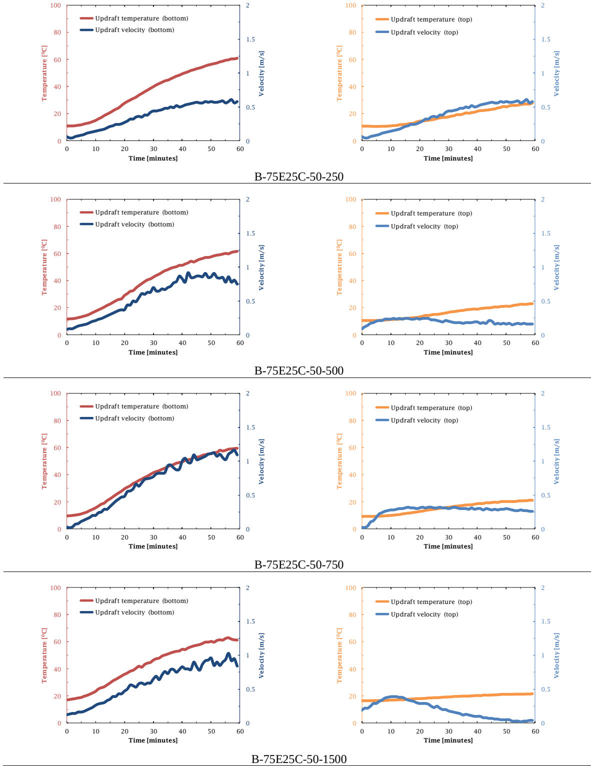
Fig. 5.19 Experimental results for the 4 th measurement group of collector type B.
