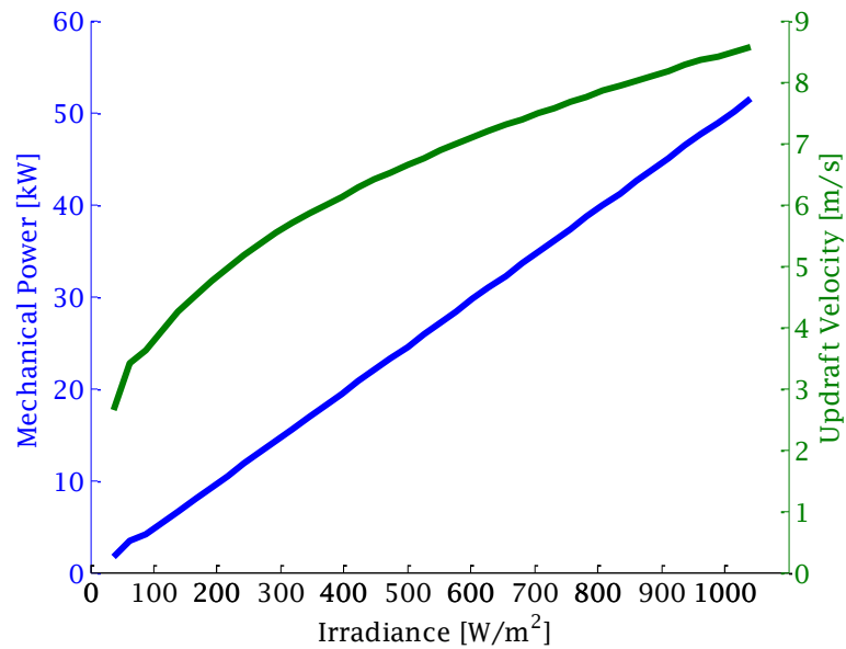
(a) Updraft velocity and mechanical power vs Irradiance
