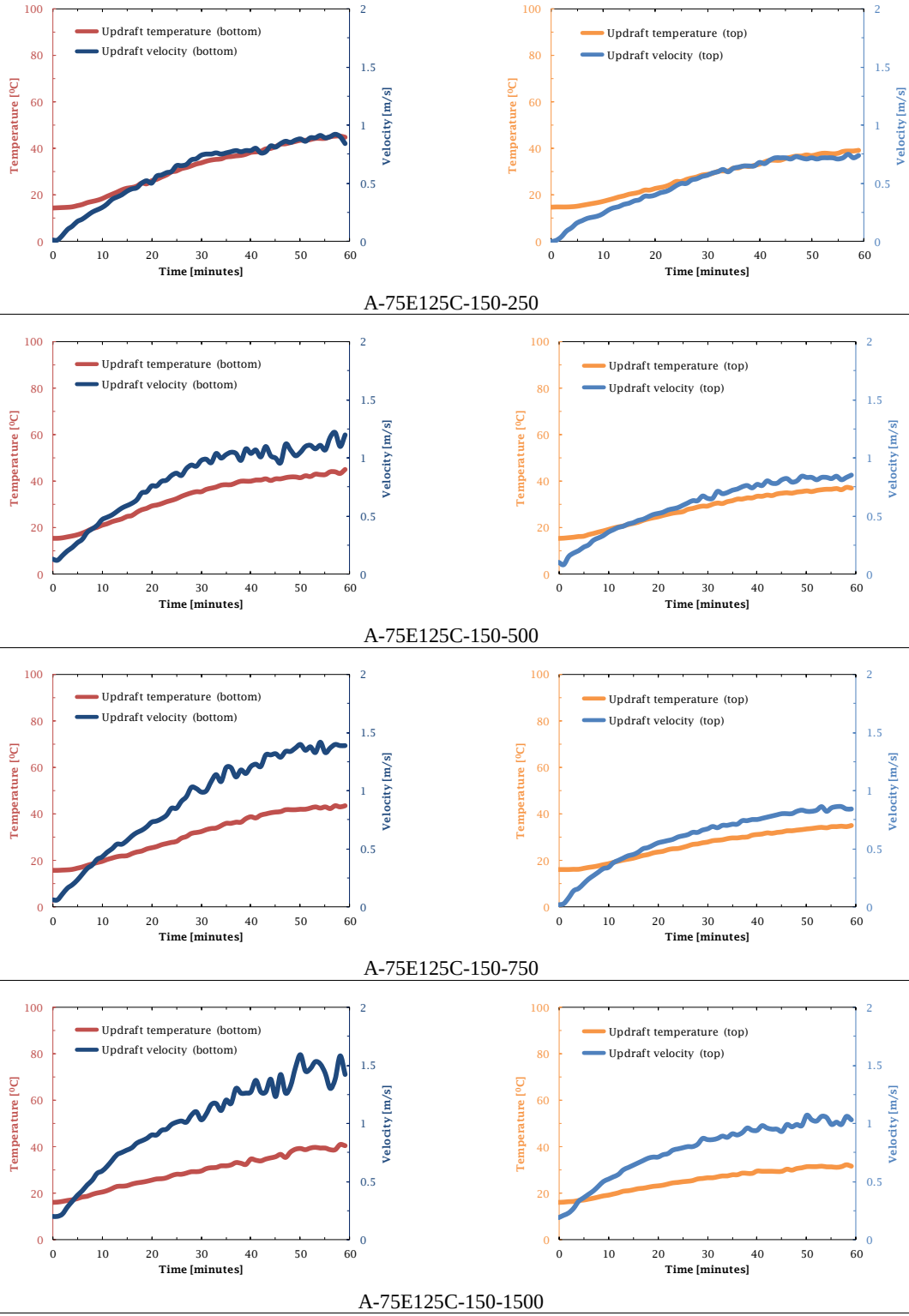
Fig. 5.15 Experimental results for the 9 th measurement group of collector type A.
