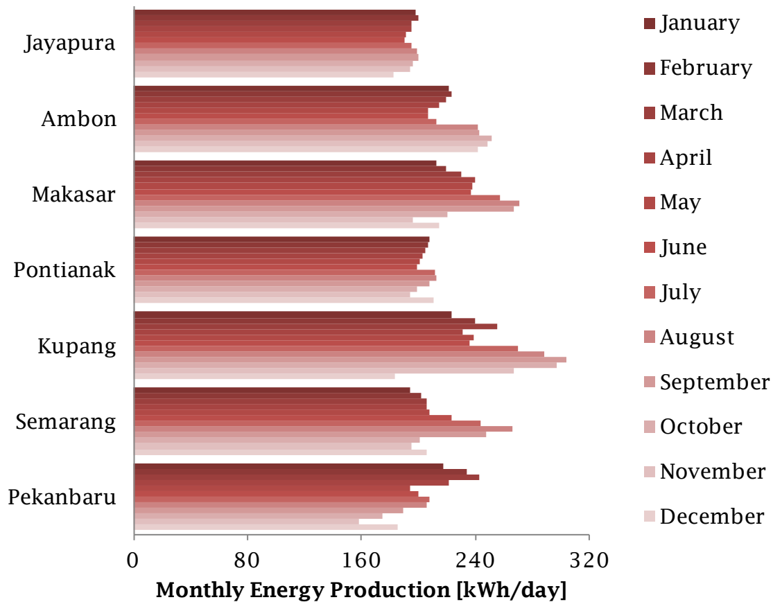
Fig 7.7 Calculated monthly mean energy production for 7 selected cities in major islands in Indonesia.
