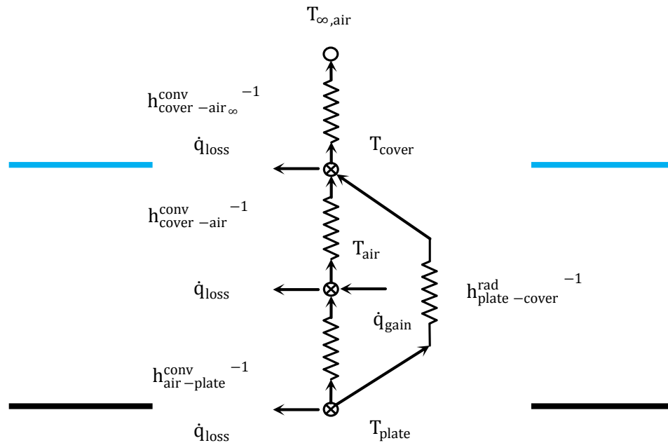
Fig. 3.16 A schematic drawing of thermal network model of lab-scale SUPG which shows the heat transfer process at the solar collector.
