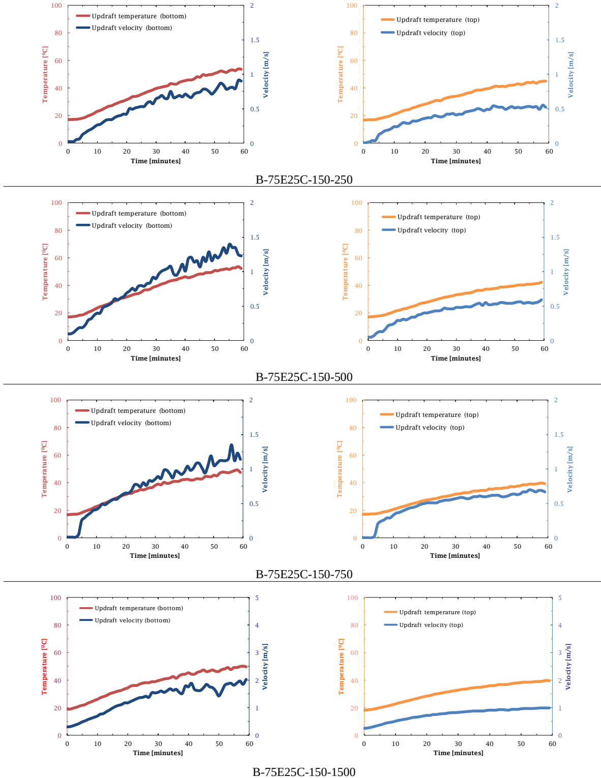
Fig. 5.21 Experimental results for the 6 th measurement group of collector type B.
