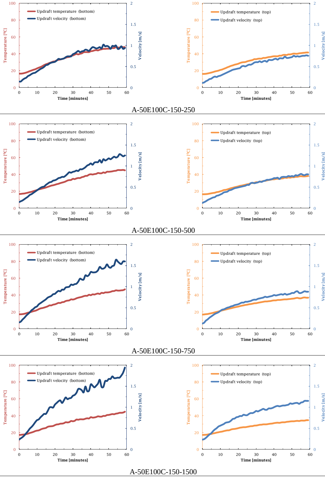
Fig. 5.12 Experimental results for the 6 th measurement group of collector type A.
