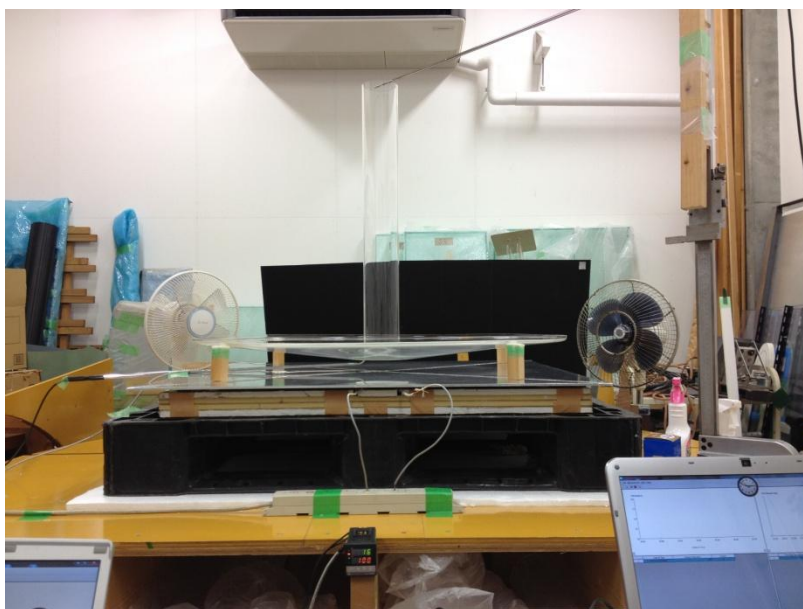
Fig. B.2 Setup of experiment for collector type B.
