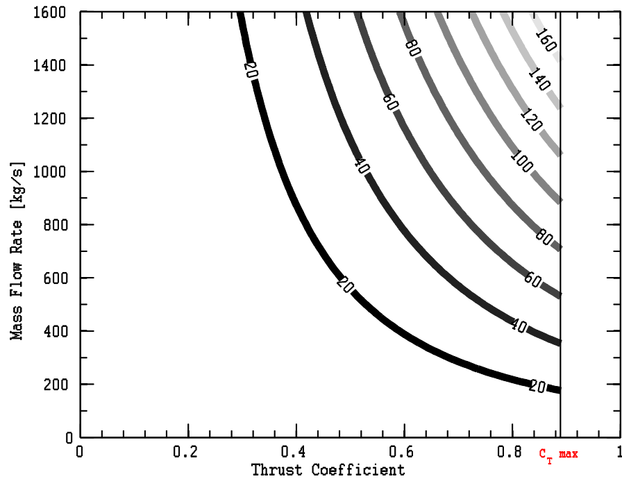
Fig. 3.13 Graphical solution of Eq. (3.48) which shows the effect of coefficient of thrust and mass flow rate to the pressure drop across the rotor blade.
