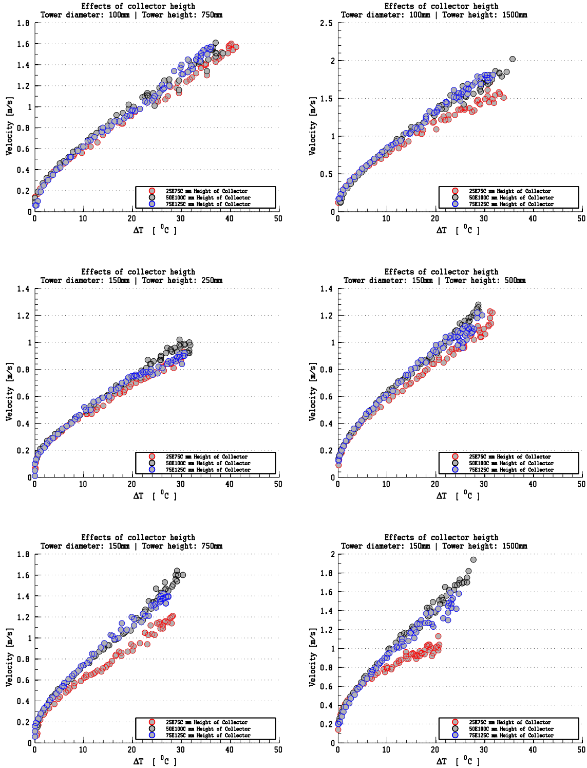
Fig. 6.1 Effects of collector height to the updraft velocity in collector type A.
