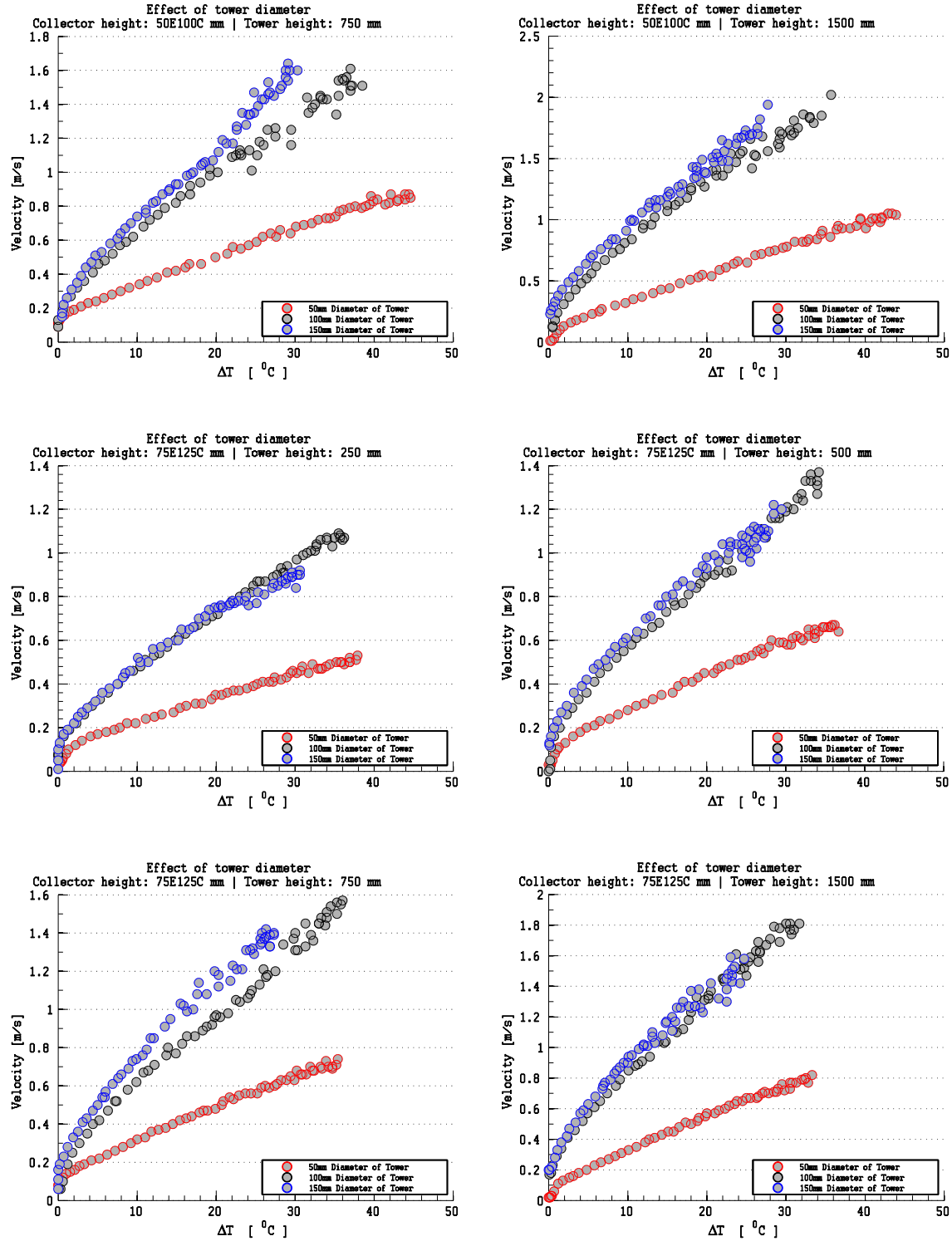
Fig. 6.3 Effects of tower diameter to the updraft velocity in collector type A.
