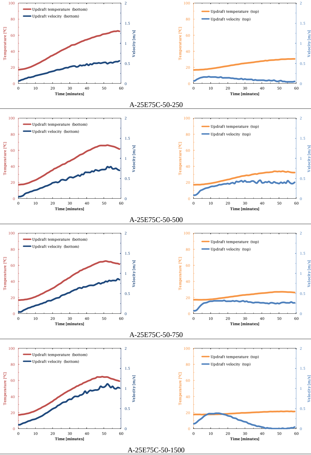
Fig. 5.7 Experimental results for the 1 st measurement group of collector type A.
