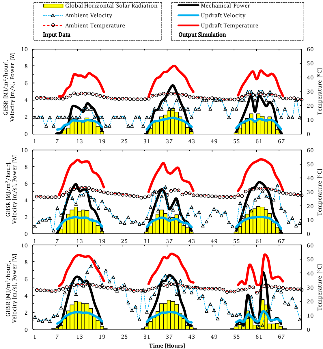
Fig. 7.5 Calculated daily mean mechanical power, updraft velocity, and updraft temperature for a 1:20 scale model Manzanares SUPG.
