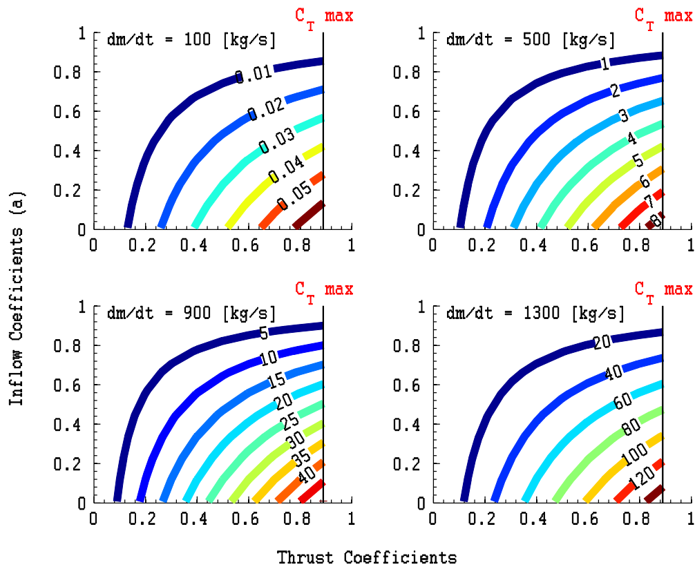
Fig. 3.14 Graphical solution of Eq. (3.49) which shows the effects of inflow coefficients and thrust coefficients to the power production by a wind turbine.
