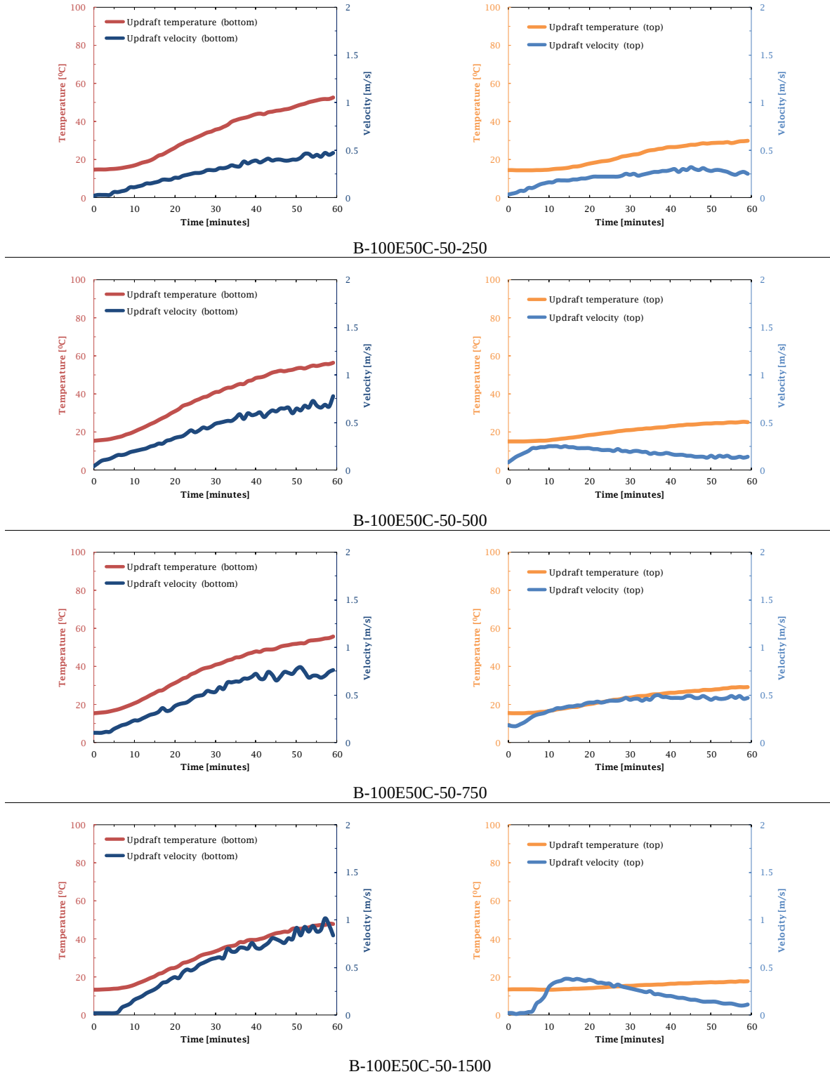
Fig. 5.22 Experimental results for the 7 th measurement group of collector type B.
