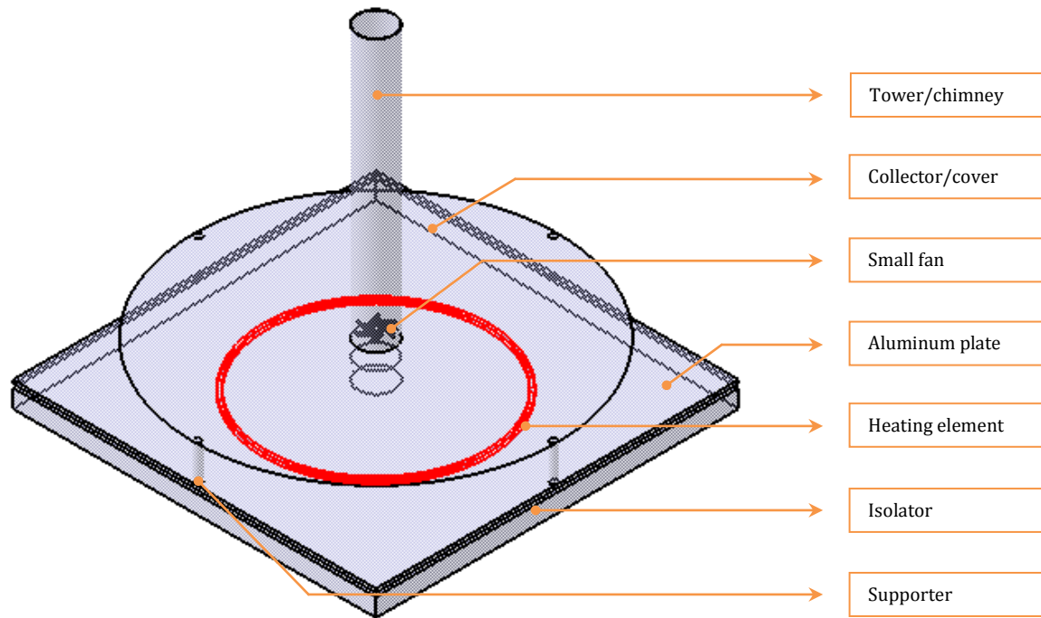
(a) Perspective view of collector type B setup
