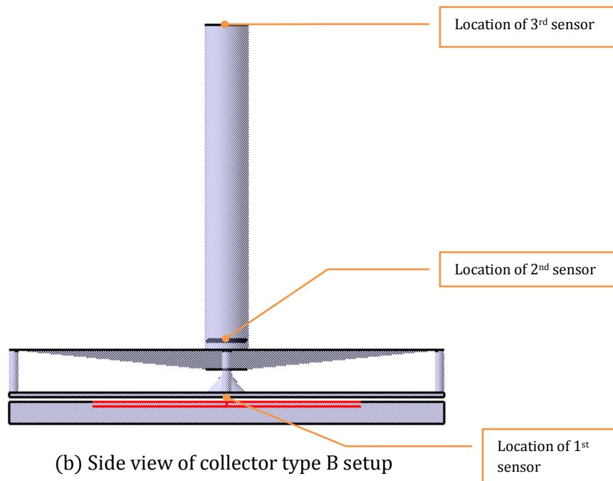
Fig. 5.6 Combination of collector type B, tower, and heating system forming a lab-scale solar updraft power generator.
