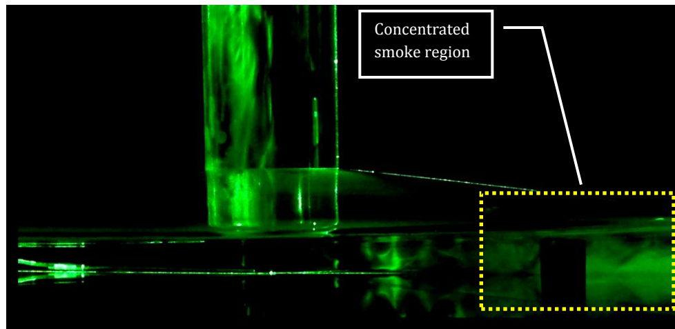
(a) Collector type A
