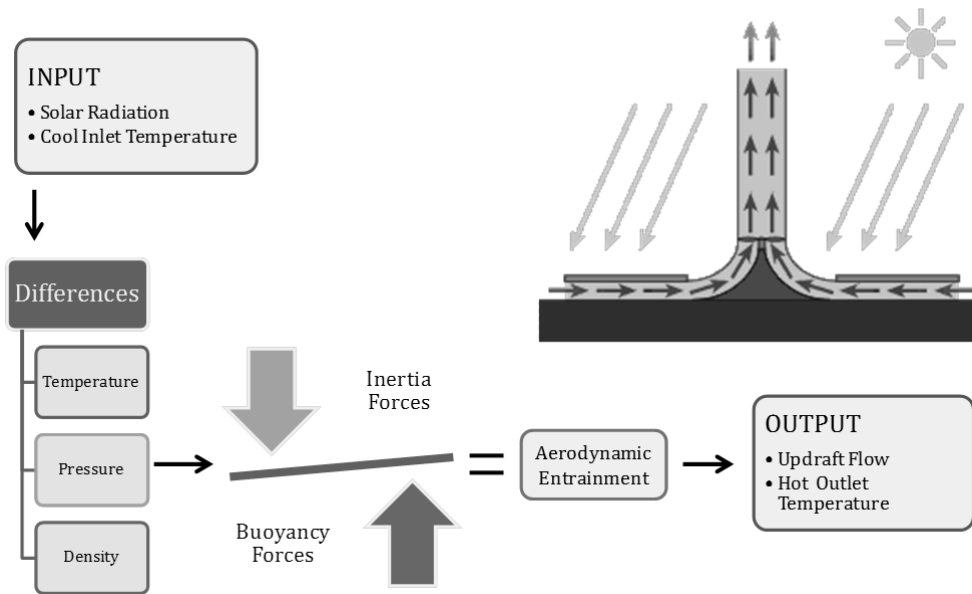
Fig. 2.1 A diagram displaying how a solar updraft power generator works and highlighting the transformation of solar radiation as input to the updraft flow as output. Picture from: http://mtholyoke.edu
