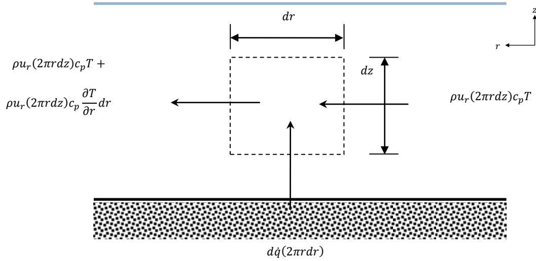
Fig. 3.6 Sketch for discussion of heat flux through normal surface 2\pi r dz for the airflow heat flux and 2\pi r dr for the radiation heat flux.
