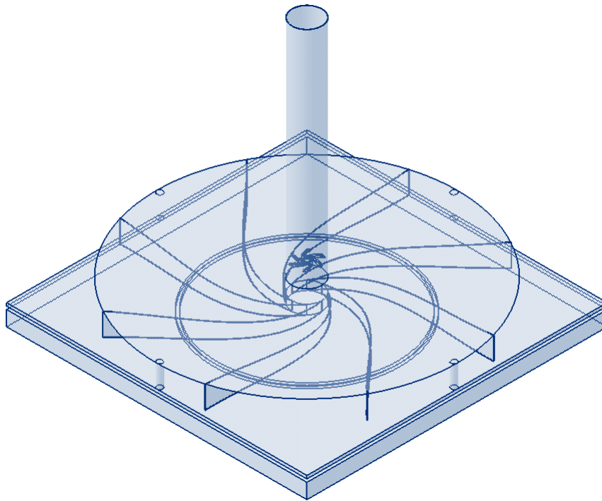
Fig. 8.1 Schematic drawing of optimum design and configuration of solar updraft power generator from the current works to be proposed as outdoor testing prototype.
