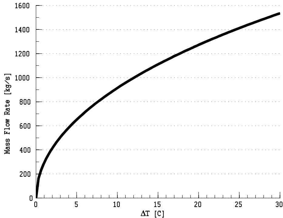
Fig. 3.11 Mass flow rate profile for prescribed airflow density, temperature difference \Delta T = (T_a - T_{a\infty}) , and geometry of solar tower.
