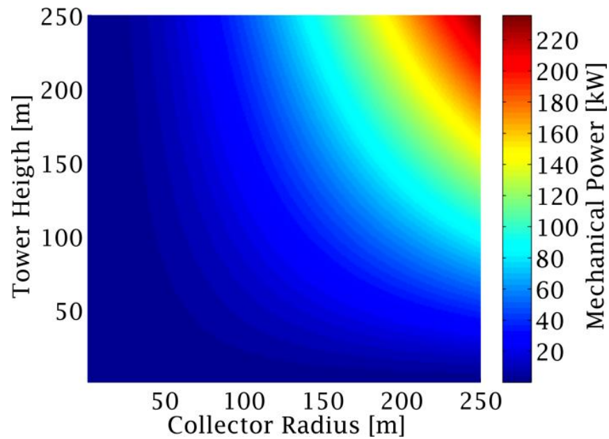
(a) Geometrical effect to the mechanical power
