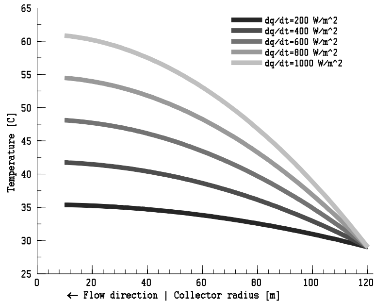
Fig. 3.7 Temperature profile of the airflow from Eq. (3.16). The results have been computed for selected value of radiation heat flux and prescribed mass flow rate.
