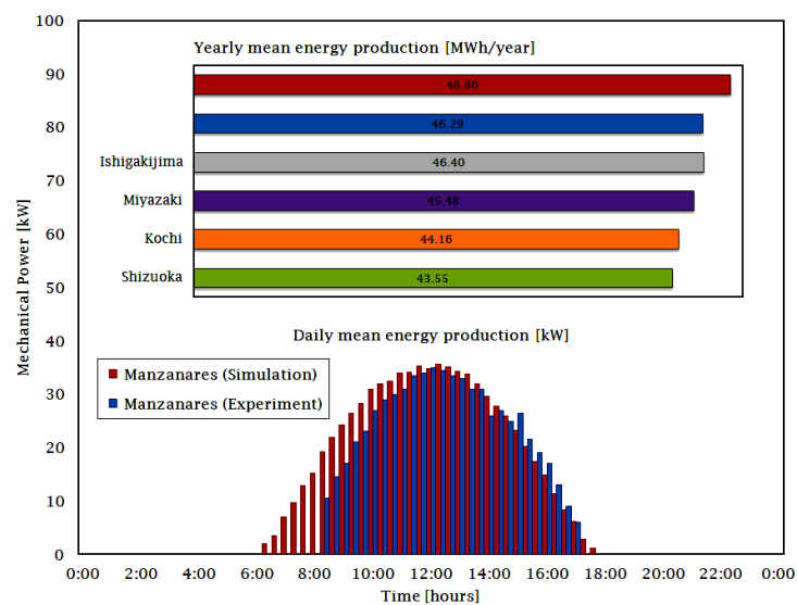
Fig. 7.3 Calculated yearly mean energy production In Japan and comparison of daily mechanical power between simulation and experiment.
