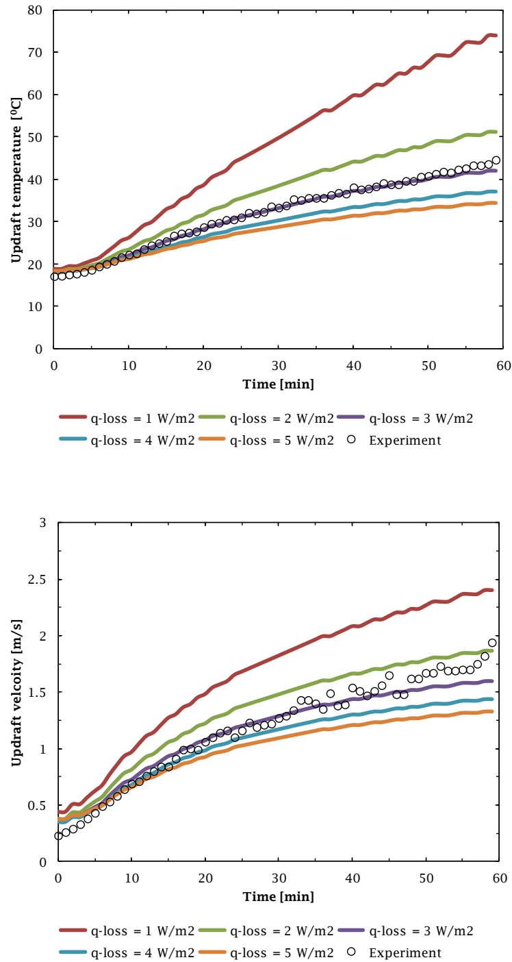
Fig. 4.14 Comparison between simulated updraft temperature and updraft velocity with the experimental results of a lab-scale SUPG.
