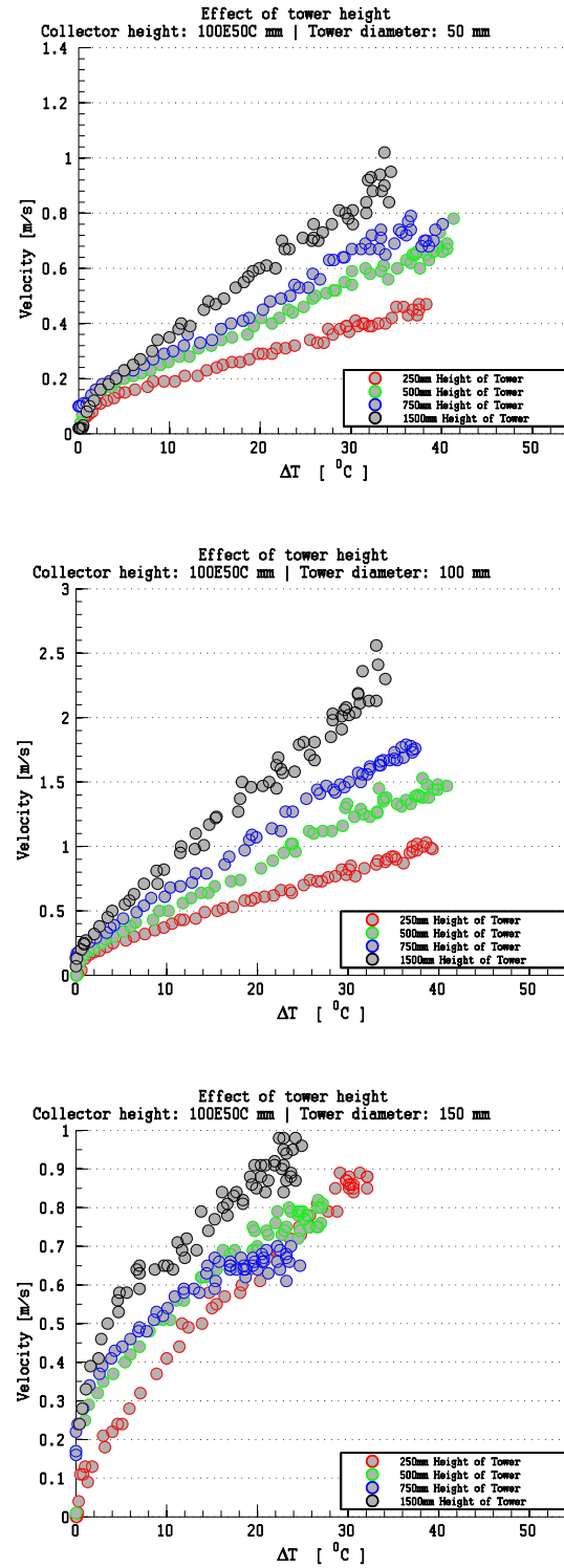
Fig. 6.6 Effects of tower height to the updraft velocity in collector type B.
