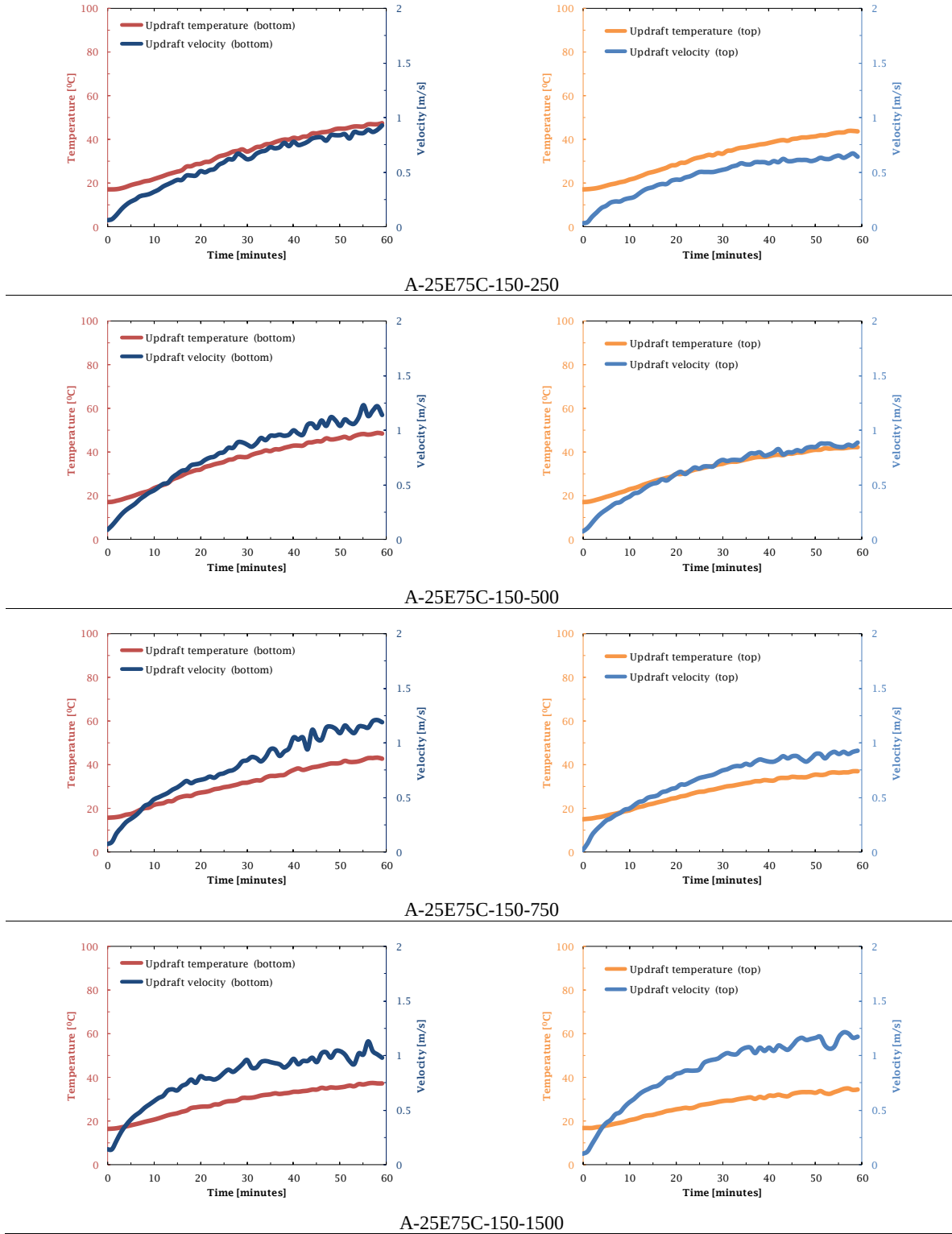
Fig. 5.9 Experimental results for the 3 rd measurement group of collector type A.
