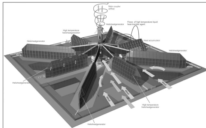
(b) Design of an artificial tornado power generator [67]
