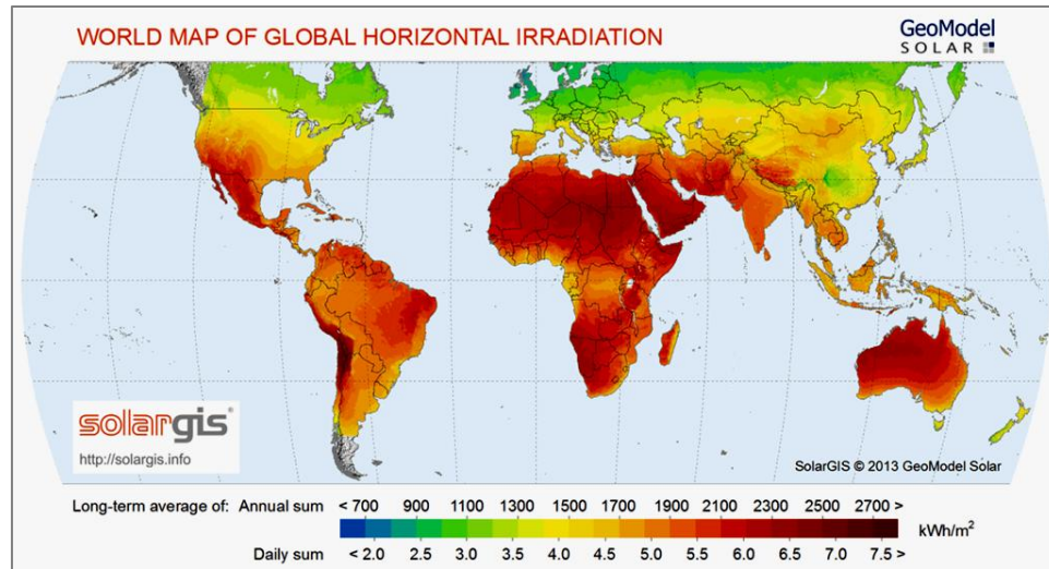
Fig. 1.3 The world map of global horizontal solar radiation. The source of solar radiation data represented on the maps is from SolarGIS database which is provided by SolarGIS © 2013 GeoModel Solar and can be accessed in http://solargis.info .
