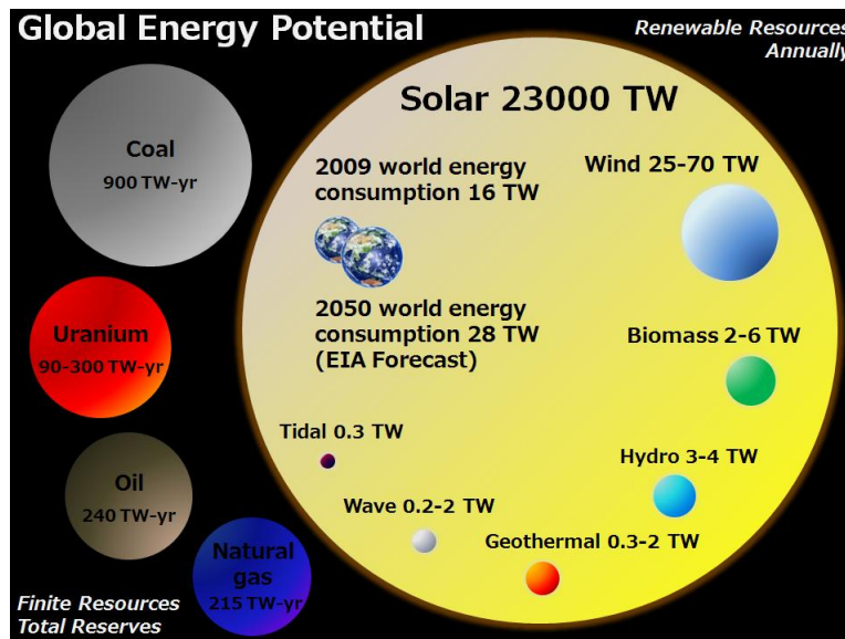
Fig. 1.2 The global energy potential showing the total reserves of finite resources and the yearly reserves of renewable resources.
