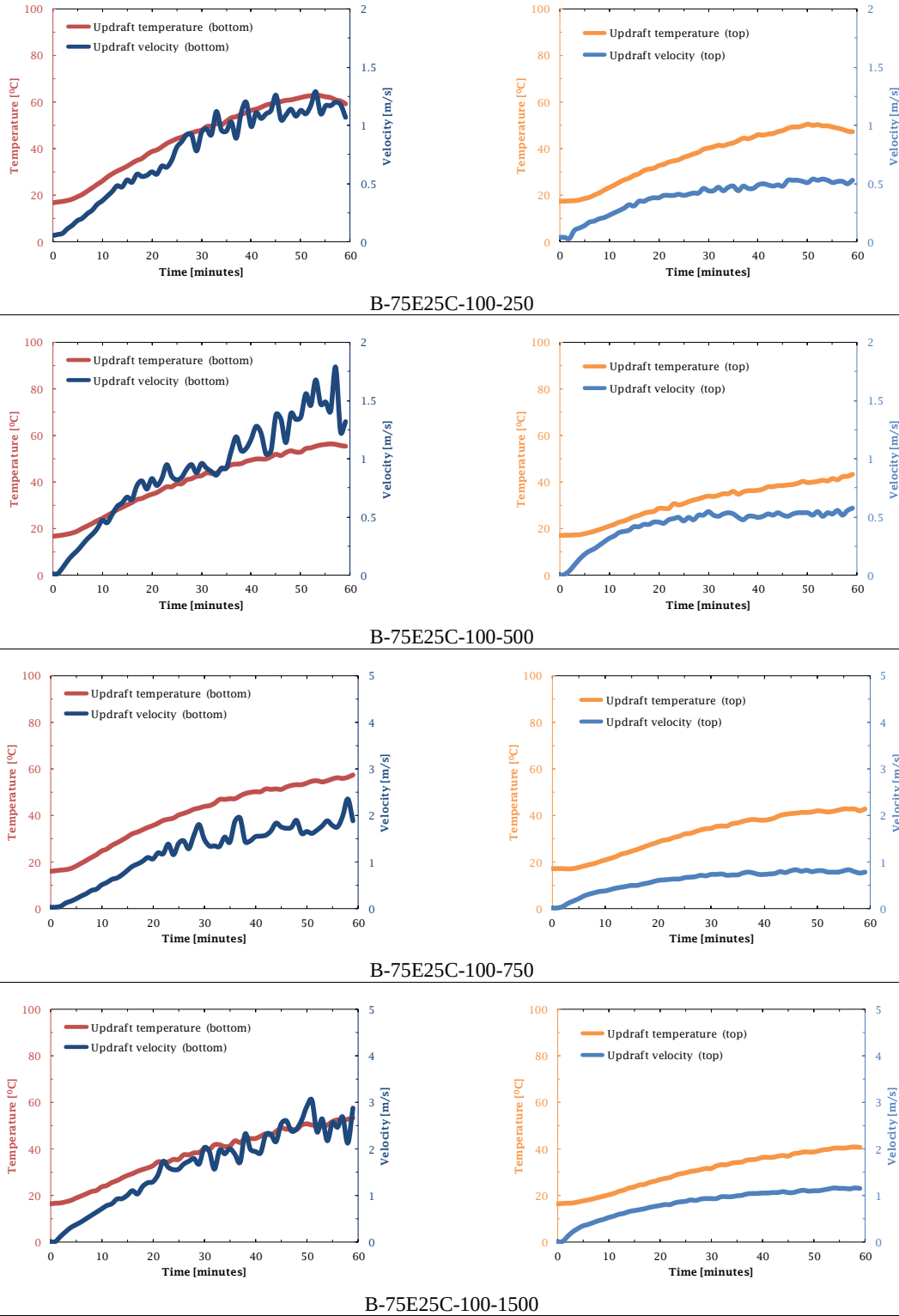
Fig. 5.20 Experimental results for the 5 th measurement group of collector type B.
