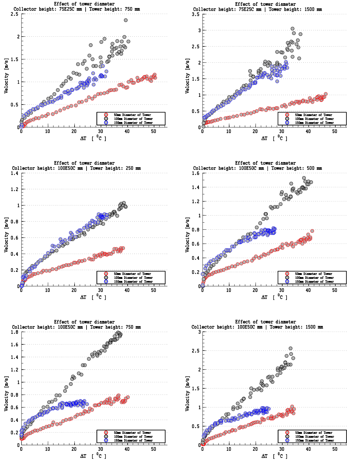
Fig. 6.4 Effects of tower diameter to the updraft velocity in collector type B.
