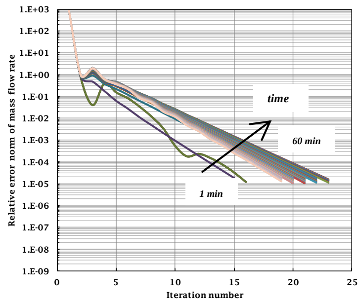
(b) Relative error norm of mass flow rate for each iteration number
