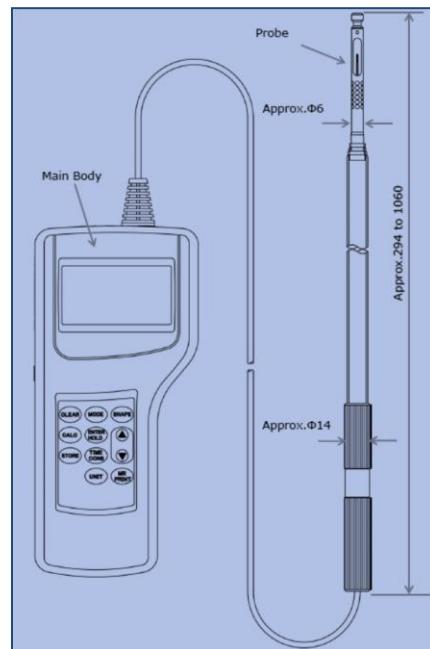
Fig. B.4 A thermo-anemometer sensor used in the experiment to measure the updraft temperature and updraft velocity.
