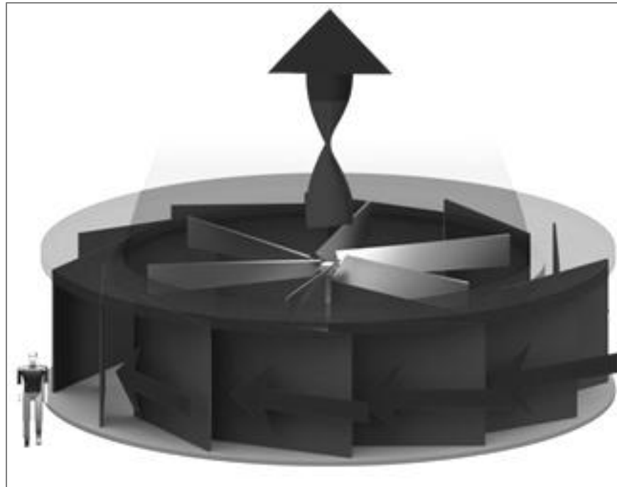
(a) Illustration of a solar vortex power generator [7]
