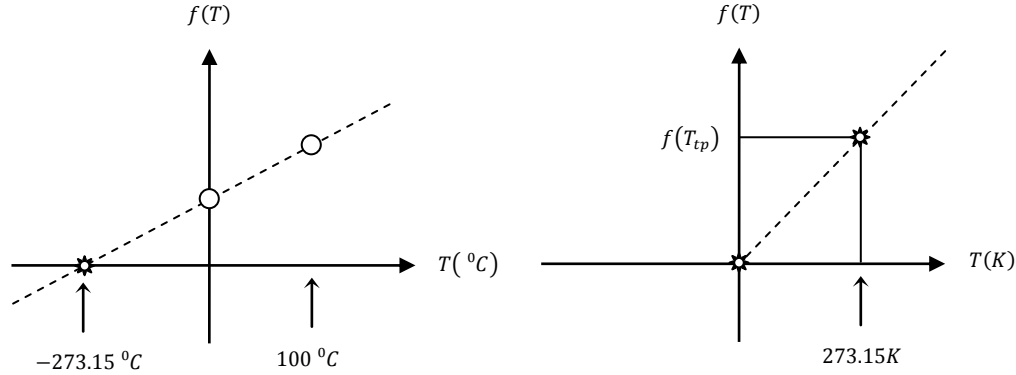
Fig. A3: Ideal gas thermometer scale.
