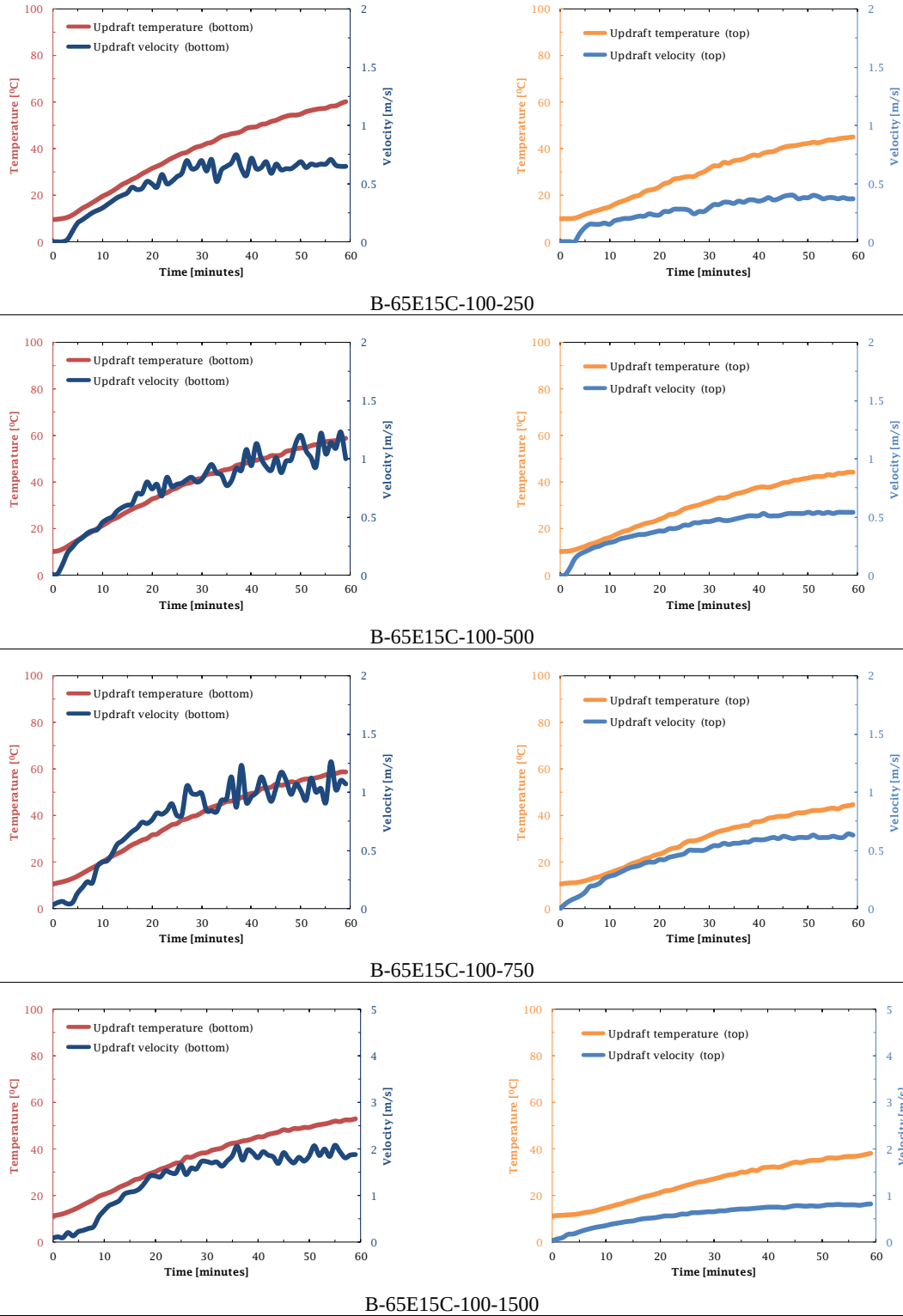
Fig. 5.17 Experimental results for the 2 nd measurement group of collector type B.
