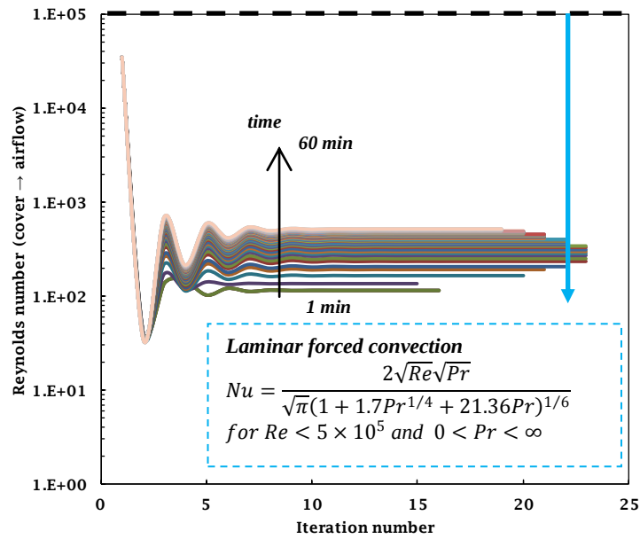
(b) Simulated Reynolds number for heat transfer between airflow and cover
