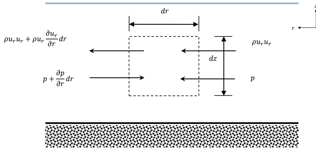
Fig. 3.4 Sketch for discussion of momentum flux through a normal surface 2\pi r dz and the change of velocity and pressure in differential radius dr . The net balance of pressure force is also showed in this figure.
