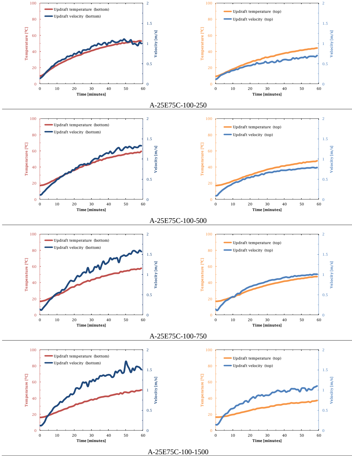
Fig. 5.8 Experimental results for the 2 nd measurement group of collector type A.
