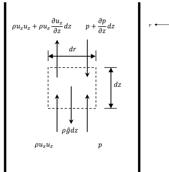
Fig. 3.10 Sketch for discussion of momentum flux for a differential volume of airflow inside the solar tower. The buoyancy force is also showed in this figure.
