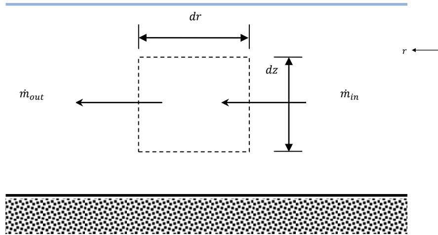
Fig. 3.2 Sketch for discussion of mass flow rate going in \dot{m}_{in} and out \dot{m}_{out} through area A_{col} which is the product of differential height dz and 2\pi r to incorporate the axisymmetric condition.
