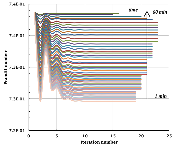
(b) Simulated Prandtl number for heat transfer between airflow and plate
