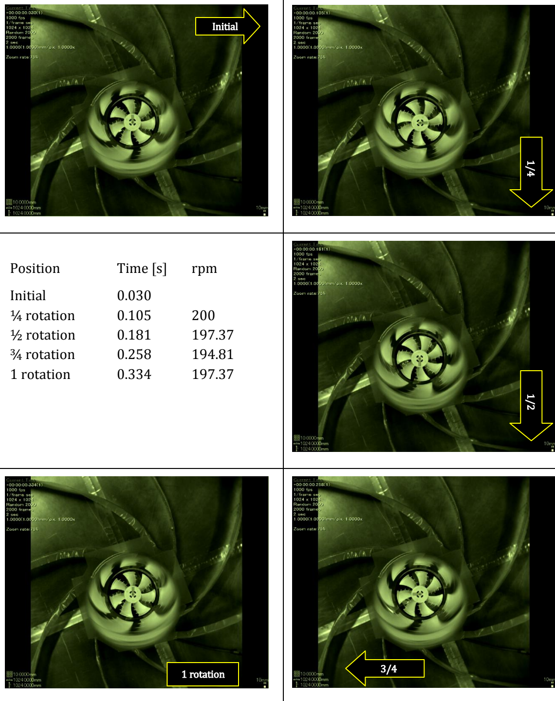
Fig. 5.25 Snapshot picture from high-speed camera showing a complete one rotation of small fan inside the tower.
