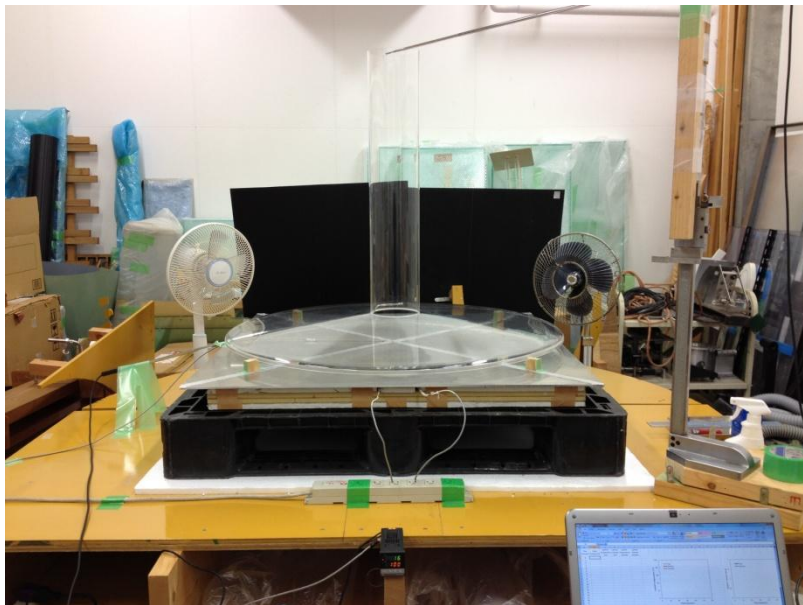
Fig. B.1 Setup of experiment for collector type A.
