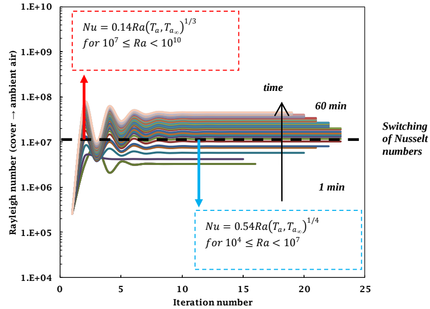
(a) Simulated Rayleigh number for heat transfer between cover and ambient air
