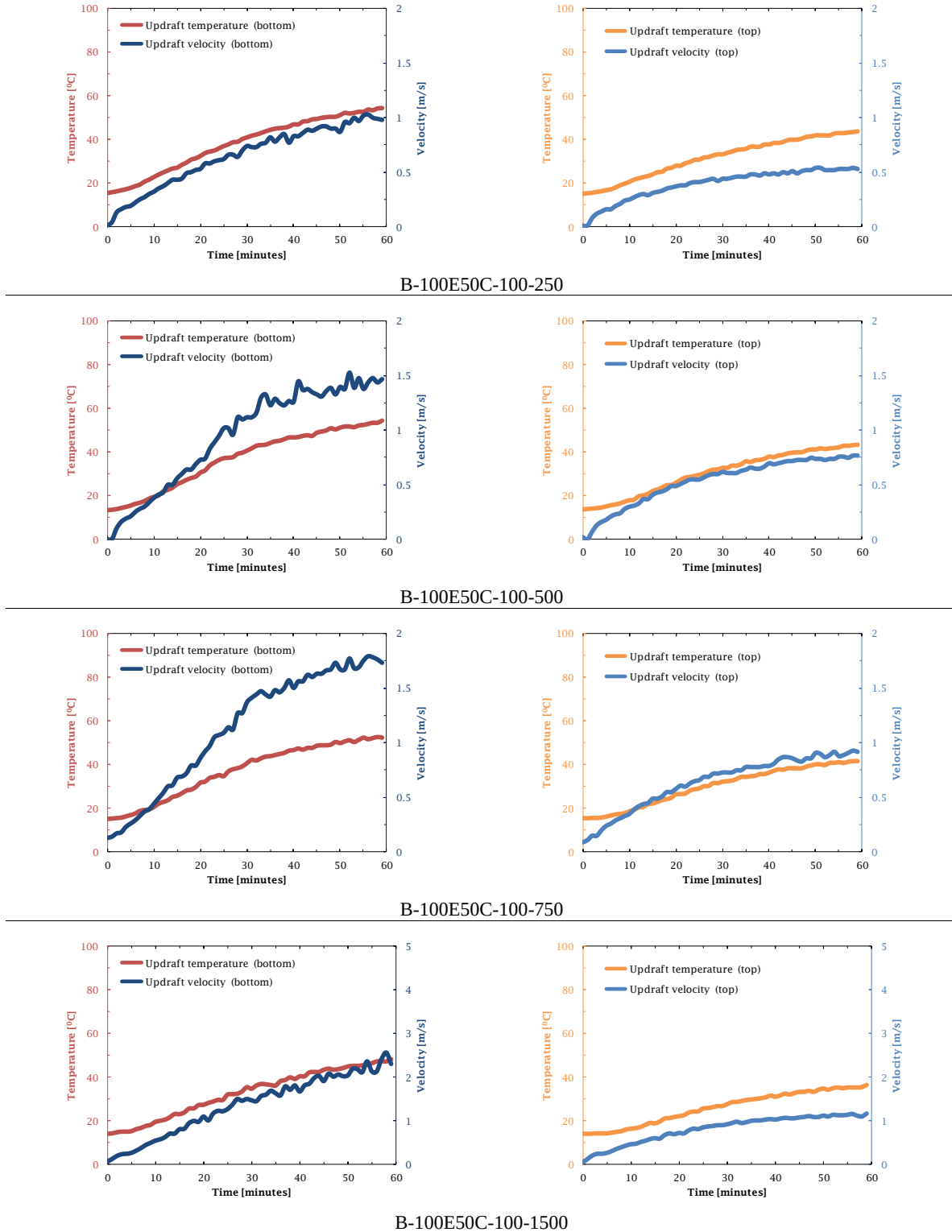
Fig. 5.23 Experimental results for the 8 th measurement group of collector type B.
