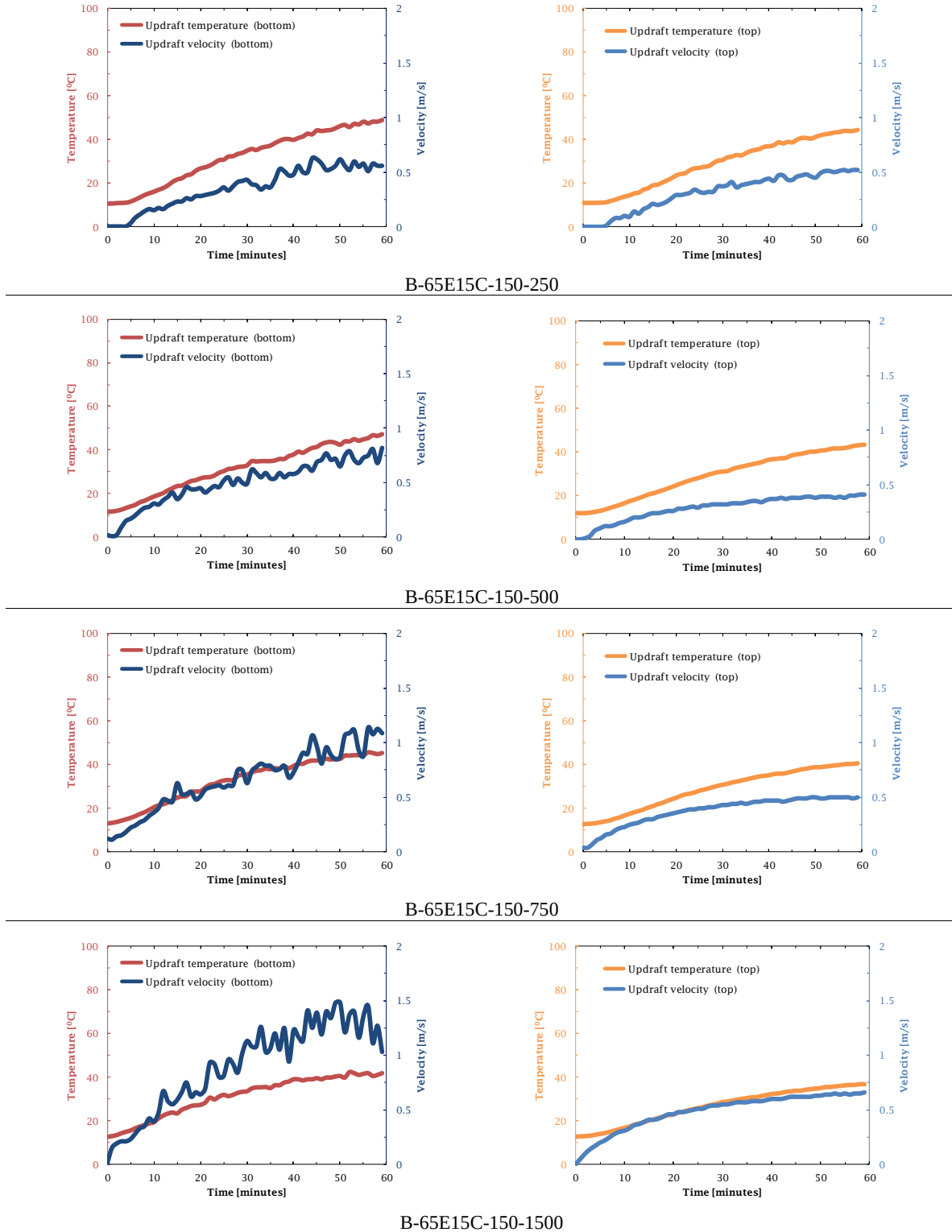
Fig. 5.18 Experimental results for the 3 rd measurement group of collector type B.
