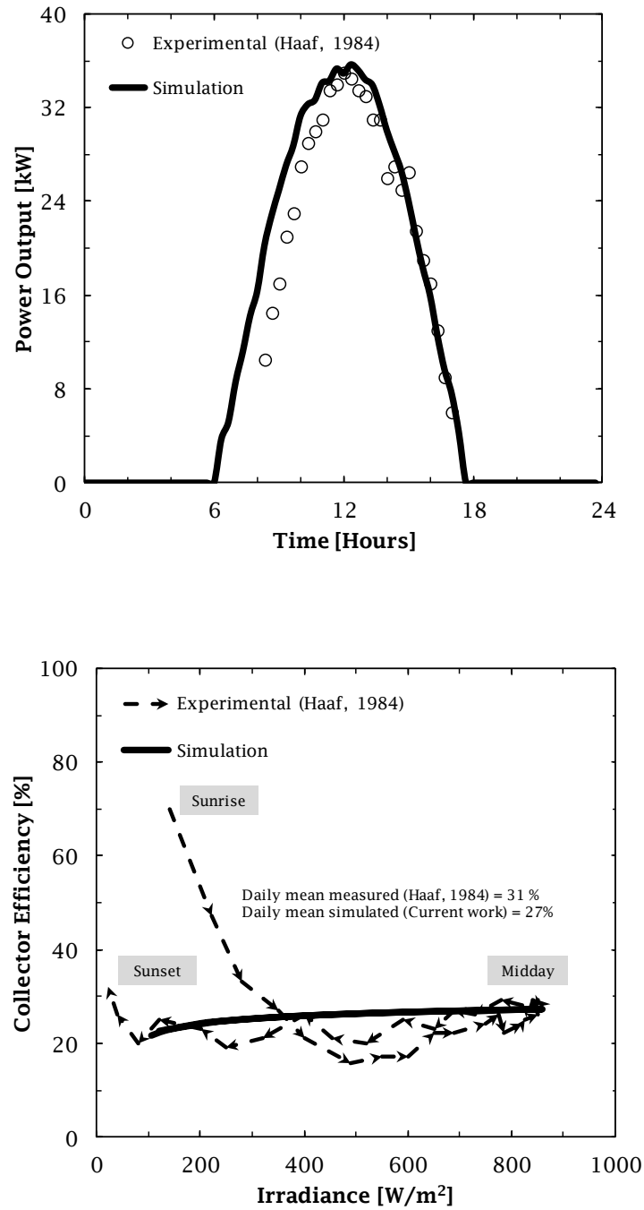
Fig. 4.5 Comparison of mechanical power and efficiency of solar collector between simulation results and the experimental results from the Manzanares experiment.
