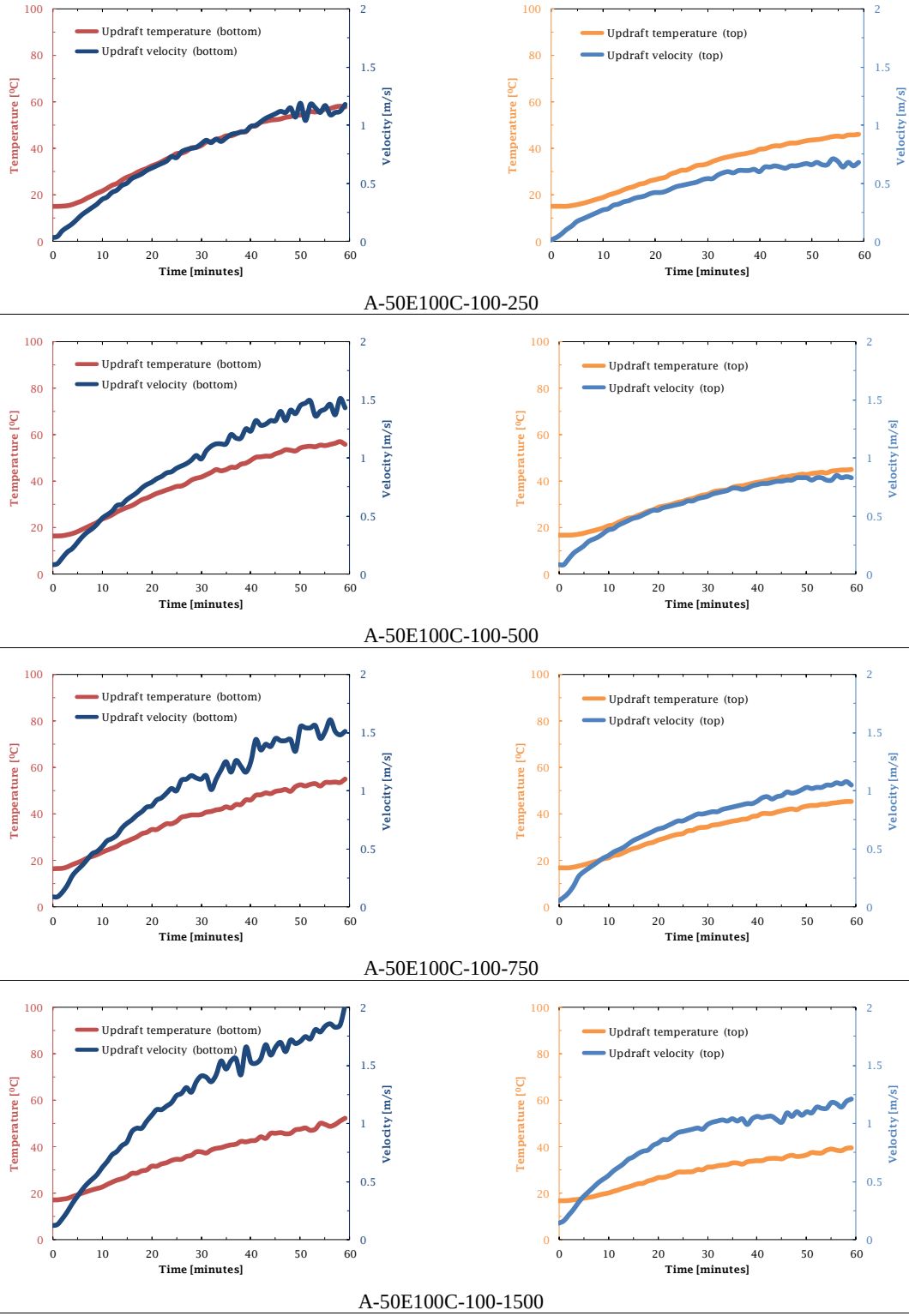
Fig. 5.11 Experimental results for the 5 th measurement group of collector type A.
