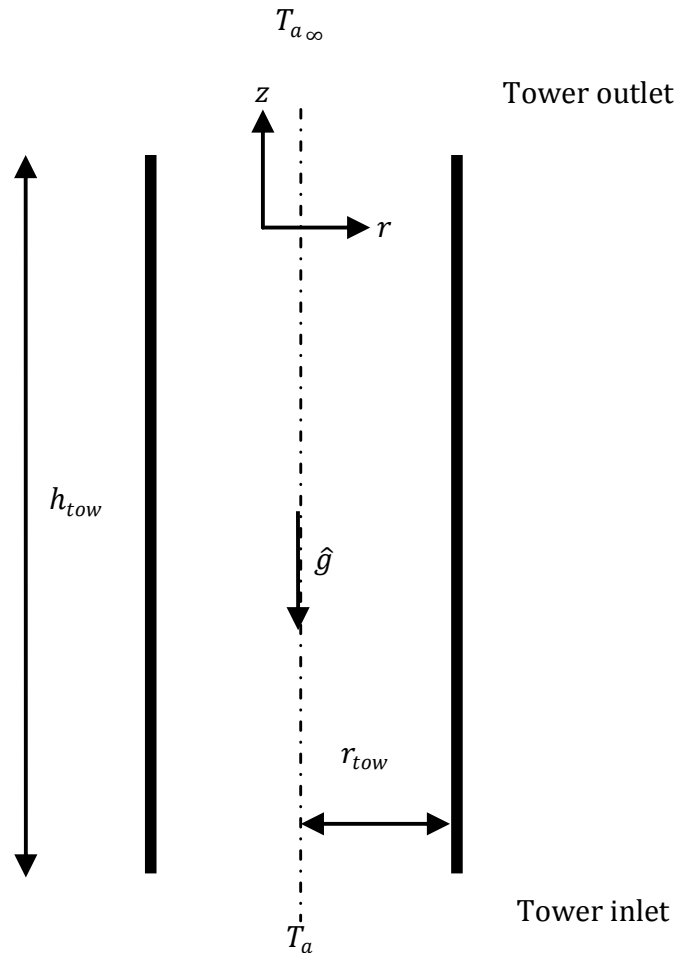
Figure 3.9 Schematic drawing of solar tower.
