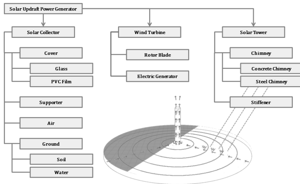
Fig. 2.2 Breakdown of each component of a solar updraft power generator showing that it consist of three main parts: solar collector, solar tower, and wind turbine. Picture from: http://solar-updraft-tower.com
