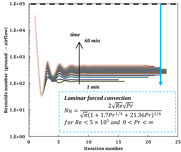
(a) Simulated Reynolds number for heat transfer between airflow and plate
