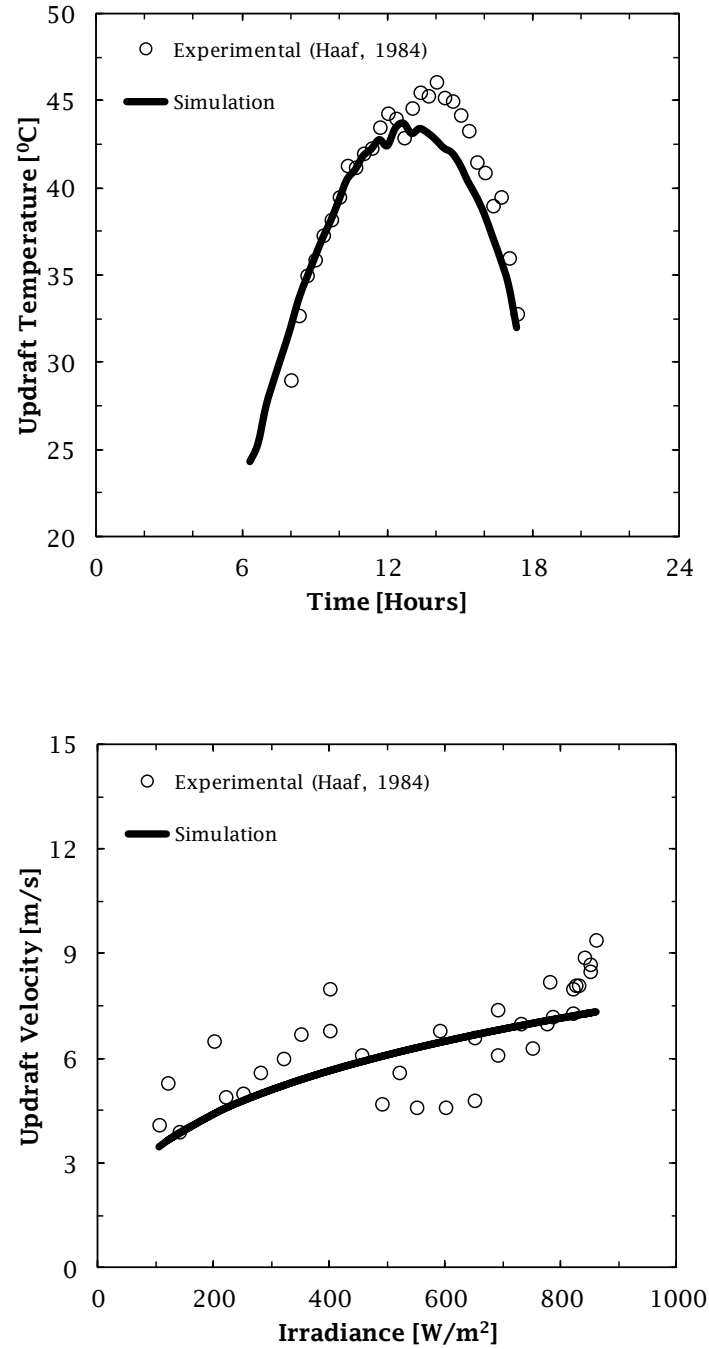
Fig. 4.4 Comparison of updraft temperature and updraft velocity between simulation results and the experimental results from the Manzanares experiment.
