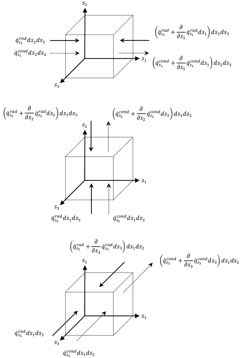
Fig. A4: Energy fluxes for conduction and radiation process associated with a fixed control and moving infinitesimal fluid element.
