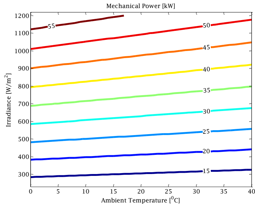
Fig. 4.9 Effect of ambient air temperature to the mechanical power of the Manzanares SUPG.
