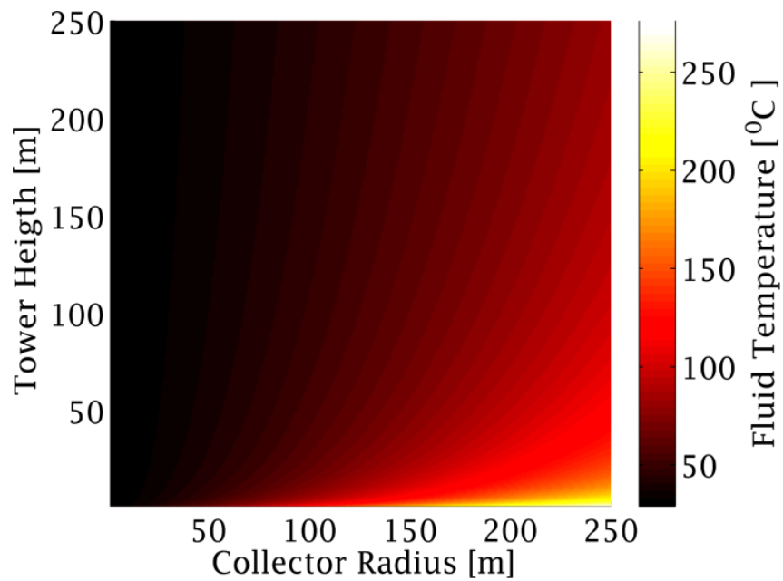
(b) Geometrical effect to the updraft temperature
