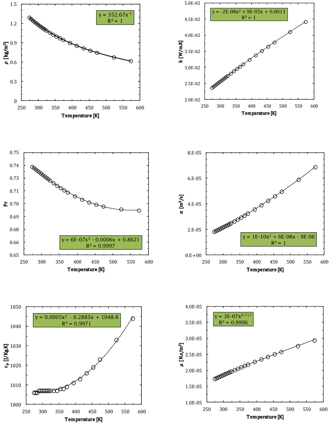
Figure 4.3 Thermal properties used for simulation.
