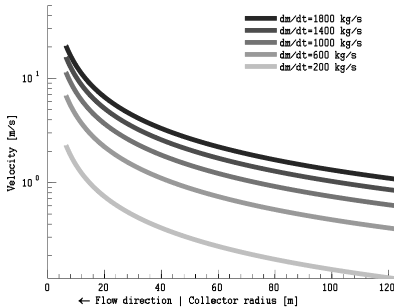
Fig. 3.3 Velocity profile of the airflow inside the solar collector for prescribed mass flow rate. The result is computed for collector radius = 122 m and collector height = 1.85 m with constant density.
