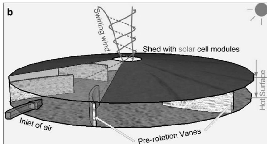
(b) Schematic drawing of a model of solar-induced updraft vortex flows [69]
