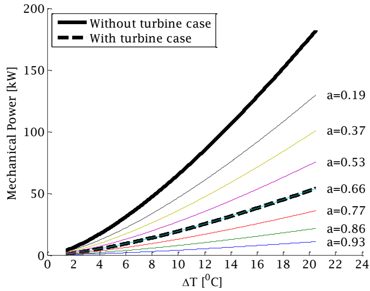
(a) Mechanical power vs temperature difference
