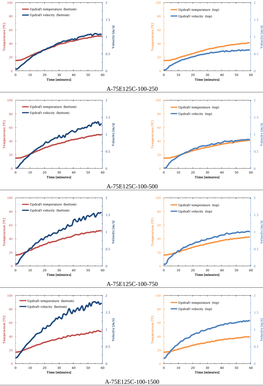
Fig. 5.14 Experimental results for the 8 th measurement group of collector type A.
