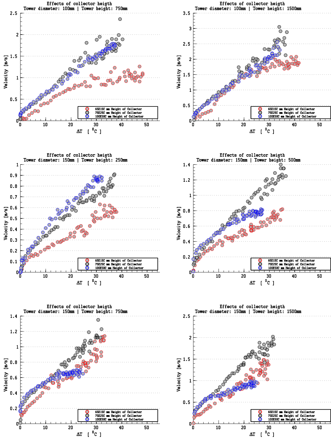
Fig. 6.2 Effects of collector height to the updraft velocity in collector type B.
