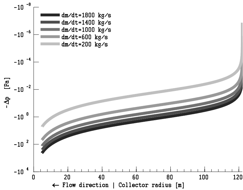
Fig. 3.5 Pressure profile of the airflow fluid inside the solar collector for prescribed mass flow rate. The result is computed for collector radius = 122 m and collector height = 1.85 m with constant density.
