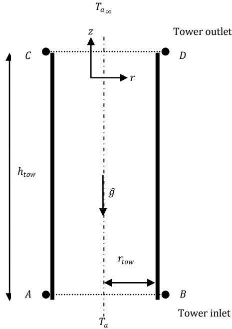
Fig. A5: Sketch for discussion of pressure difference at the inlet and outlet of solar tower.
