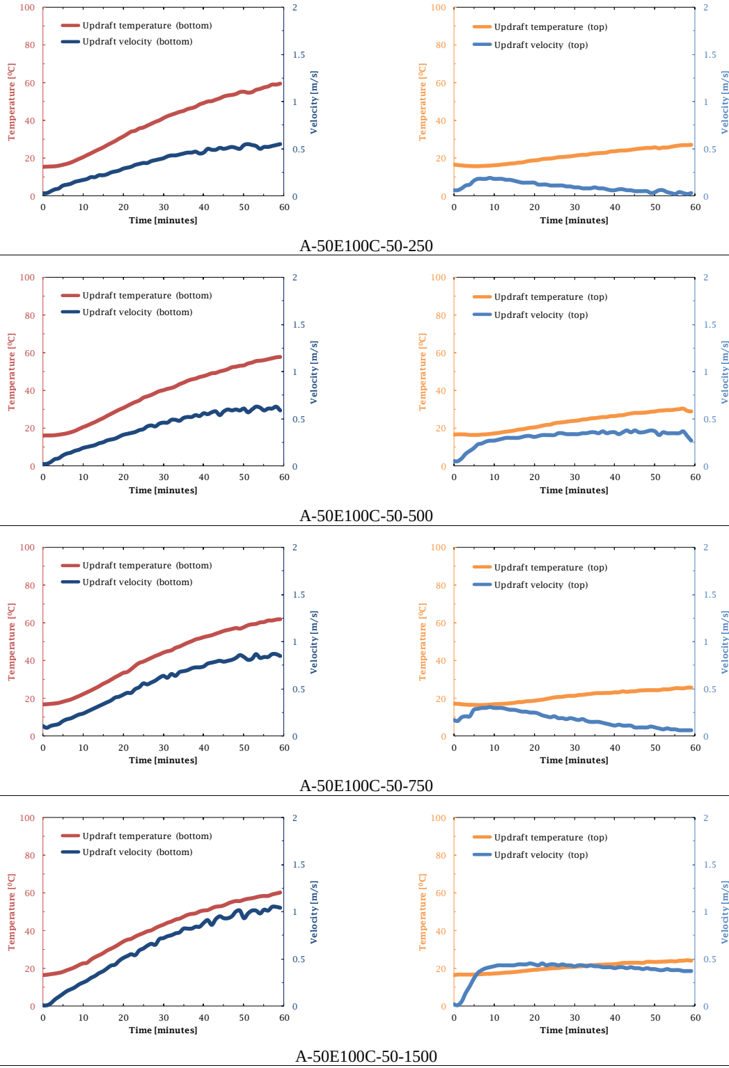
Fig. 5.10 Experimental results for the 4 th measurement group of collector type A.
