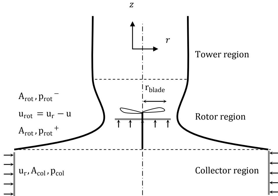
Fig. 3.12 Sketch for discussion of wind turbine model which shows the stream-tube model for energy extraction.
