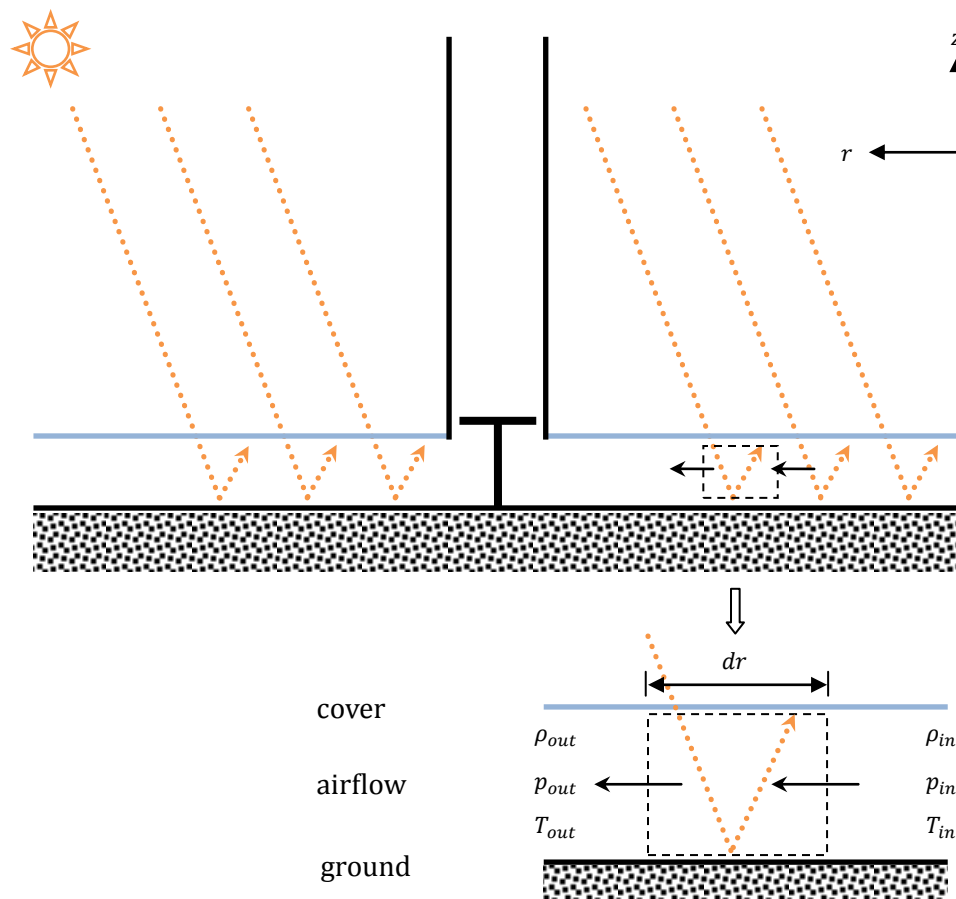
Fig. 3.1 Schematic drawing of a solar updraft power generator focusing on the solar collector where solar radiation heats the air inside.
