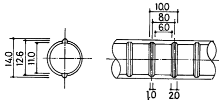
Fig. A-2 Dimensions of Deformed Bar
