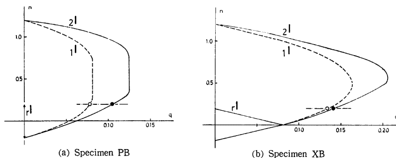
Fig. C-2 Axial Load-Shear Interactions Obtained by Superposition Method
