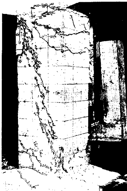
Photo. 4 Damage of Specimen XA
