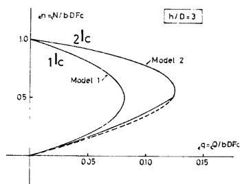
Fig. C-1 Axial Load-Shear Interactions for Plain Concrete
