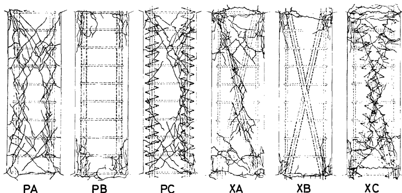
Fig. 4. Crack Observation
