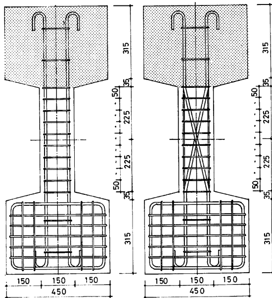
(a) Series P (Conventional Arrangement) (b) Series X (Diagonal Arrangement)
