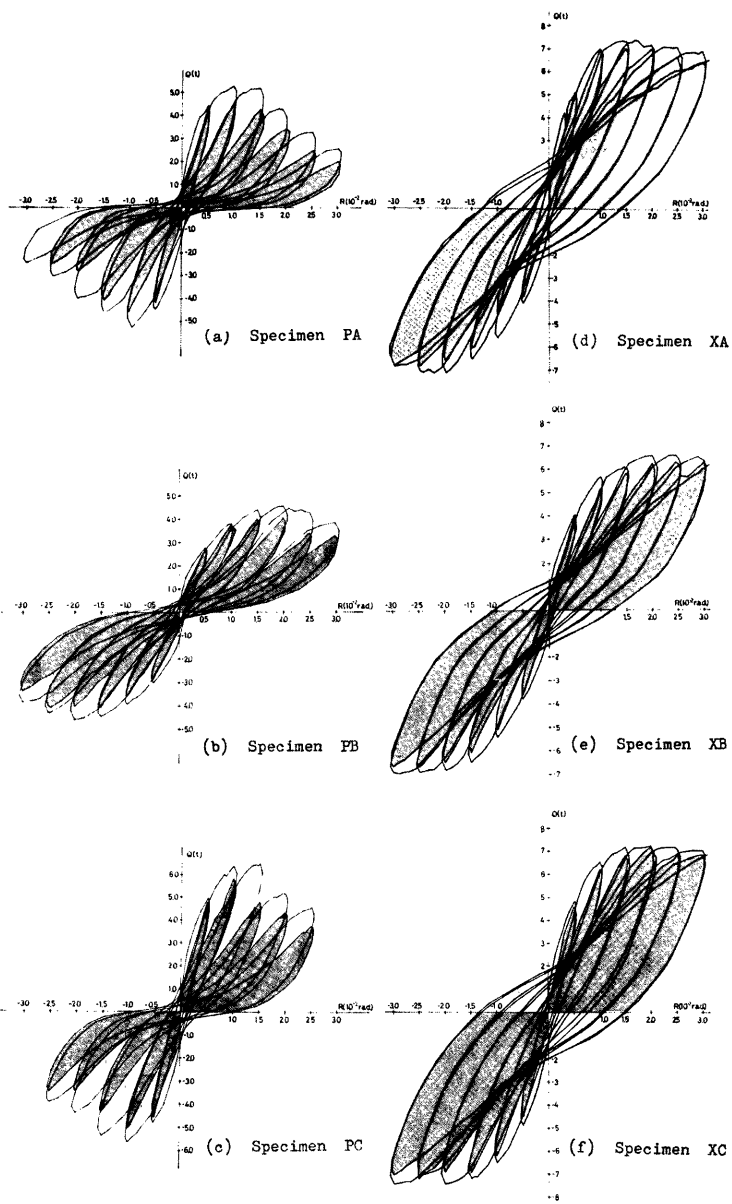
Fig. 6. Load-Deflection Relationships
