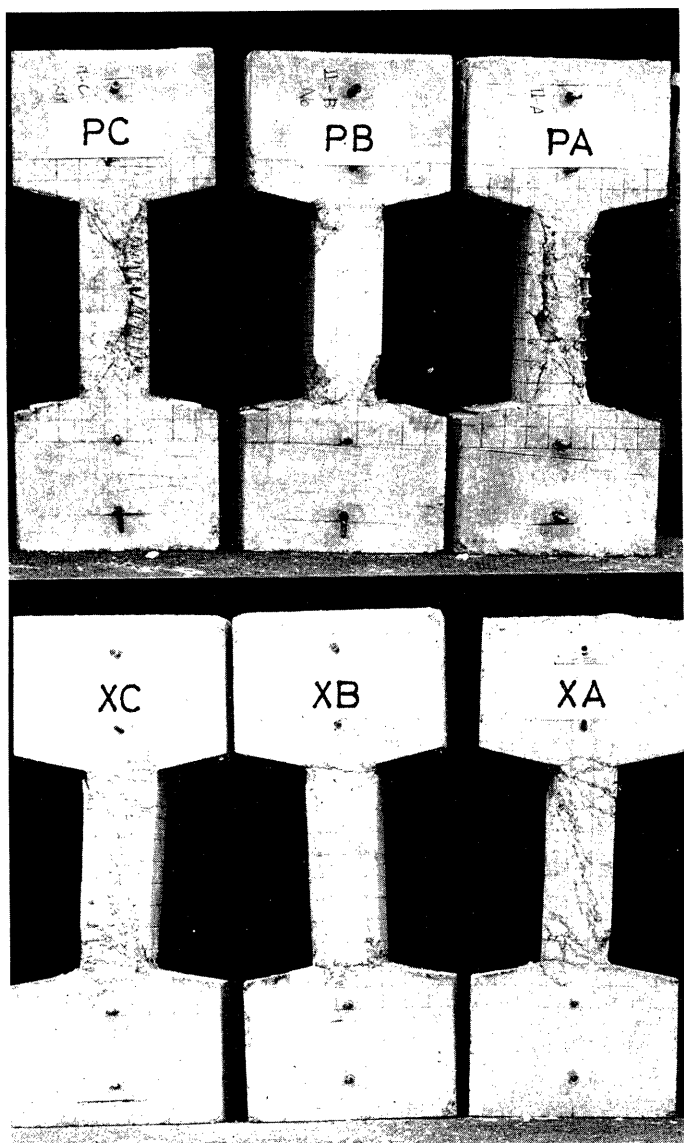
Photo. 3 Test Specimens after Test
