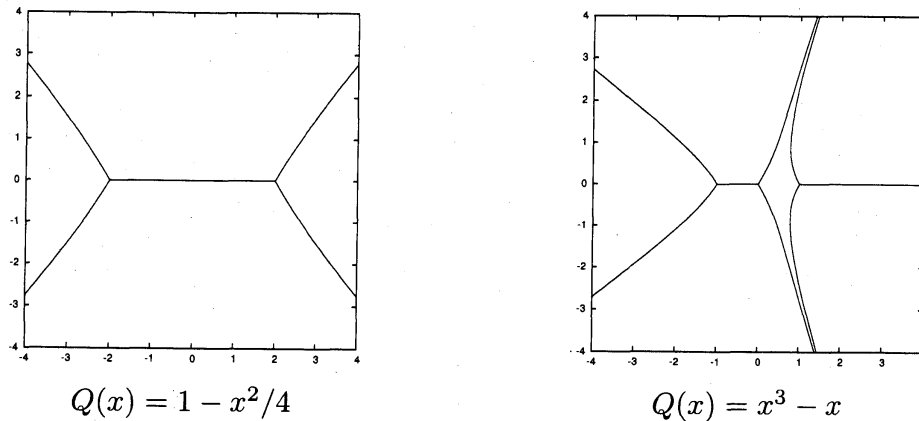
Figure 1. two examples in which Stokes lines connect simple turning points
