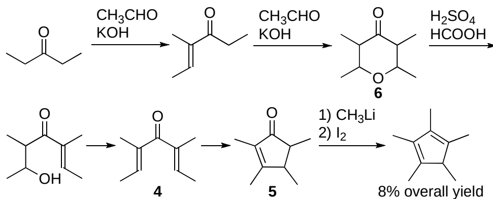
Scheme 4. Burger's Method
