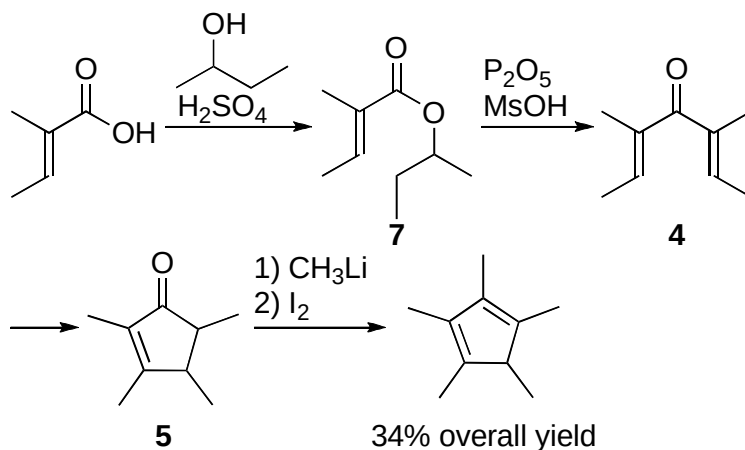
Scheme 5. Whitesides's Method
