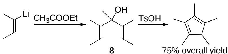
Scheme 6. Bercaw's Method
