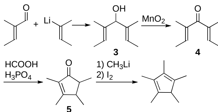
Scheme 3. First Synthesis of Cp*H
