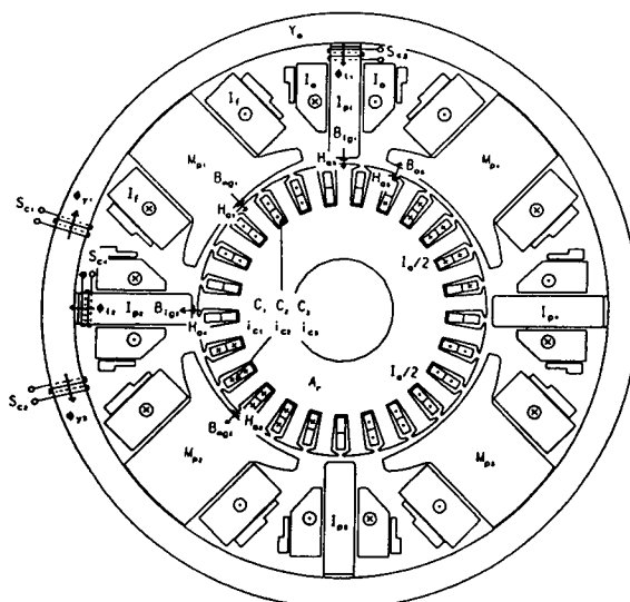
Fig. 1 Gross-sectional view of supplied dc motor.
