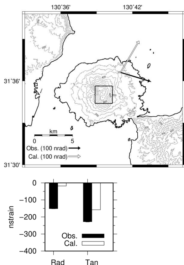
Fig. 6 Comparison of observed and calculated tilt (top) and strain change (bottom) at KMT for the obtained sill model.
