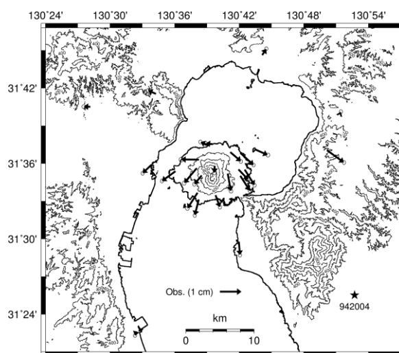
Fig. 7 Horizontal displacement relative to GNSS Earth Observation Network (GEONET) station 942004 (solid star) during the period from October 2011 to March 2012 (Hotta et al., 2016).
