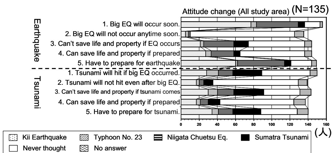
Fig. 3 Indirect disaster experience and attitudinal change (multiple answers, All study areas)
