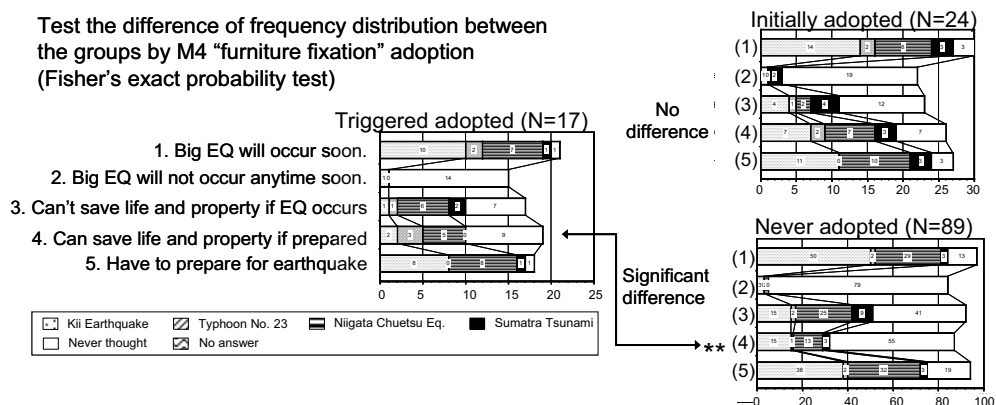
Fig. 6 Attitudinal changes by adoption of furniture fixation
