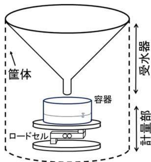
Fig. 5 Structure of water storage rain gauge
