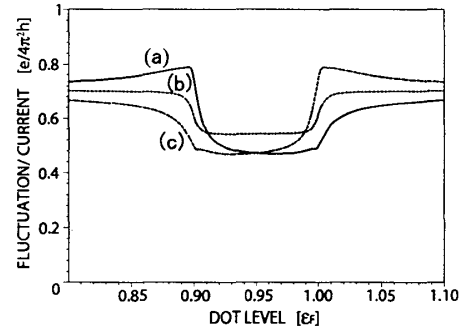
Fig.2. Relative fluctuation at high bias voltage V ( eV/\epsilon_F = 0.1 ) (a) \varphi = \pi , (b) \varphi = \pi/2 , (c) \varphi = 0
