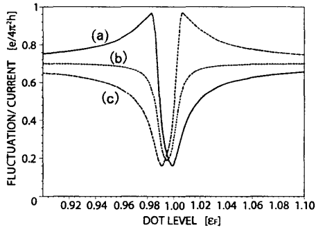
Fig.1. Relative fluctuation at low bias voltage V ( eV/\epsilon_F = 0.01 . \epsilon_F : Fermi energy at eV = 0 ) (a) magnetic flux \varphi = \pi , (b) \varphi = \pi/2 , (c) \varphi = 0
