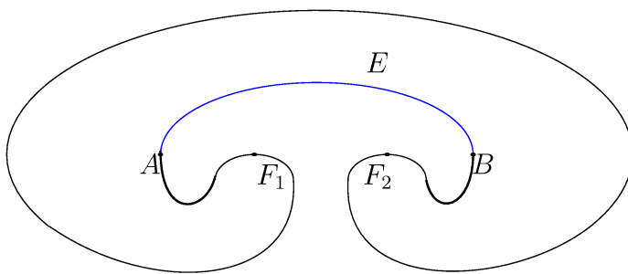
Figure 3. Example of Livshits
