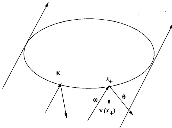
FIGURE 1. Strictly convex obstacle
