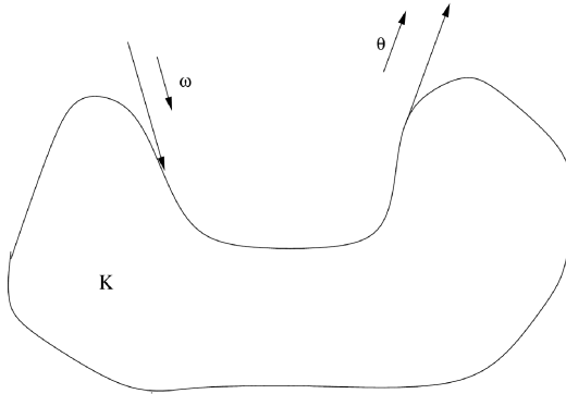
FIGURE 2. Generalized (\omega, \theta) -ray with gliding segments
