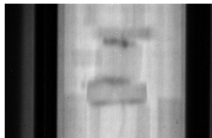
Fig. 2. Typical neutron radiography image of ^7\text{Li-LAGP} after electrolysis for 60 min.
