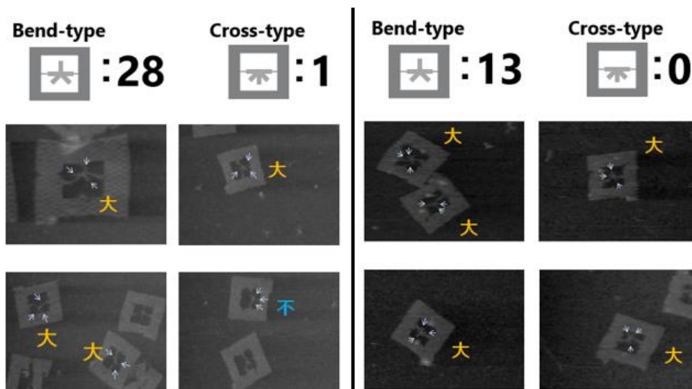
Figure 3. The AFM images of (left) pentapodna#1-4 and (right) pentapodna*1-4 are shown.
