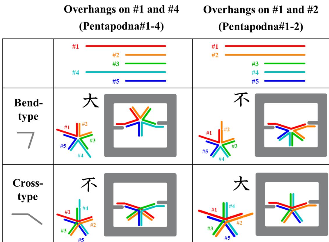
Figure 1. Estimated planar images of ODN orientation in DNA frame. The estimated planar images of pentapodna#1-4 and pentapodna#1-2 were drawn with the assumption that the ODNs are in the bend-type conformation (top) or in the cross-type conformation (bottom). Each ODN is marked with a different color: ODN#1, red; ODN#2, orange; ODN#3, green; ODN#4, cyan; and ODN#5, blue. The grey rectangles are the DNA origami frames.
