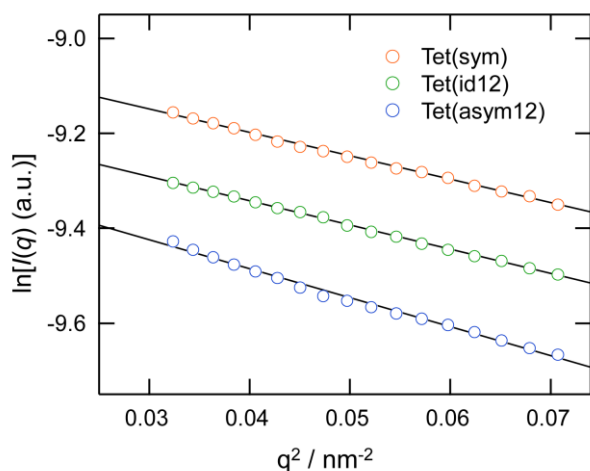
Figure 13. Guinier plots (i.e., \ln(I(q)/c versus q^2 ) of Tet(sym), Tet(id12) and Tet(asym12).
