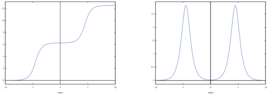
図 9 v = 1/\sqrt{2}, \tau = -6
