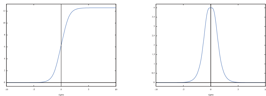
図 10 v = 1/\sqrt{2} , \tau = 0
