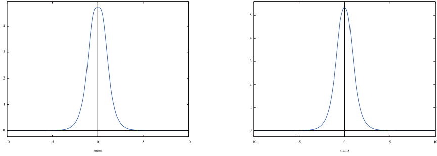
図 14 v = 0.8, \tau = -\tau_0 \simeq -0.38034, \tau = 0
