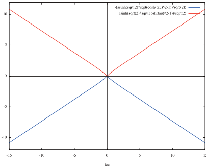
図 8 trajectory v = 1/\sqrt{2}
