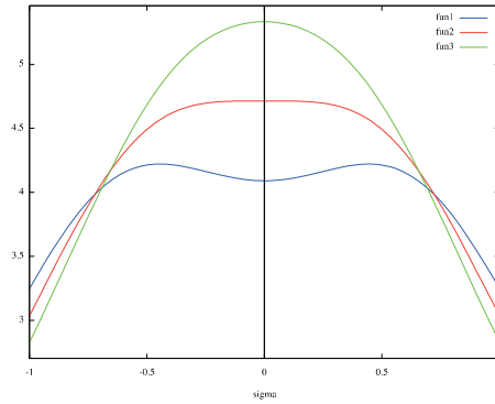
図 15 v = 0.8, \tau = -1.5\tau_0 \tau = -\tau_0 \simeq -0.38034, \tau = 0
