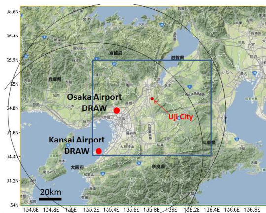
Fig. 7 Locations of the Doppler radars (DRAW) at the Kansai Airport and at the Osaka airport, and their observation areas (circles).
