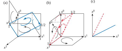
Fig. 1. Faces of primal and dual grids based on Hodge duality (13): (a) primal face, (b) dual face, and (c) the projections on the x^0 - x^1 plane.
