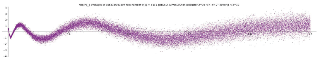
abelian surfaces with generic Sato–Tate group
