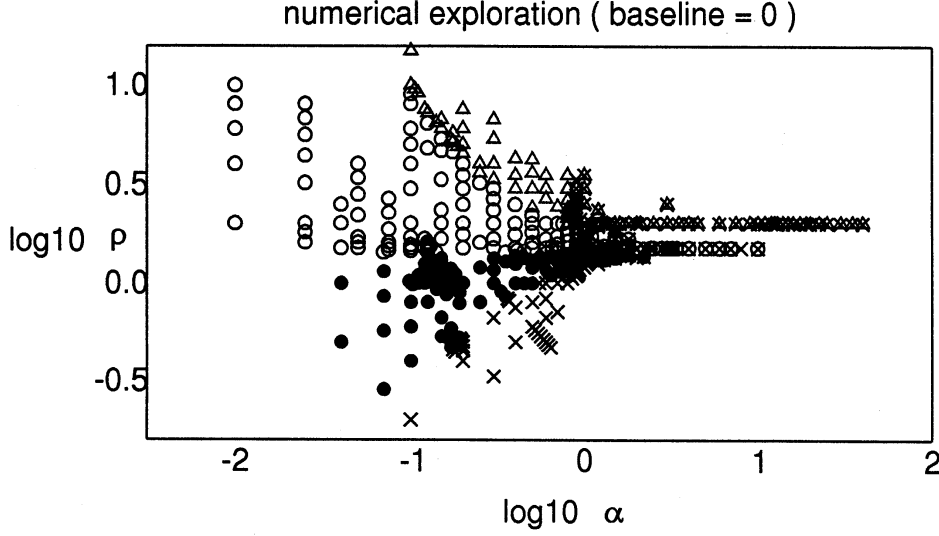
Figure 1: The range of (\alpha, \beta) for numerical exploration of steady pulses: \rho = \beta/\alpha , u_b = 0 . Symbols stand for: \circ and \bullet , positive and negative pulses with monotone tails; and \Delta and \times , positive and negative ones with oscillatory tails, respectively.
