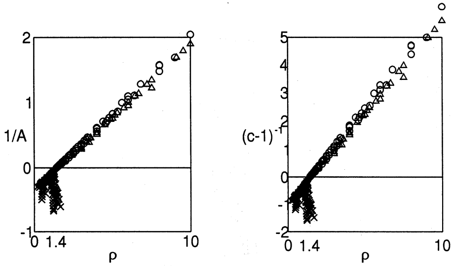
Figure 4: Dependence of A and c on \rho = \beta/\alpha , in the case when \alpha and \beta are not very large.
