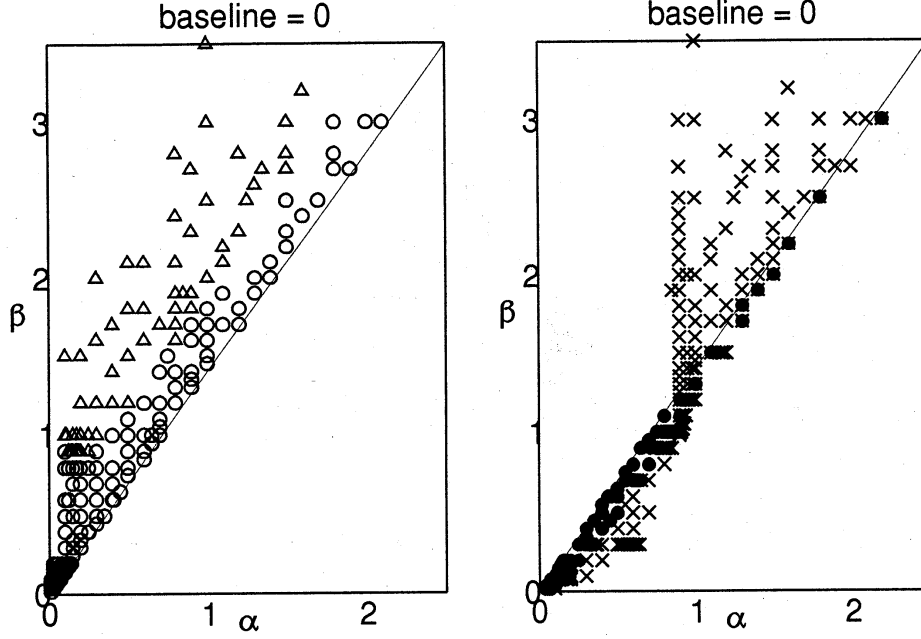
Figure 3: The range of the parameters (\alpha, \beta) for which positive (left figure) or negative (right figure) steady pulses were found ( u_b = 0 ). Symbols are the same as in Fig. 1.
