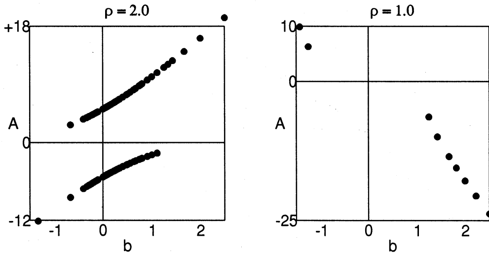
Figure 6: Dependence of the amplitude A on b in the normalized equation (27), for \rho = 2.0 (left figure) and for \rho = 1.0 (right figure).
