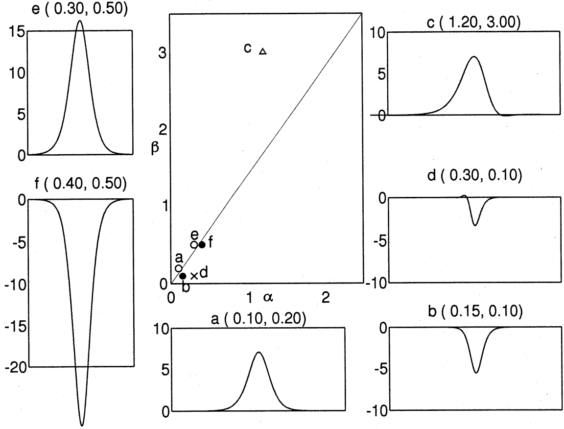
Figure 2: Pulse solutions of the equation (15), numerically obtained for the parameter values indicated in the graph at the center (and for u_b = 0 ). (a),(c),(e) are positive pulses, while (b),(d),(f) are negative. (c) and (d) have an oscillatory tail. The line ( \beta/\alpha = 7/5 ) on the parameter plane is predicted by (22) to divide the territories of the positive and negative pulses. Symbols are the same as in Fig. 1.
