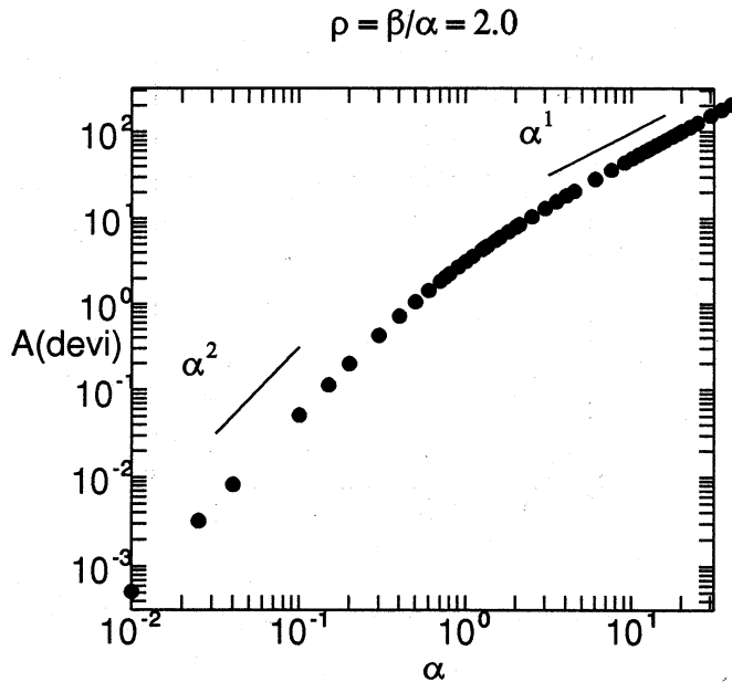
Figure 5: Deviation of A from (22), shown against \alpha in log-log plot; \rho = \beta/\alpha = 2.0 is fixed.
