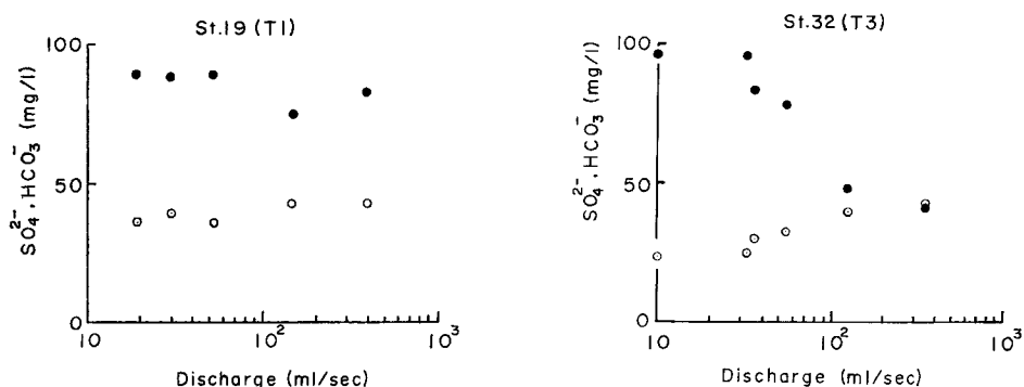
Fig. 6A Plots of HCO 3 - and SO 4 2- contents against discharge of waters in the Kamenose landslide area (●: HCO 3 - and ○: SO 4 2- ).
