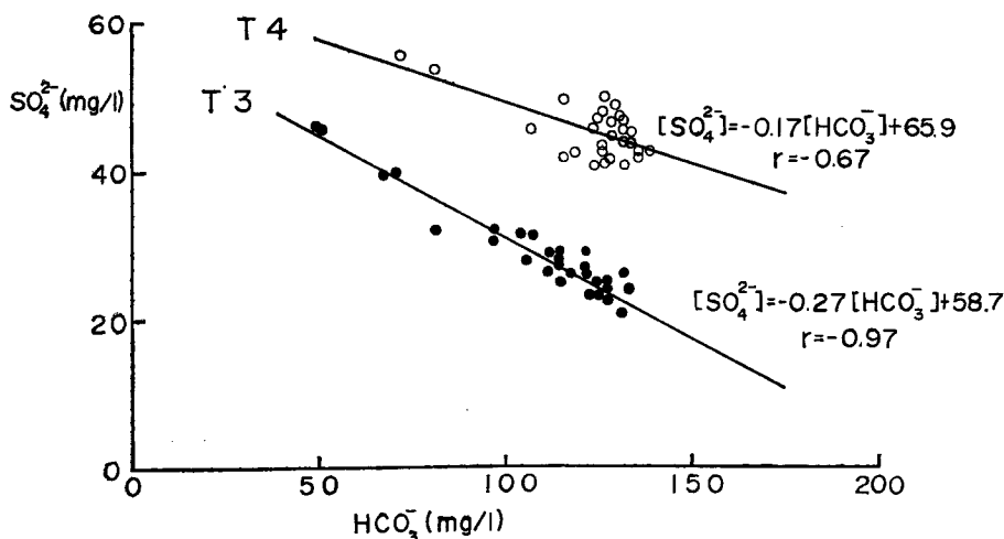
Fig. 3 Plots of \text{SO}_4^{2-} content against \text{HCO}_3^- content of waters in the Kamenose landslide area.
