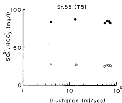
Fig. 6B Plots of HCO 3 - and SO 4 2- contents against discharge of waters in the Kamenose landslide area (●: HCO 3 - and ○: SO 4 2- ).
