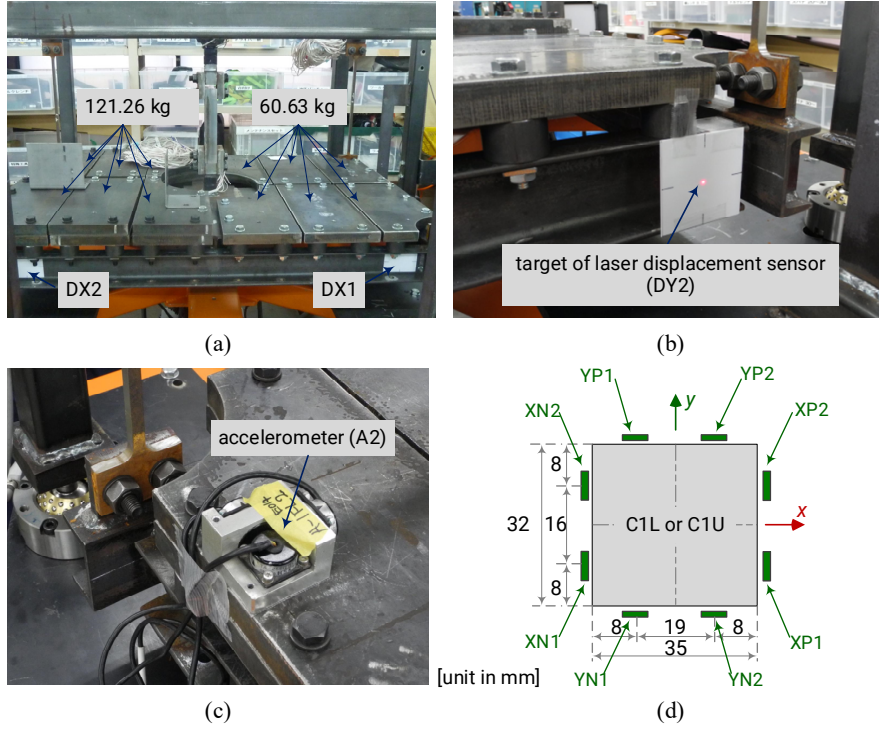
Figure 2: Arrangements of mass and measurement devices. (a) Arrangement of steel plate masses on the floor; (b) A target of a laser displacement sensor; (c) An accelerometer installed; (d) Layout and label of strain gauges at C1L and C1U columns.
