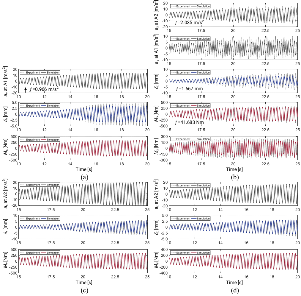
Figure 17: Comparison of test data and simulated values of the responses of interest from the test used for identification and from the verification tests using the best parameter set found from case 5 (i.e., No. 9). Arrow indicates the response used for formulating f_2 . (a) Test No. 9; (b) Test No. 3; (b) Test No. 4; (d) Test No. 10.
