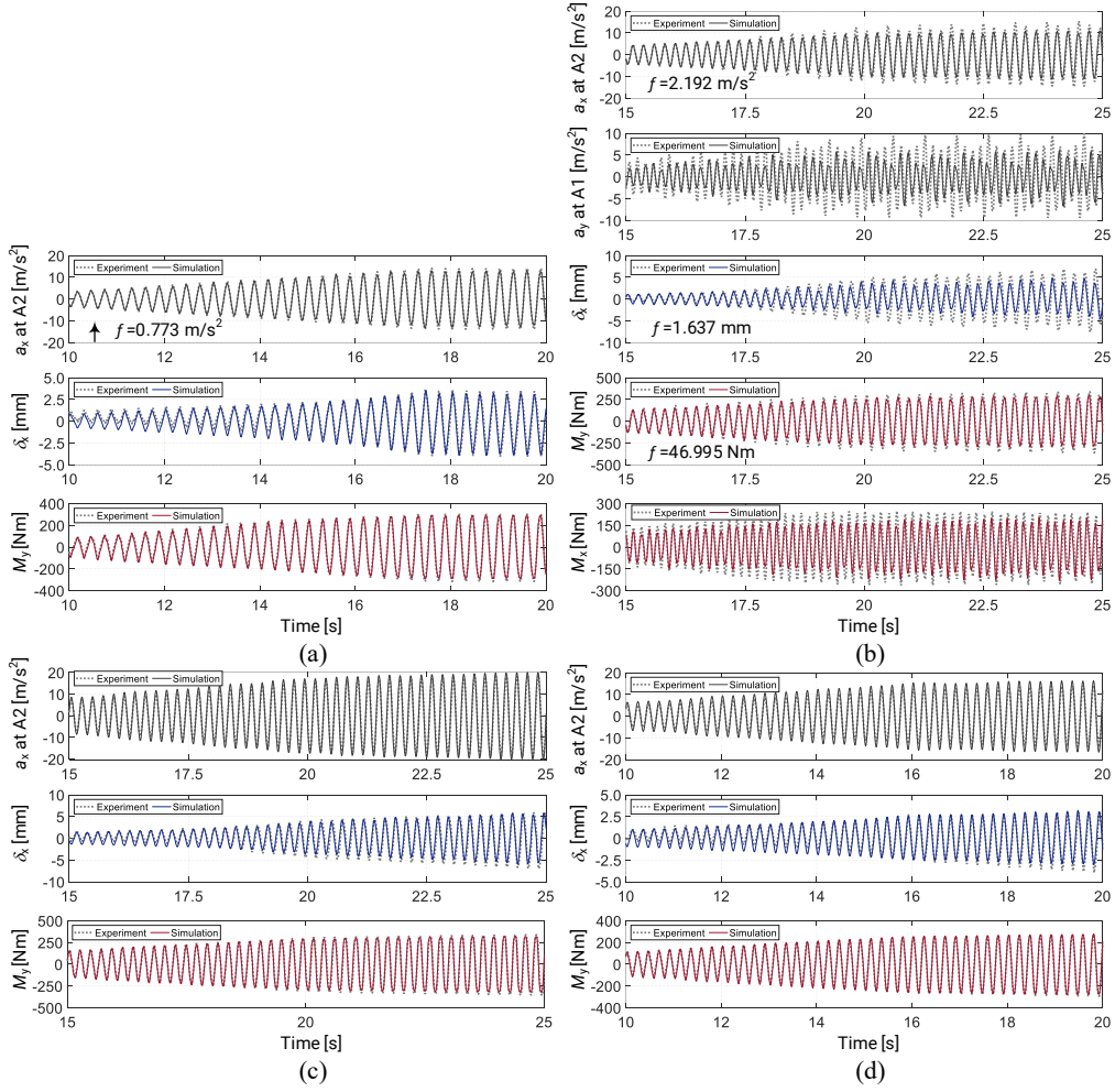
Figure 16: Comparison of test data and simulated values of the responses of interest from the test used for identification and from the verification tests using the best parameter set found from case 4 (i.e., No. 8). Arrow indicates the response used for formulating f_2 . (a) Test No. 8; (b) Test No. 3; (c) Test No. 4; (d) Test No. 10.
