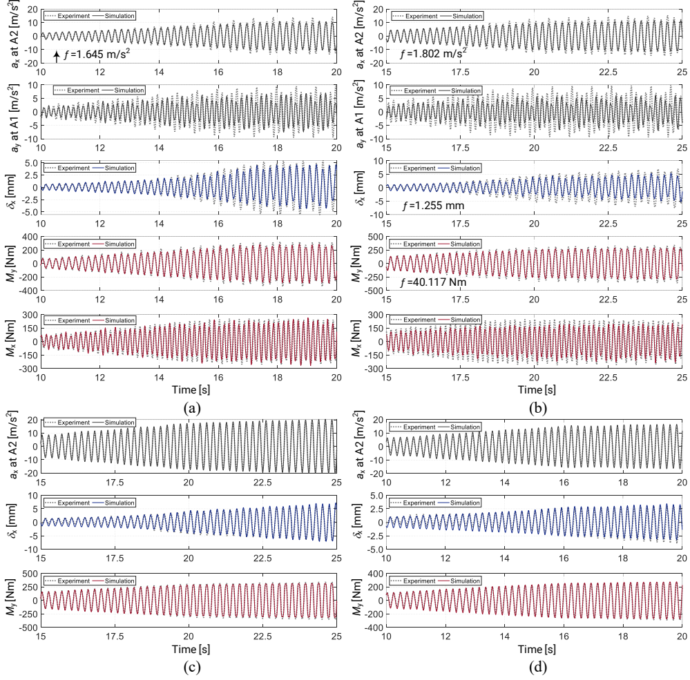
Figure 13: Comparison of test data and simulated values of the responses of interest from the test used for identification and from the verification tests using the best parameter set found from case 1 (i.e., No. 2) for the predictions. Arrow indicates the response used for formulating f_2 . (a) Test No. 2; (b) Test No. 3; (c) Test No. 4; (d) Test No. 10.
