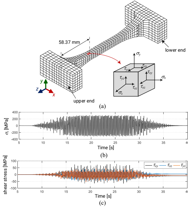
Figure 7: Example of histories of normal and shear stresses at the first integration point of an element of the specimen model. (a) Element of consideration; (b) Normal stress; (c) Shear stresses.
