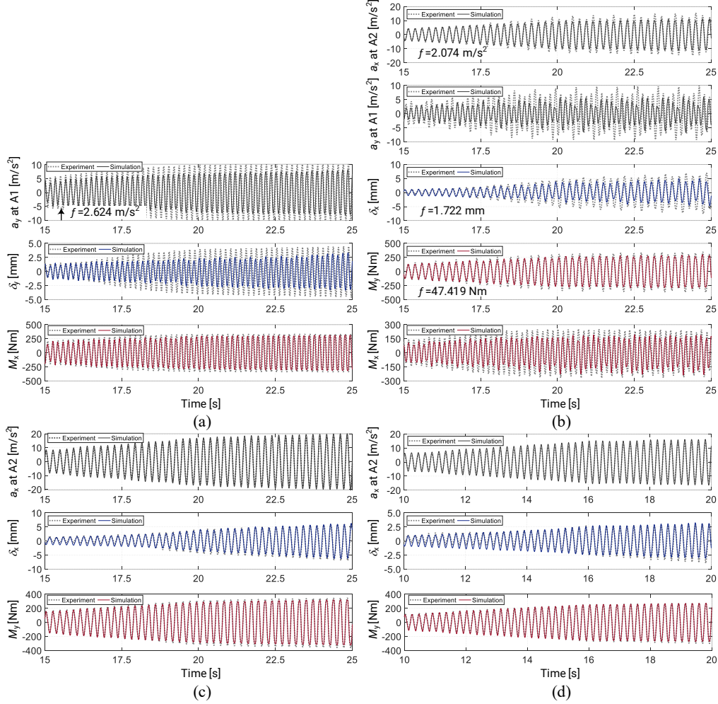
Figure 14: Comparison of test data and simulated values of the responses of interest from the test used for identification and from the verification tests using the best parameter set found from case 2 (i.e., No. 5) for the predictions. Arrow indicates the response used for formulating f_2 . (a) Test No. 5; (b) Test No. 3; (c) Test No. 4; (d) Test No. 10.
