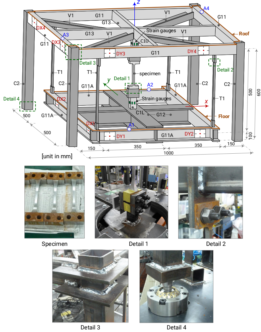
Figure 1: Schematic drawing of the experiment and some connection details.
