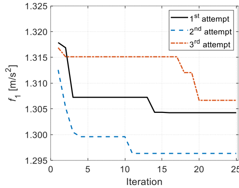
Figure 10: Histories of three BO attempts of the first identification step.
