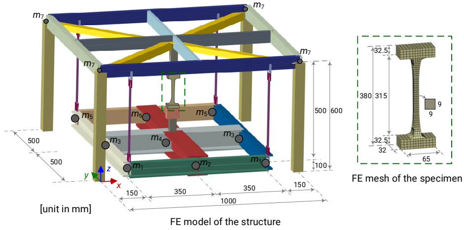
Figure 5: FE model of the structure and FE mesh of the specimen.
