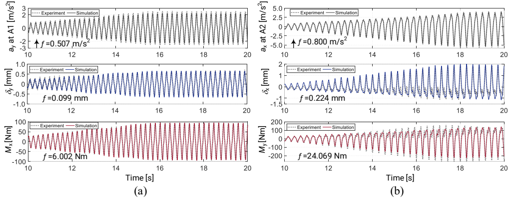
Figure 11: Comparison of test data and simulated values of the responses of interest from tests Nos. 1 and 6 with use of Young's modulus values identified from the 3rd BO attempt for the predictions. Arrows indicate the responses used for formulating f_1 . (a) Test No. 1; (b) Test No. 6.
