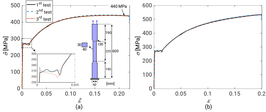
Figure 4: Geometric property of the rods used in three monotonic tension tests and stress-strain curves obtained from these tests. (a) engineering stress-strain; (b) true stress-strain.
