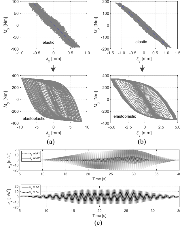
Figure 8: Examples of M_y - \delta_x and M_x - \delta_y curves in elastic and elastoplastic states of the structure, and acceleration histories at A1 and A2 on the floor. (a) M_y - \delta_x curves; (b) M_x - \delta_y curves; (c) a_x and a_y histories at A1 and A2.
