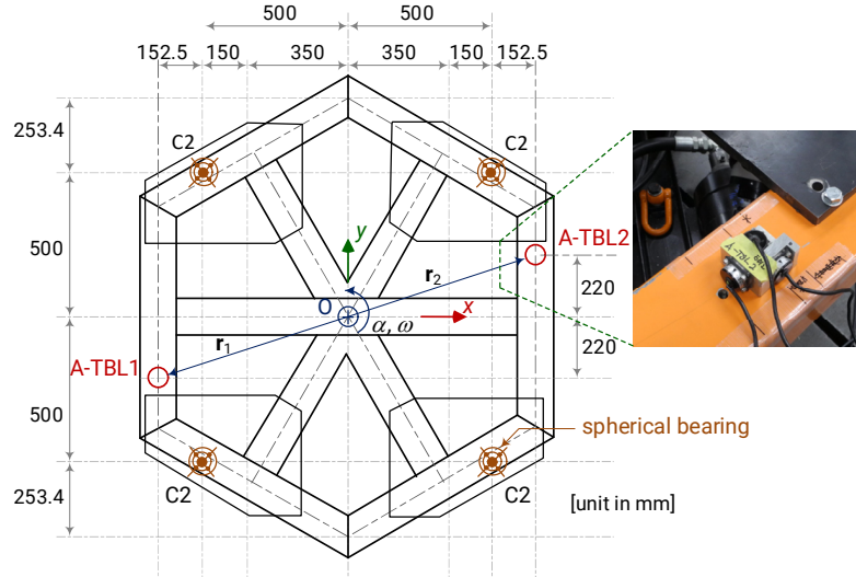
Figure 3: Accelerometers at A-TBL1 and A-TBL2 on the shaking table.
