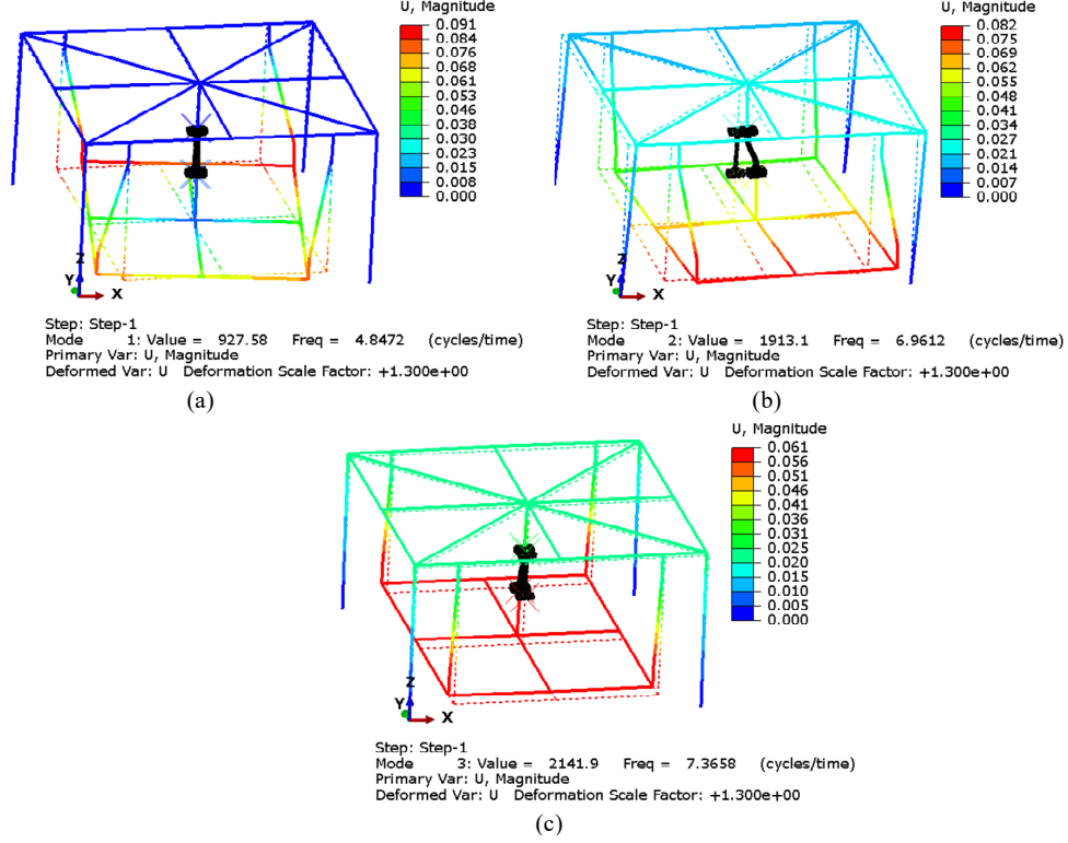
Figure 6: First three mode shapes of the structure for E = 205 and E_1 = E_2 = E_3 = 200 GPa. (a) 1st mode; (b) 2nd mode; (b) 3rd mode.
