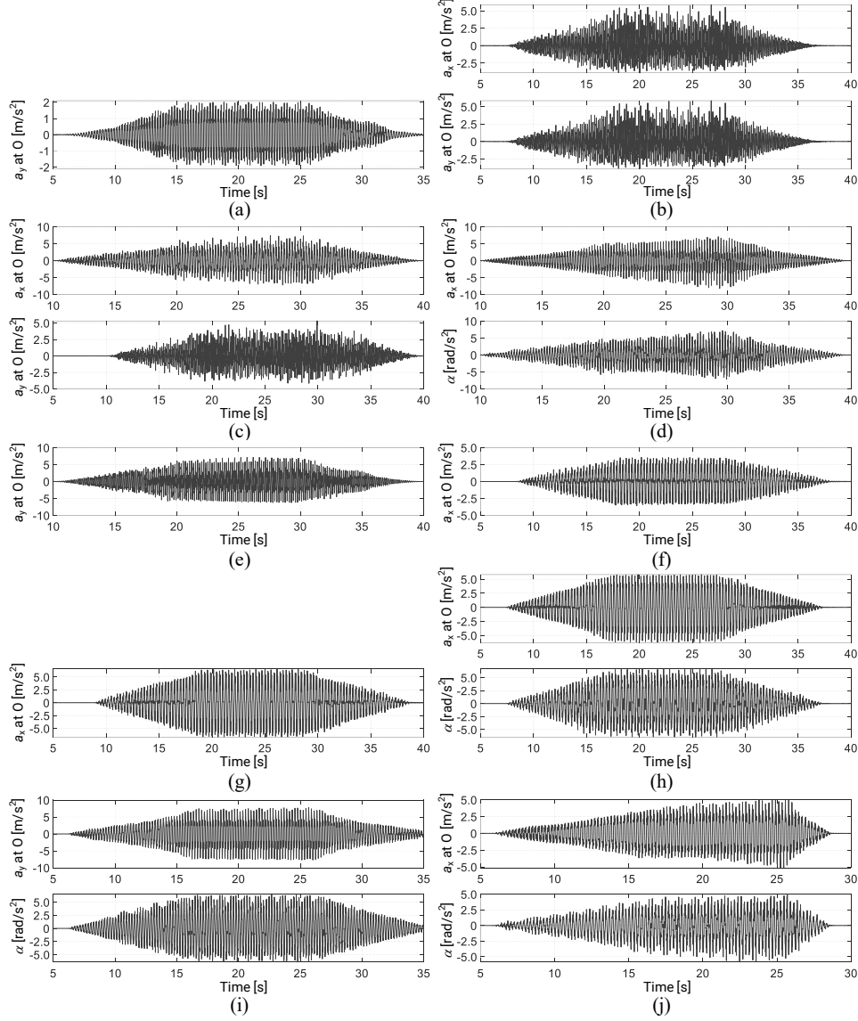
Figure 9: Input acceleration histories for the FE models associated with ten cyclic tests used for parameter identification and verification. (a)–(j) Nos. 1–10, respectively.
