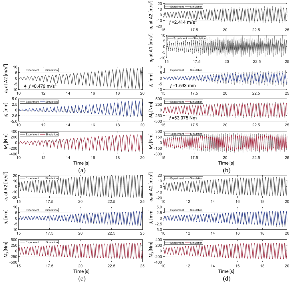
Figure 15: Comparison of test data and simulated values of the responses of interest from the test used for identification and from the verification tests using the best parameter set found from case 3 (i.e., No. 7). Arrow indicates the response used for formulating f_2 . (a) Test No. 7; (b) Test No. 3; (c) Test No. 4; (d) Test No. 10.
