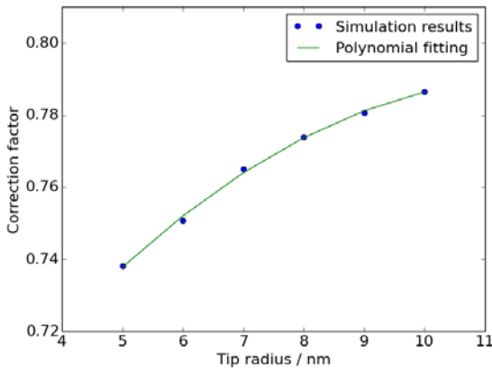
Fig. 3 Tip radius dependency of correction factor
