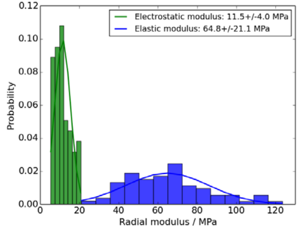
Fig. 7 Measured electrostatic and elastic moduli ( N=72 )
