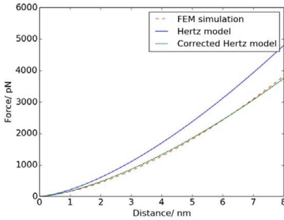
Fig. 2 Prediction of FEM simulation results by corrected Hertz model (tip radius: 9 nm, Young's modulus: 50 MPa)
