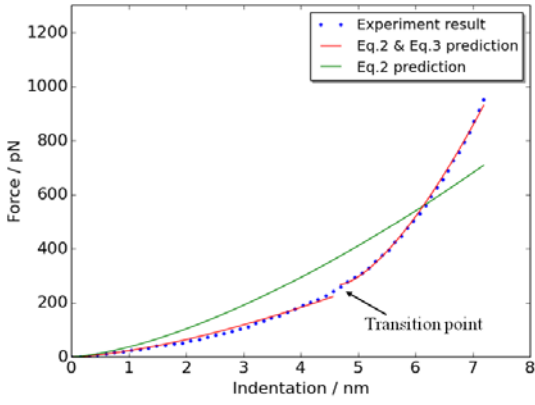
Fig. 5 Measured force-indentation data (blue dots) and fitted curves obtained by the corrected Hertz model, compared with single phase prediction (green line) and two-phase prediction (red lines).
