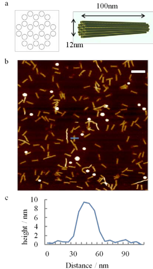
Fig. 1 Schematic configuration and AFM image of the designed DNA nanotubes. (a) Schematic view of DNA nanotube three-dimensional structure (right), with a cross-section showing the honeycomb lattice (left); (b) AFM image of DNA nanotubes deposited on mica substrate; (c) the cross-sectional profile of one DNA nanotube indicated by the
