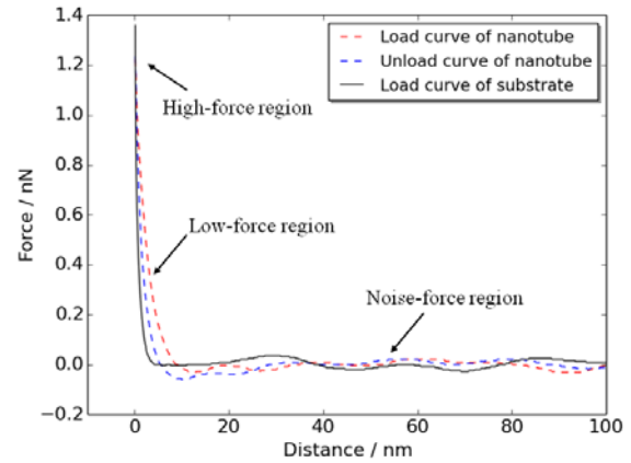
Fig. 4 Typical nanoindentation force-distance curves for DNA nanotubes on a mica substrate.
