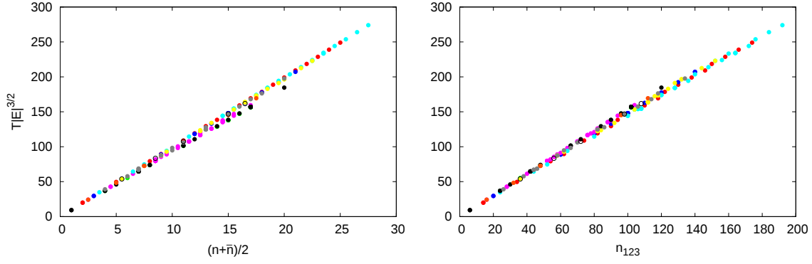
Figure 1: (color on-line) (a) Left panel: The scale-invariant periods |E|^{3/2}T(w) of more than 200 presently known zero-angular-momentum three-body orbits versus one half of the number of all letters in the free-group word w describing the orbit, N_w = n_w + \bar{n}_w , where n_w is the number of small letters a , or b , and \bar{n}_w is the number of capital letters A , or B in the word w . (b) Right panel: Same as (a), only in terms of the number of symbols n_{123} in the sequence of symbols (1,2,3) describing the topology of the orbit, see Appendix C. Color code: 1) red = sequence I - butterfly I; 2) green = sequence II - dragonfly; 3) dark blue = sequence III - yin-yang; 4) pink = sequence IVa - moth I; 5) light blue = sequence IVb - butterfly III; 6) yellow = sequence IVc - moth III; 7) black = sequence V - figure-eight; 8) orange = sequence VI - yarn; 9) grey = sequence VII - moth; 10) empty circles = other.
