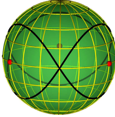
Figure 5: The shape-space sphere: the figure-eight orbit (solid black curve); three two-body collision points (red), singularities of the potential, lie on the equator.
