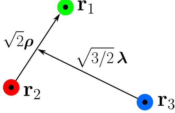
Figure 4: The two three-body Jacobi coordinates \rho, \lambda .
