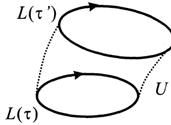
Figure 1: Transport of a loop and circulation [15]. Given a loop L in space, the circulation of a vector field \mathbf{P} is the integral \oint_L \mathbf{P} \cdot d\mathbf{x} . Two loops L(\tau) and L(\tau') , connected by the “flow” d\mathbf{x}/d\tau = \mathbf{U} (the parameter \tau may be regarded as time), are shown in the figure. A circulation theorem pertains to a “movement” of loops; the rate of change of circulation is calculated as (1). On a loop L(\tau) carried by the fluid (i.e., \tau = t and \mathbf{U} = \mathbf{V} ), the circulation is conserved because \oint_{L(t)} \nabla \mathcal{E} \cdot d\mathbf{x} \equiv 0 (Kelvin’s circulation law). To generalize the argument to the relativistic regime, we have to immerse the loop in the 4-d space-time and transport it by the 4-velocity dx_\mu/d\tau = U_\mu ; see Fig. 2. The explicitly Lorentz covariant equality, written in terms of the proper time \tau = s = ct/\gamma is found to be d(\oint_{L(s)} P^\mu dx_\mu)/ds = \oint_{L(s)} (\partial^\mu P^\nu - \partial^\nu P^\mu) U_\nu dx_\mu . Thus if the fluid equation could be cast in the form (\partial^\mu P^\nu - \partial^\nu P^\mu) U_\nu = \partial^\mu \phi , the circulation would, indeed, be conserved. The relativistic space-time circulation conserves in ideal fluids; see (2).
