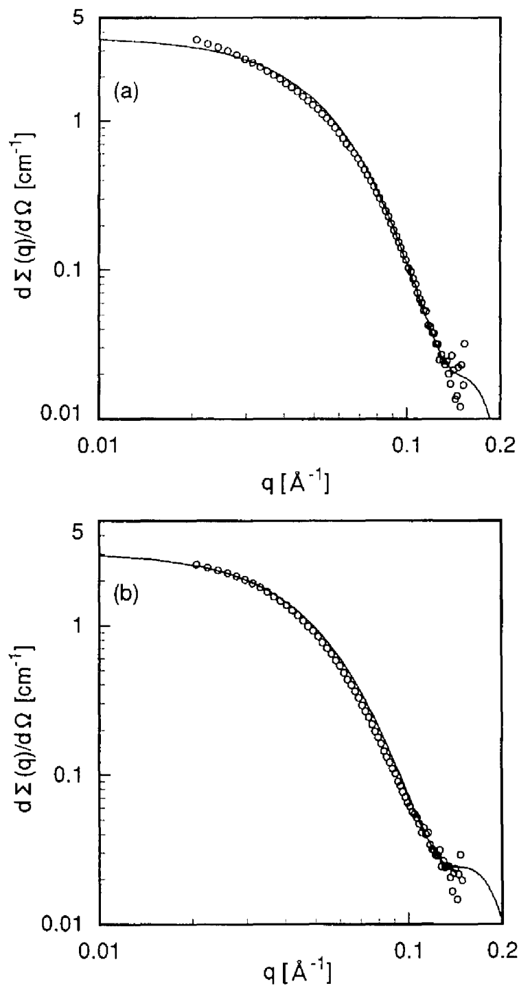
Figure 4.4. SANS profiles of \text{D}_2\text{O} solutions of OD20 (a) and OD30 (b). Solid lines are theoretical curves of spherical core-shell model.
