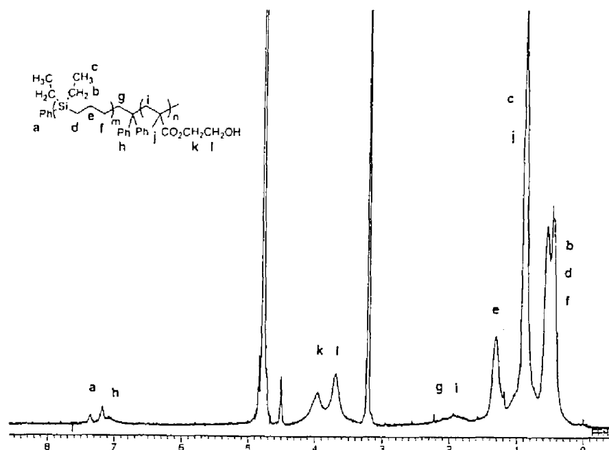
The tert -butyldimethylsilyl groups were easily hydrolyzed with 3M HCl in dioxane, and poly(1,1-diethylsilabutane)- block -poly(2-hydroxyethyl methacrylate) ( 11 ) was obtained. Figure 5.5 shows the ^1\text{H} NMR spectrum of polymer 11 in \text{CD}_3\text{OD} . It is noteworthy that signals ascribed to poly(1,1-diethylsilabutane), which is insoluble in methanol, could be observed. This result provides another evidence for the formation of the block copolymer. Because polymer 11 (1 wt %) was soluble in a polar solvent such as methanol or even in a methanol–water (1 : 5) mixture as well as in a nonpolar solvent such as chloroform, it can be considered as a nonionic amphiphilic block copolymer.
