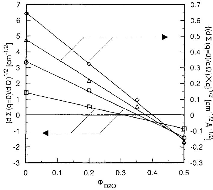
Figure 3.3. Square root of forward scattering intensity plotted against the volume fraction of D_2O : N8515 ( \square ), N8530 ( \circ ), N8545 ( \triangle ), and N8560 ( \diamond ). For the latter two cases, \{(d\Sigma(q=0)/d\Omega) \times q\}^{1/2} is plotted instead of forward scattering intensity. The solid lines are due to least-squares fits, and the crossing point with y = 0 is zero average contrast ( \phi_{ZAC} ).
