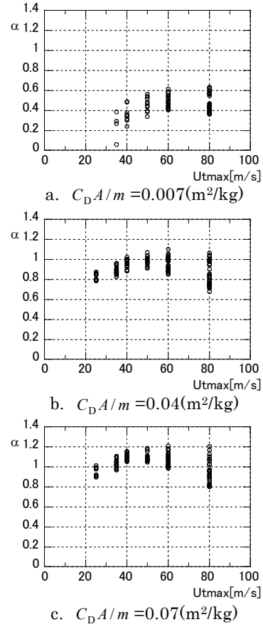
Fig. 16 Variation of amplification factor \alpha with maximum tangential speed U_{\text{tmax}}
