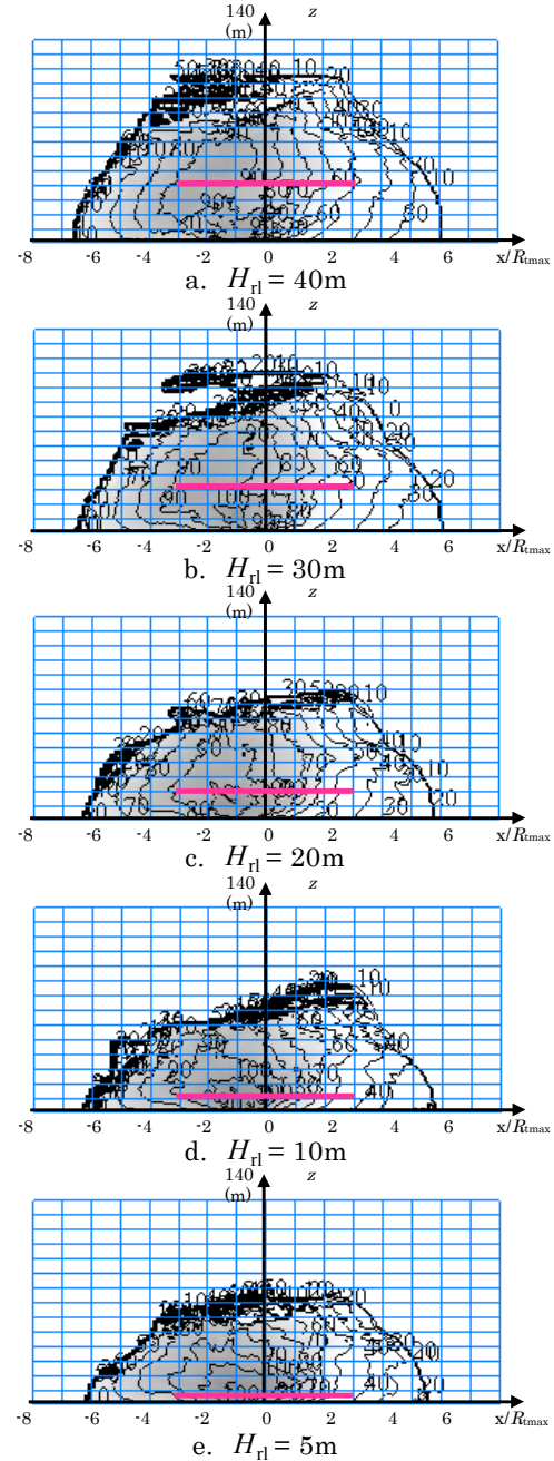
Fig. 10 Frontal view of contour plot of maximum ground speed of debris, U_{\text{emax}} (m/s). Variation with release height, H_{\text{rl}} . Release positions are on the red lines. C_D A / m = 0.07 (\text{m}^2/\text{kg}) , U_{\text{tmax}} = 80 (\text{m/s}) , R_{\text{tmax}} = 30 (\text{m}) , U_{\text{tr}} = 35 (\text{m/s})
