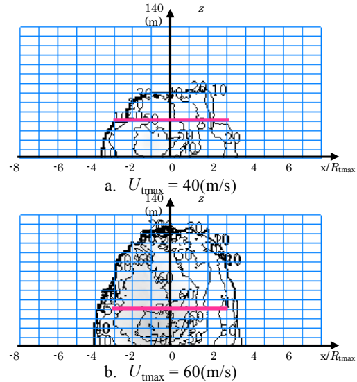
Fig. 13 Frontal view of contour plot of maximum ground speed of debris, U_{\max} (m/s). Variation with maximum tangential speed, U_{tmax} . Release positions are on the red lines. C_D A/m = 0.07 \text{ (m}^2/\text{kg)} , H_{rl}=40 (m), R_{tmax} = 60 (m), U_{tr} = 15 (m/s)
