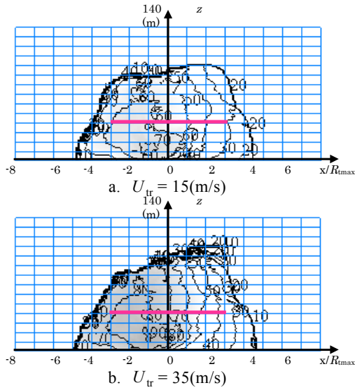
Fig. 14 Frontal view of contour plot of maximum ground speed of debris, U_{\text{emax}} (m/s). Variation with traveling speed, U_{\text{tr}} . Release positions are on the red lines. C_D A/m = 0.07(\text{m}^2/\text{kg}) , U_{\text{tmax}} = 60(\text{m/s}) , R_{\text{tmax}} = 40(\text{m}) , H_{\text{rl}} = 40(\text{m})
