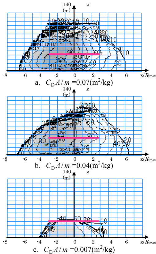
Fig. 11 Frontal view of contour plot of maximum ground speed of debris, U_{\max} (m/s). Variation with aerodynamic parameter, C_D A/m . Release positions are on the red lines. H_{rl}=40 (m), U_{tmax} = 80 (m/s), R_{tmax} = 30 (m), U_{tr} = 35 (m/s)
