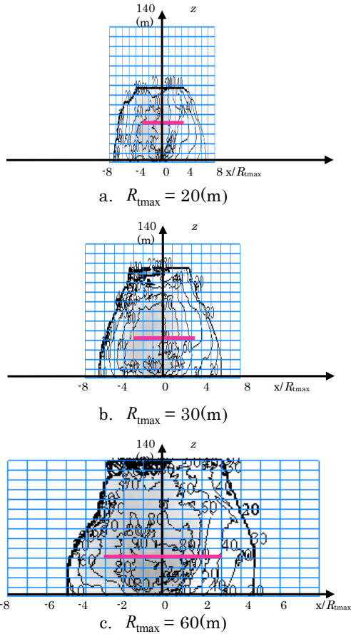
Fig. 15 Frontal view of contour plot of maximum ground speed of debris, U_{\text{emax}} (m/s). Variation with maximum tangential speed radius, R_{\text{tmax}} . Release positions are on the red lines. C_D A/m = 0.07(\text{m}^2/\text{kg}) , U_{\text{tmax}} = 80(\text{m/s}) , H_{\text{rl}} = 40(\text{m}) , U_{\text{tr}} = 15(\text{m/s})
