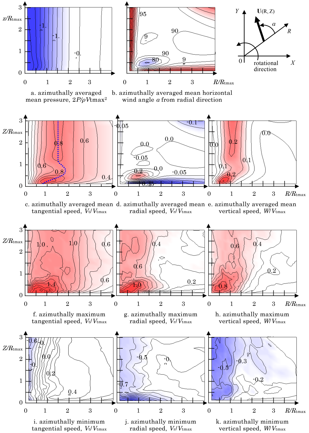
Fig. 4 Distributions of velocity and pressure field of single core two cell type shown in Figure 3 in a vertical plane.
