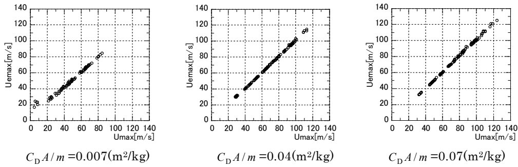
Fig. 9 Maximum ground effective speed U_{\text{emax}} vs Maximum ground horizontal speed U_{\text{hmax}}
