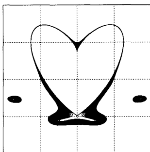
図 6: conplot
