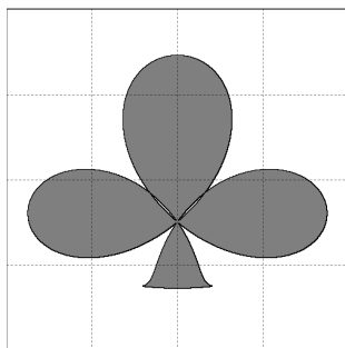
☒ 12: ineqnQ(-C,Gray50)
