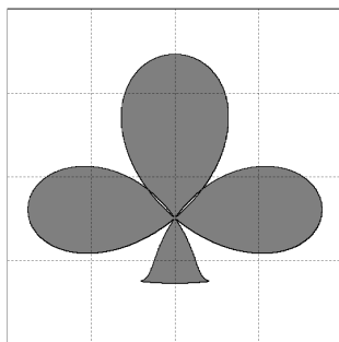
☒ 11: ineqnD(-C,Gray50)
