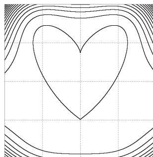
☒ 10: conplotB(H)
