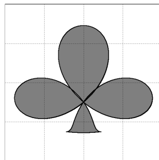
☒ 13: ineqnB(-C,Gray5)0
