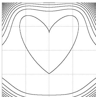
☒ 8: conplotD(H)
