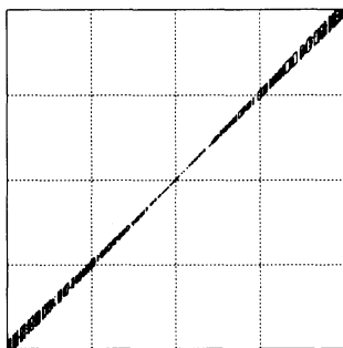
図 3: ifplotD
