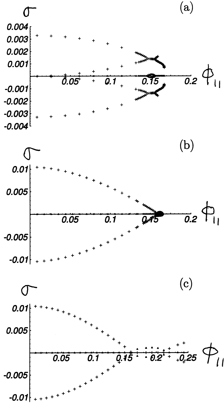
Figure 3: Frequency [-\Re(\sigma_{\pm 26})] (+) and growth rate [-\Im(\sigma_{\pm 26})] ( \blacktriangle ) as a function of coefficient \phi_{11} for depth d = 1 and angle \theta = 66^\circ : (a) branch I; (b) branch II; (c) branch III. See Figure 2 for definition of the branches.
