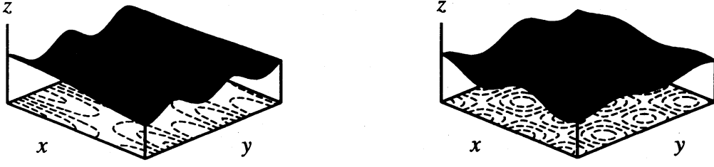
FIG 1: Short-crested wave fields for angles \theta = 10^\circ (left) and \theta = 45^\circ (right) on deep water.
