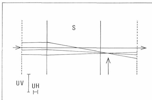
Fig. 4 Optics near the sample compartment of UV-200. S; sample compartment, UV; 1 cm in the vertical direction, UH; 1 cm in the horizontal direction
