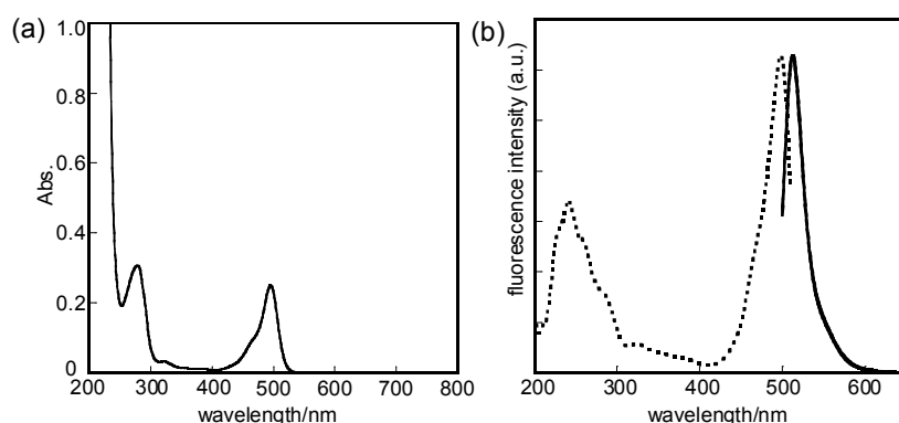
Figure 19. a) UV-visible spectroscopy of the FL-Con A. b) Excitation (dot line) and emission (solid line) spectra of FL-Con A, \lambda_{\text{ex}} = 488 \text{ nm} , \lambda_{\text{em}} = 513 \text{ nm} .
