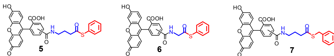
Figure 23. Molecular structures of acyl donors 5-7 .
