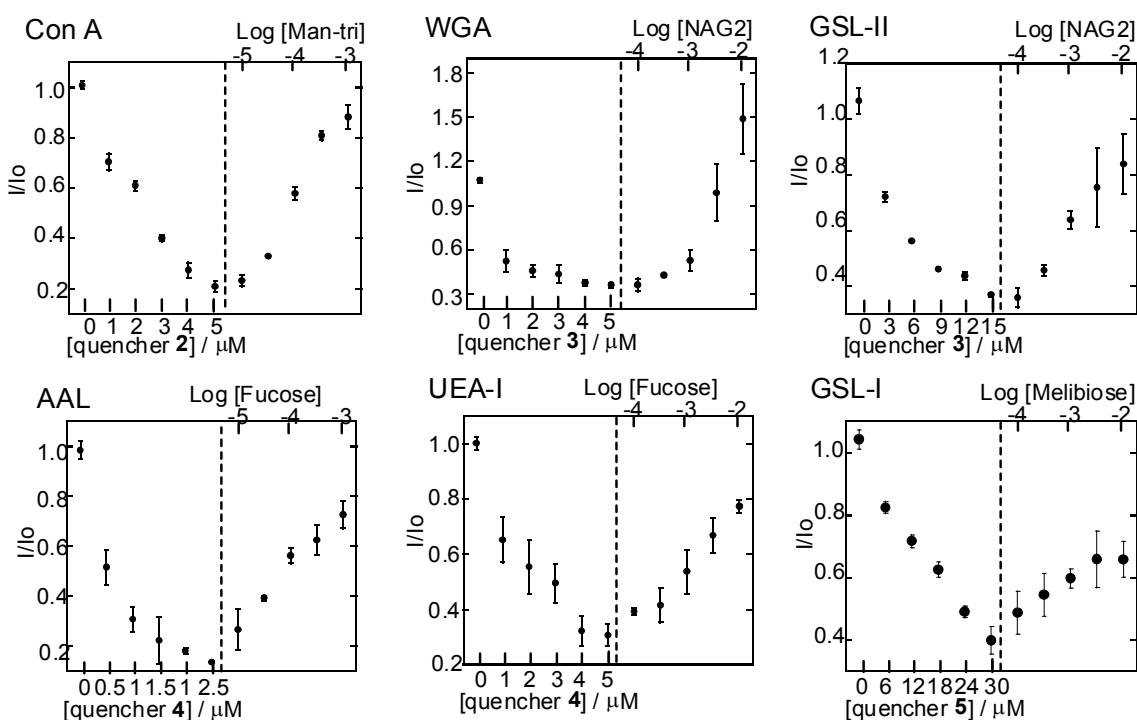
Figure 15. Fluorescent titration curve of Fluorescein-labeled lectins with quenchers and saccharides in hydrogel matrix. [\text{FITC-lectin}] = 1 \mu M in 50 mM HEPES buffer (pH 7.5, containing 1 mM \text{MnCl}_2 , 1 mM \text{CaCl}_2 , 0.1 M NaCl), in 0.25 wt% of 1 , 20^\circ \text{C} , \lambda_{\text{ex}} = 475 \text{ nm} . The error bar in graph mean standard deviation of independent 3 times measurement.
