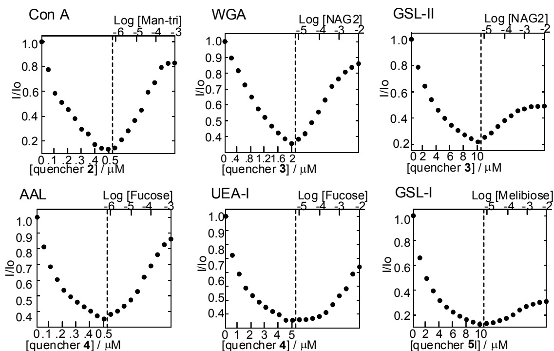
Figure 14. Fluorescent titration curve of Fluorescein-labeled lectins with quenchers and saccharides in aqueous solution. [\text{FITC-lectin}] = 0.1 \mu M in 50 mM HEPES buffer (pH 7.5, containing 1 mM \text{MnCl}_2 , 1 mM \text{CaCl}_2 , 0.1 M NaCl), 20^\circ \text{C} , \lambda_{\text{ex}} = 488 \text{ nm} .
