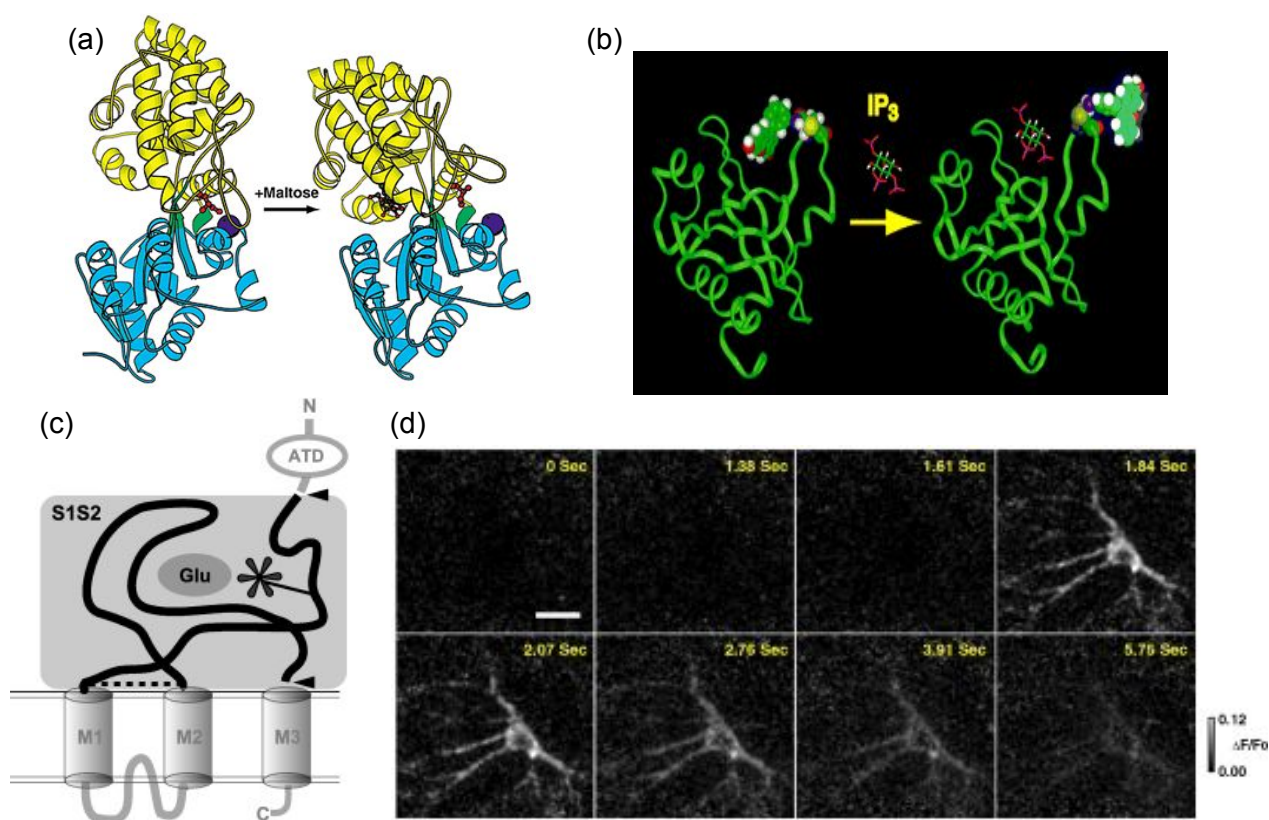
Figure 2. Schematic illustration of ligand mediated conformational changes in fluorescent biosensor for maltose (a) 4 , IP 3 (b) 5 and glutamate (c) 6 . (d) Visualization of the glutamate release from neuron cells using the glutamate biosensor. 6
