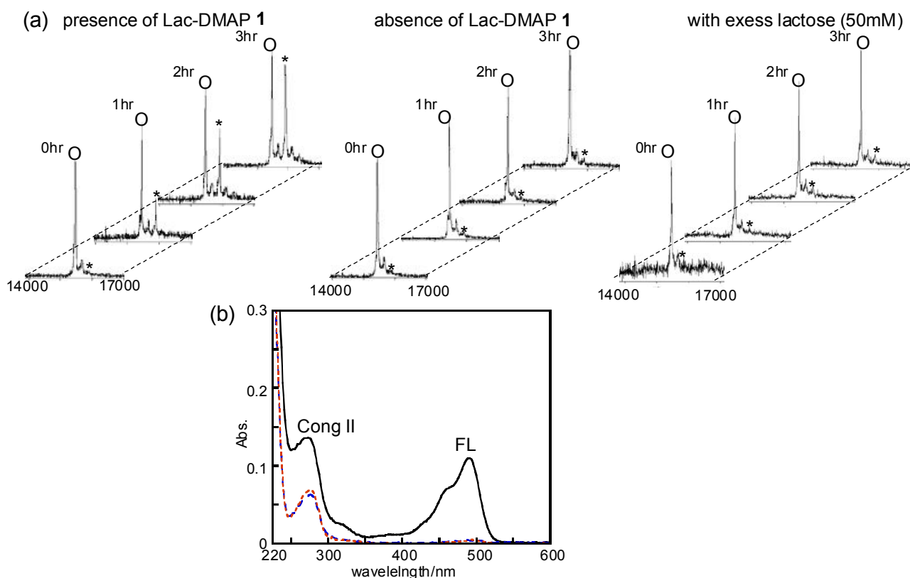
Figure 12. (a) MALDI-TOF mass spectra of reaction mixture of Cong II (10 \mu M) with Lac-DMAP 1 (50 \mu M) and acyl donor 5 (50 \mu M) (O ; native Cong II ( M_w 15,330), * ; FL-Cong II ( M_w 15,770)).
