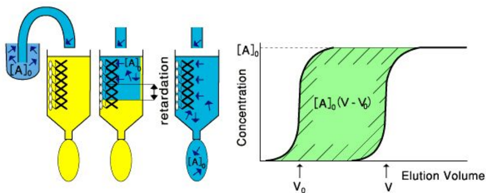
Figure 18. Principle of FAC: “A” (e.g., sugar) is continuously applied to a column, where affinity ligand “B” (e.g., lectin) is immobilized. If “A” has affinity to “B,” elution front of “A” is retarded. 29a
