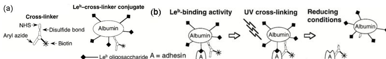
Figure 6 (a) A multifunctional cross-linking agent was conjugated to the Le b glycoconjugate. (b) The labeling for the adhesin of H. Pylori . 7
