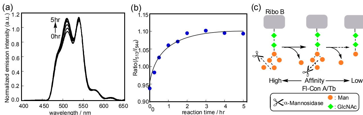
Figure 14. (a) Time dependent spectral change of the emission of FL-Con A/Tb in the presence of Ribo B by addition of \alpha -mannosidase (0 \rightarrow 5hr). (b) Time profile of the ratiometric intensity ( I_{513}/I_{544} ). (c) Illustration of luminescent sensing scheme of the branched mannide on Ribo B by \alpha -mannosidase.
