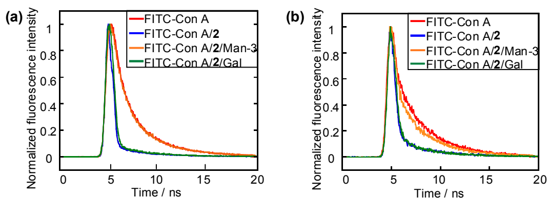
Figure 10. Fluorescent lifetime study of FITC-Con A in aqueous solution (a) and in hydrogel 1 matrix (b).
