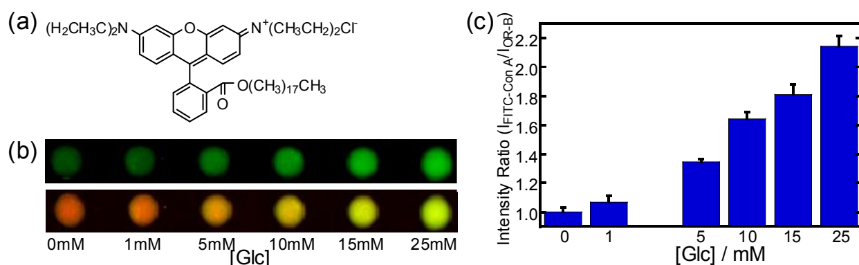
Fig.13 (a) Molecular structure of octadecyl rhodamine B chloride (OR-B). (b) Clear image of glucose using Con A chip containing OR-B. Upper; fluorescent image of FITC-Con A for various concentration of glucose by fluorescein-excitation. Lower; fluorescent merged image by fluorescein (green) excitation and by OR-B (red) excitation. (c) The graph of fluorescent ratio (F-Con A / OR-B) by the addition of various concentration of glucose. [FITC-Con A] = 0.1 \mu M, [quencher 2 ] = 0.5 \mu M. The bar height and the error bar were estimated by the average and standard deviation of 4 spots on the same plate
