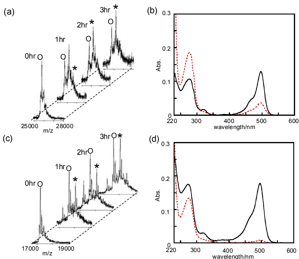
Figure 16. (a) MALDI-TOF mass spectra of reaction mixture of Con A and Man4-DMAP 4 and acyl donor 5 (O ; native Con A (M w 25,600), * ; FL-Con A (M w 26,040)). (b) Absorption spectra of fluorescein labeled Con A in the presence (black line), the absence (red dot line) of 4 . (c) MALDI-TOF mass spectra of reaction mixture of WGA and NAG3-DMAP 3 and acyl donor 5 (O ; native WGA (M w 17,100), * ; FL-WGA (M w 17,540)). (d) Absorption spectra of fluorescein labeled WGA. in the presence (black line), the absence (red dot line) of 3
