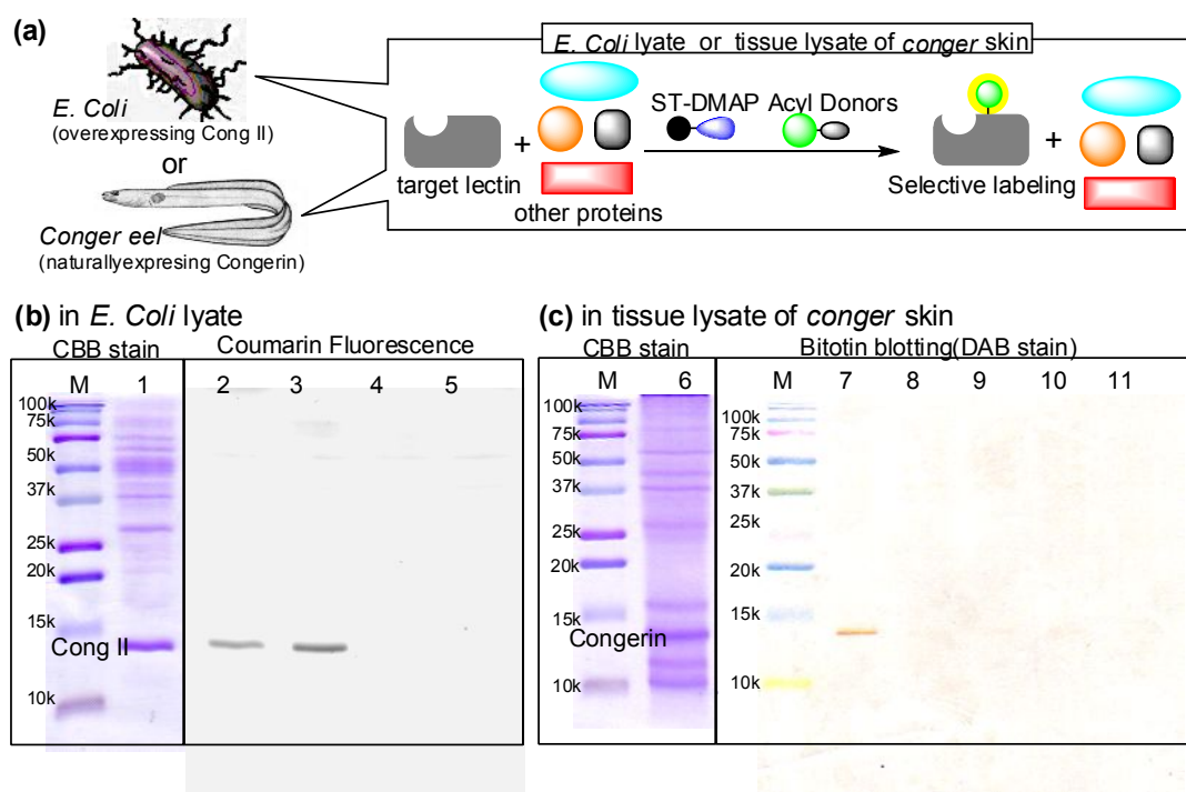
Figure 18. (a) Schematic illustration of selective acylation of lectin in crude mixtures. Protein modification was detected by SDS-PAGE: CBB staining (lane M, 1, 6); coumarin fluorescence (lane 2-5); biotin blotting (lane 7-11). (b) Coumarin labeling in cell lysates of E. coli overexpressing Cong II. (c) Biotin labeling in tissue lysates of conger skin mucus. Lane = M: protein marker, 1: whole proteins of E. coli , 2: Lac-DMAP 1, 3: Lac4-DMAP 2, 4: Lac4-DMAP 2 with 50mM Lactose, 5: in the absence of DMAP, 6: whole proteins of conger skin mucus, 7: Lac4-DMAP 2, 8: Man4-DMAP 4, 9: NAG3-DMAP 3, 10: Lac4-DMAP 2 with 50mM Lactose, 11: in the absence of DMAP. Reaction conditions: 50 \mu M sugar-tethered DMAPs, 50 \mu M acyl donor, pH 8.0, 3h, 25 ^{\circ} C.
