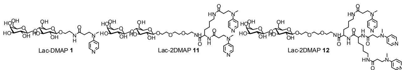
Figure 21. Molecular structures lactose-tethered multi DMAPs 1 , 11 , 12 .
