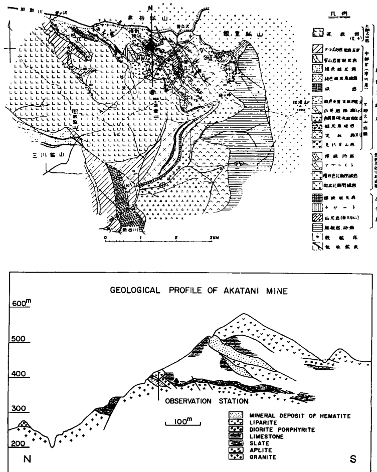
Fig. 2 Geological map and cross section (supplied by the Akatani mine). ▲: observational room.
