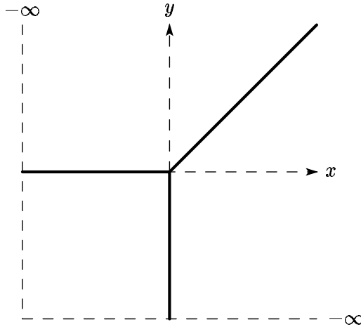
Figure 1: V(x \oplus y \oplus 0)
