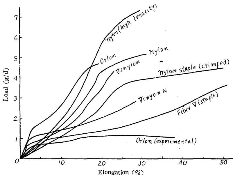
Fig. 1. Stress-strain curves for various synthetic fibers
