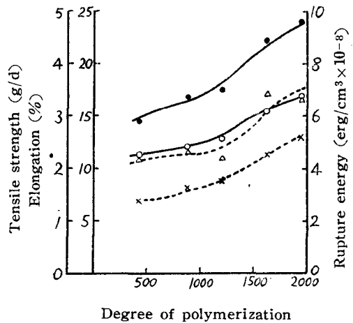
Fig. 4. Relation between mechanical properties of Vinyon and its degree of polymerization
