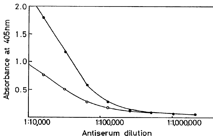
Fig. 2. Antiserum dilution curves. Either 1 \mu\text{g/ml} (○) or 5 \mu\text{g/ml} (●) of desmosine-KLH was coated in the wells. Serial dilutions of the rabbit antiserum were added to the wells. The amount of bound antibody was determined by incubating with alkaline phosphatase labeled IgG diluted 1:1000 and 2.7 mM p-nitrophenylphosphate. The enzyme activity was measured by the absorbance at 405 nm.
