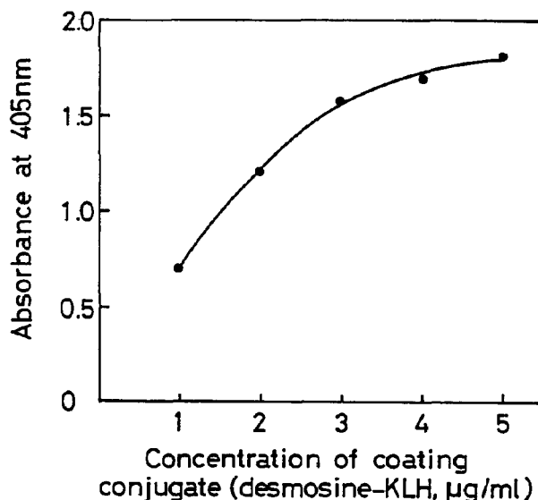
Fig. 4. The concentration of coating conjugate and the absorbance of blank solution. Using the plates coated with serially diluted desmosine-KLH conjugate from 5 to 1 \mu\text{g/ml} , the enzyme activities in the blank solution were determined as in Fig. 3. Antiserum diluted at 1:15,000 was used.
