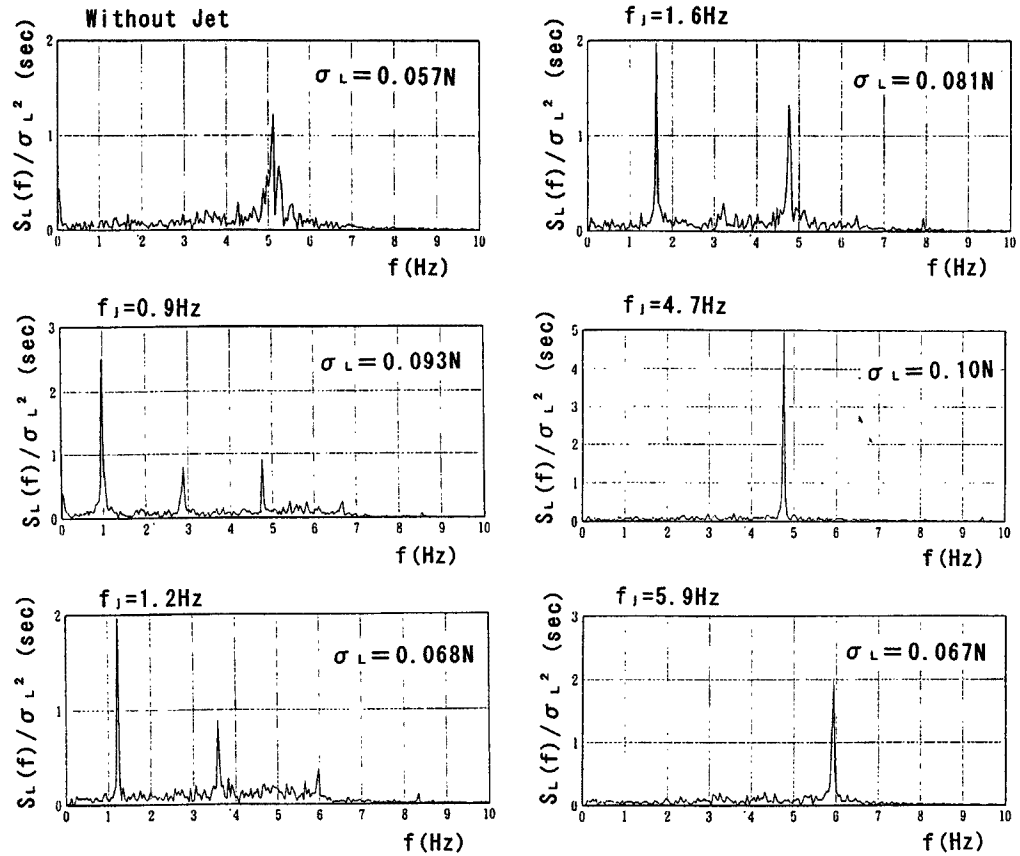
Fig. 6 Spectra of fluctuating lift force of the model with alternately fluctuating jet. ( U=4 m/sec, C_q=0.25\% )
