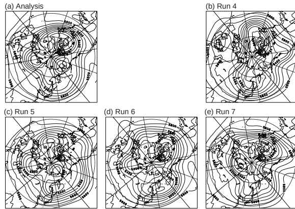
Fig.2. Three-day mean geopotential height field at 500 hPa for the period of 00 UTC 23 December 1998–12 UTC 25 December 1998. (a) Observation; (b) Run 4 from 12 UTC 26 November 1998; (c) Run 5 from 12 UTC 3 December 1998; (d) Run 6 from 12 UTC 10 December 1998; (e) Run 7 from 12 UTC 16 December 1998. Contour interval is 100 m. during the period of November 1998–January 1999.
