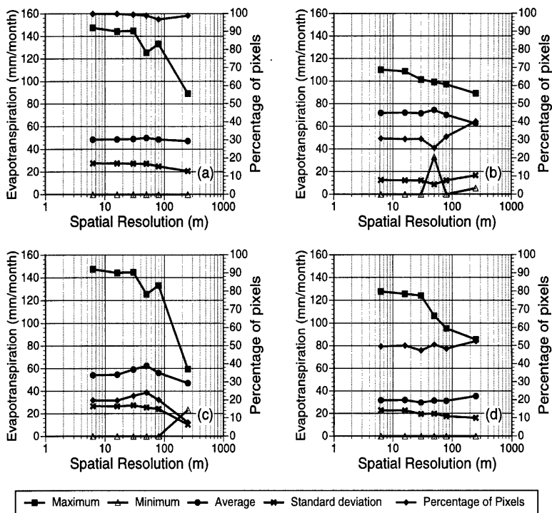
Fig. 6 Relationship between spatial resolution and estimated evapotranspiration in Site 1.
