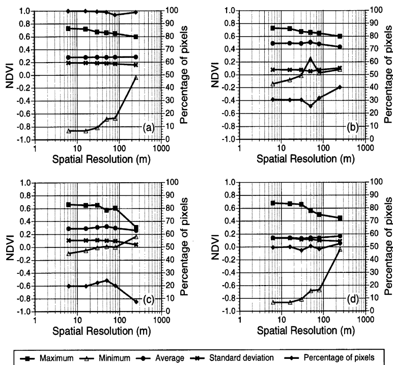
Fig. 2 Relationship between spatial resolution and NDVI in Site 1.
