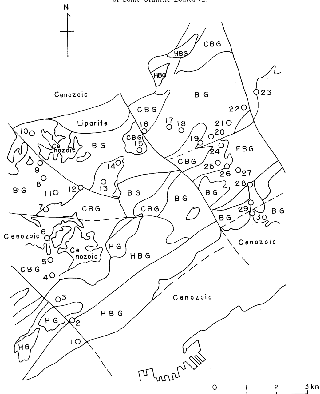
Fig. 3 Geological and sample station map (the west part of Rokkô). CBG : coarse-grained biotite granite BG : medium-grained biotite granite FBG : fine-grained biotite granite HBG : hornblende-bearing biotite granite
