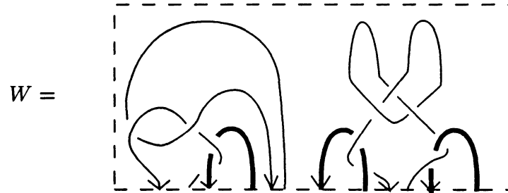
Figure 14: An even-trivial bottom tangle W \in BT_6 . Here W^{\text{ev}} is depicted with thick lines.
