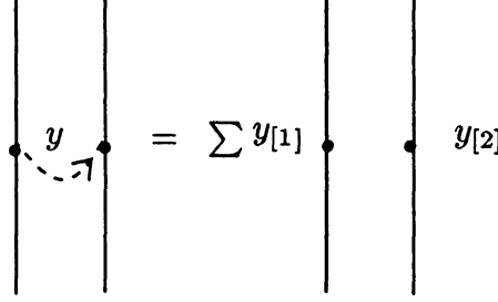
Figure 6: How we read an element y = \sum y_{[1]} \otimes y_{[2]} \in U_h^{\hat{\otimes} 2} .
