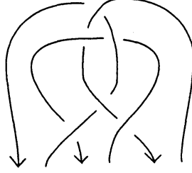
Figure 20: The Borromean tangle B \in BT_3 .
