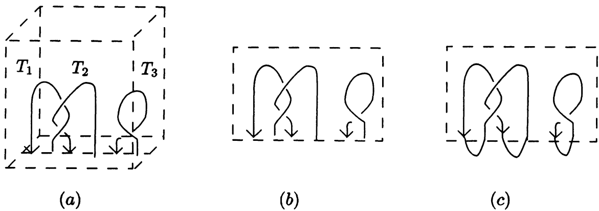
Figure 2: (a) A 3-component bottom tangle T = T_1 \cup T_2 \cup T_3 . (b) A diagram of T in a rectangle. (c) A closure of T .
