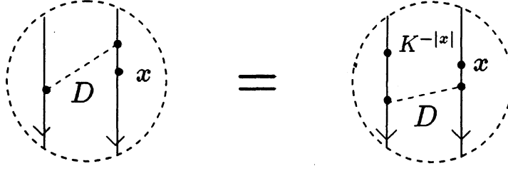
Figure 19: The sliding process of D .
