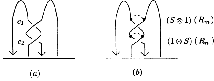
Figure 7: (a) A diagram P of C \in BT_2 . (b) The diagram P attached elements.
