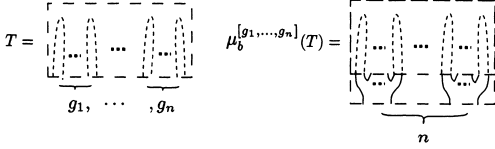
Figure 11: A bottom tangle T \in BT_k and the bottom tangle \mu_b^{[g_1, \dots, g_n]}(T) \in BT_n .
