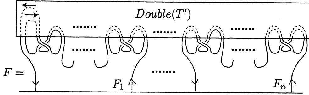
Figure 9: An arranged Seifert surfaces of the bottom tangle T .
