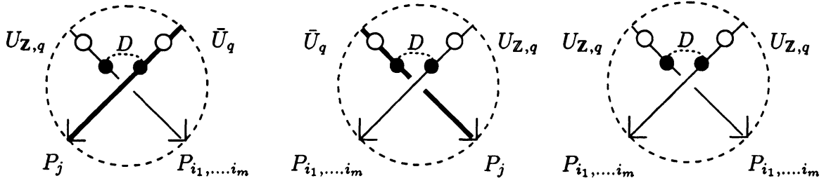
Figure 18: How we treat \alpha_m \otimes \beta_m .
