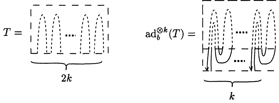
Figure 13: A bottom tangle T \in BT_{2k} and the bottom tangle \text{ad}_b^{\otimes k}(T) \in BT_k .
