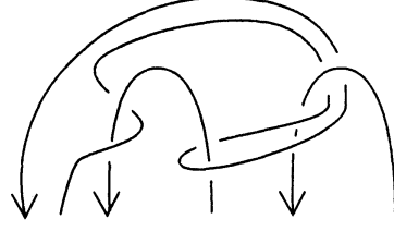
Figure 16: A diagram of the Borromean tangle P = P_1 \cup P_2 \cup P_3 , where P_2 \cup P_3 is the trivial diagram.
