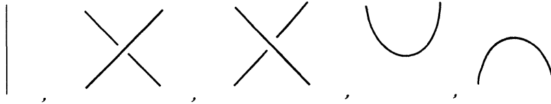
Figure 3: Fundamental tangles. The orientations of the strands are arbitrary.
