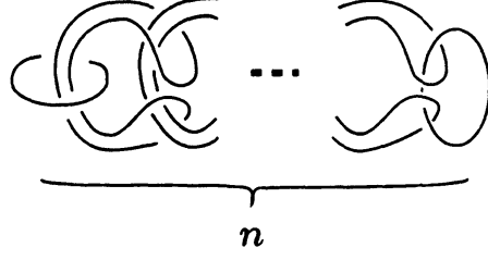
Figure 21: Milnor's link L_{M,n} .
