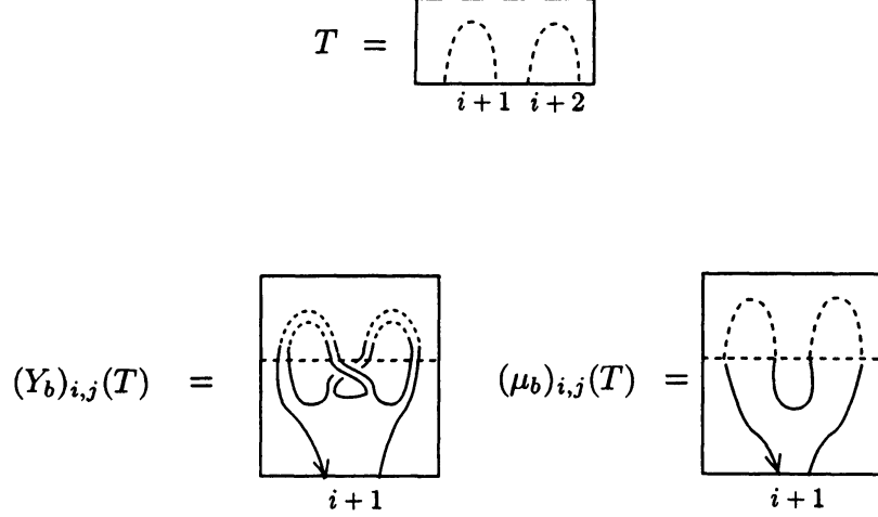
Figure 8: A bottom tangle T \in BT_{i+j+2} and the bottom tangles (Y_b)_{(i,j)}(T) , (\mu_b)_{(i,j)}(T) \in BT_{i+j+1} . We depict only the (i+1) , (i+2) th components of T , and the (i+1) th components of (Y_b)_{(i,j)}(T) , (\mu_b)_{(i,j)}(T) .
