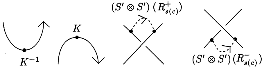
Figure 4: How to attach elements on the fundamental tangles.
