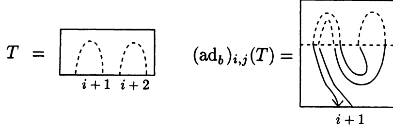
Figure 12: A bottom tangle T \in BT_{i+j+2} and the bottom tangles (\text{ad}_b)_{(i,j)}(T) . We depict only the (i+1), (i+2) th components of T , and the (i+1) th components of (\text{ad}_b)_{(i,j)}(T) .
