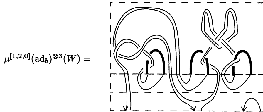
Figure 15: The ribbon bottom tangle \mu^{[1,2,0]}(\text{ad}_b)^{\otimes 3}(W) \in BT_3 for the even-trivial bottom tangle W \in BT_3 in Figure 14.
