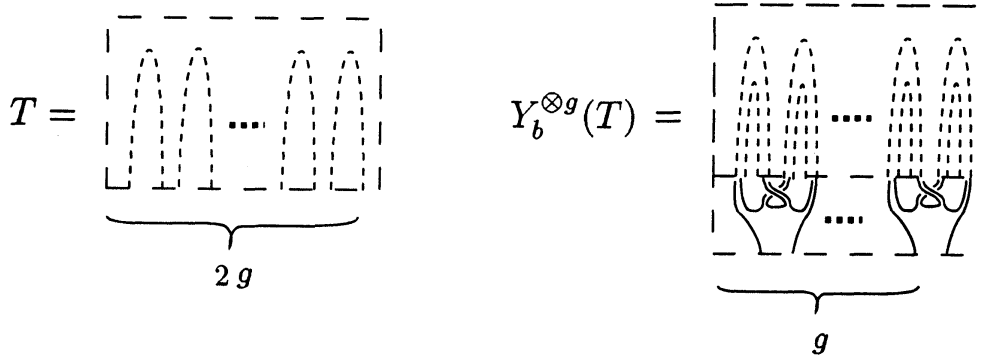
Figure 10: A bottom tangle T \in BT_{2g} and the bottom tangle Y_b^{\otimes g}(T) \in BT_g .
