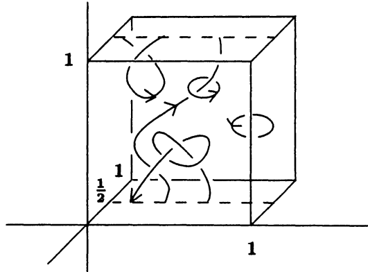
Figure 1: A tangle consisting of 3-arc components and 2-cycle components.
