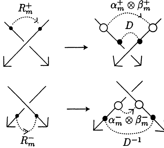
Figure 17: The modification process of elements on positive and negative crossings.
