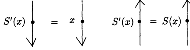
Figure 5: The definition of S' .
