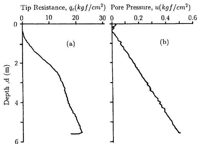
Fig. 8. Variation of Cone Tip Resistance, q_c , and Pore Pressure, u , with Penetration Depth, d (Case 4-1).
