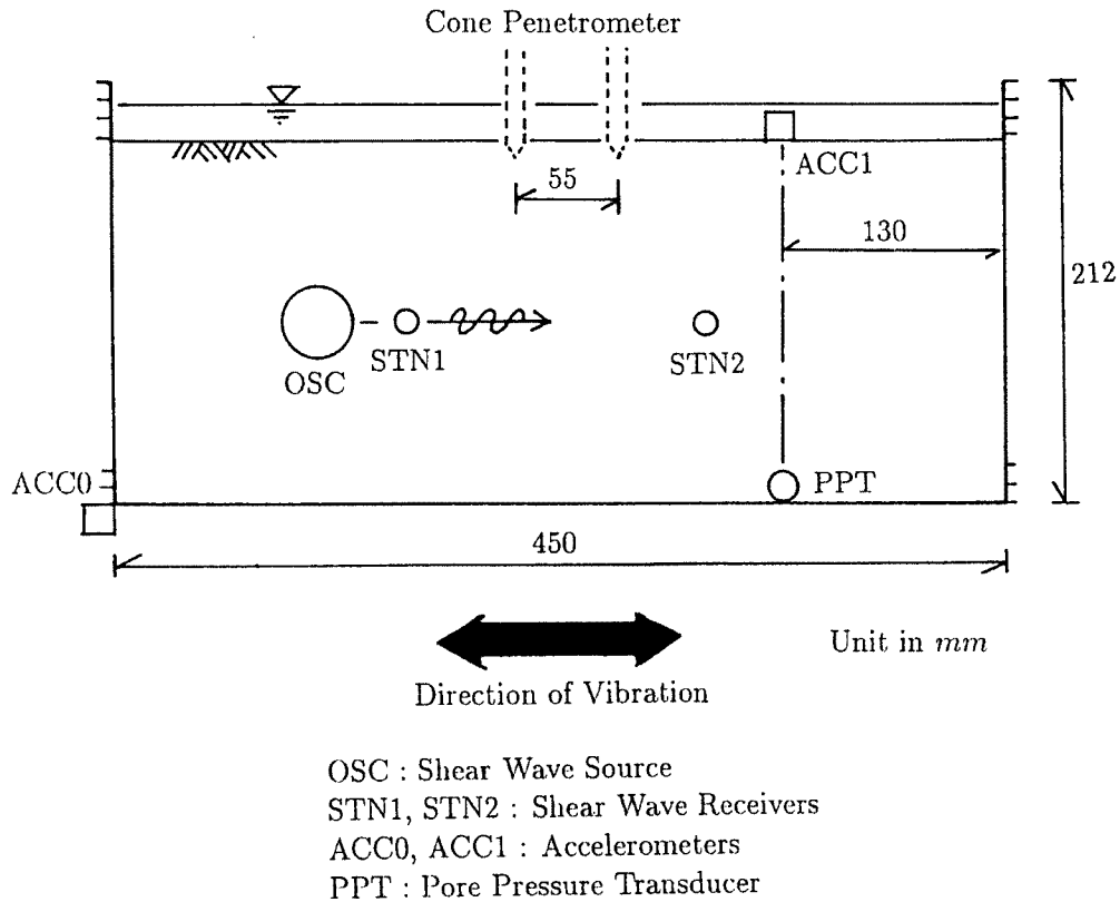
Fig. 1. Location of Transducers and Devices for Shaking Table Tests and Measurement of Shear Wave Velocities.
