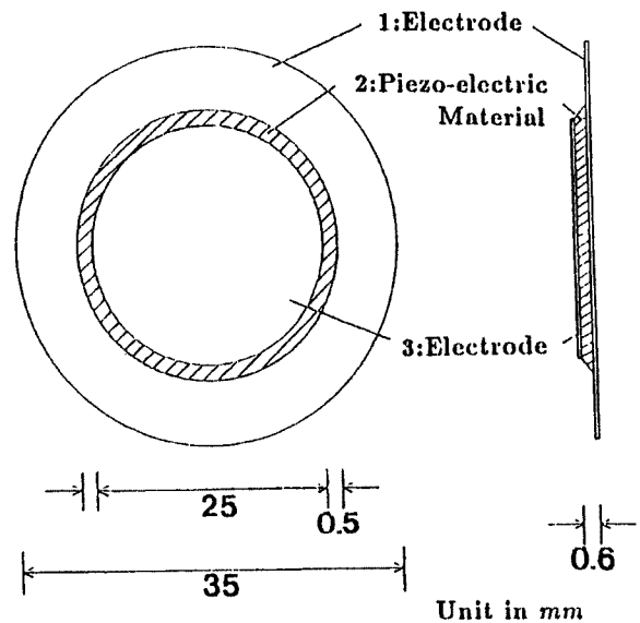
Fig. 2. Piezo-electric Oscillator.
