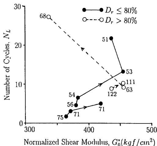
Fig. 14. Correlation between Normalized Shear Modulus, G_0^* , and Number of Cycles to Cause Liquefaction, N_L .
