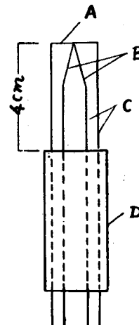
Fig. 1. Diagram of the thermocouple anemometer.
