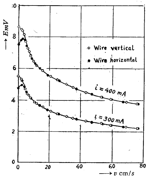
Fig. 8. Correlation plots of E versus v with constant i for two different orientations of the hot wire.
