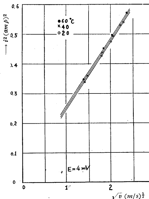
Fig. 10. Correlation plots of i^2 versus \sqrt{v} for wind of three different temperatures.
