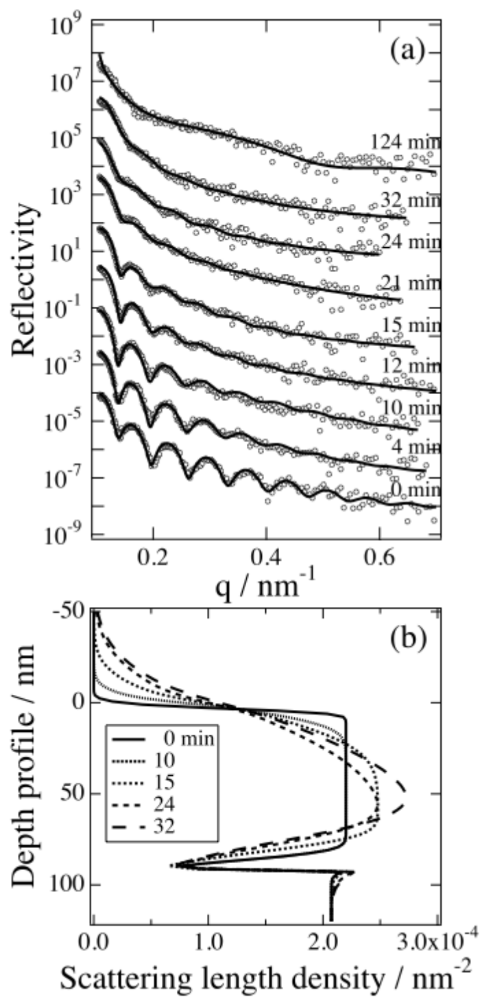
Figure 6.2: Time evolution of NR (a) and depth profile of scattering length density (b) of 98 nm dPS/PVME blend thin films after temperature jump to 125 °C.
