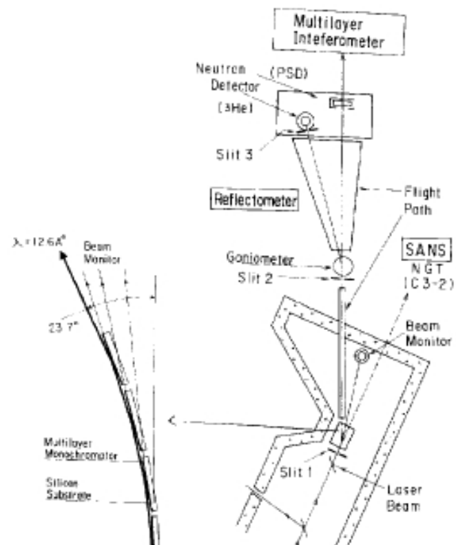
Figure 2.10: Schematic view of MINE.
