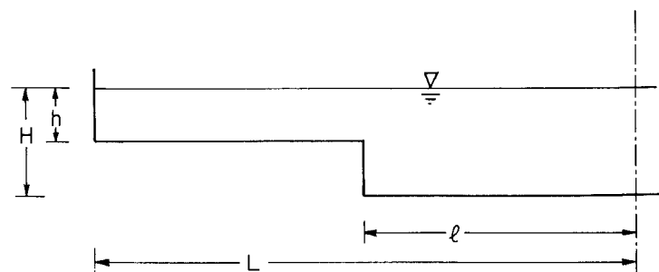
THE WIDE SYMMETRIC CHANNEL
