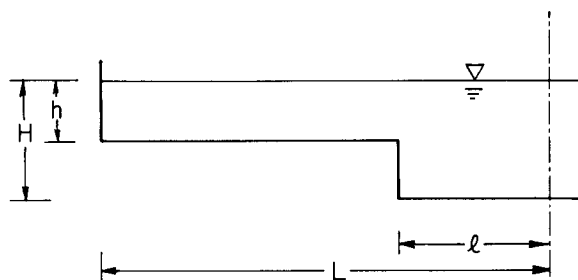
THE SYMMETRIC SMOOTH CHANNEL
