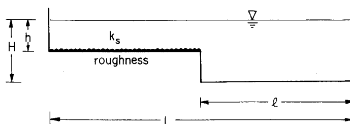
ASYMMETRIC CHANNEL WITH ROUGH FLOOD PLAIN
