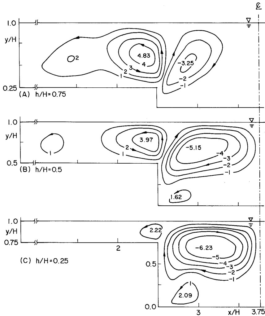
Fig. 8 Lateral Stream Function, 10^3 \phi / \langle W \rangle H , for Re_H = 10^5 in the Symmetric Smooth Channel.
