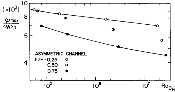
Fig. 17 Dependence of the Vortex Pair Intensity, 10^3 \psi_{\max} / (\langle W \rangle h) , at the Flood Plain Threshold on the Reynolds Number, Re_{DH} .
