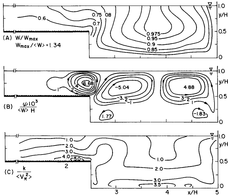
Fig. 12 The Asymmetric Channel with Rough Flood Plain Features : (A) W/W_{max} , (B) 10^3 \phi / \langle W \rangle H , and (C) k / \langle U_*^2 \rangle . ( Re_H = 10^5 , k_s/H = 0.024 , h/H = 0.5 ).
