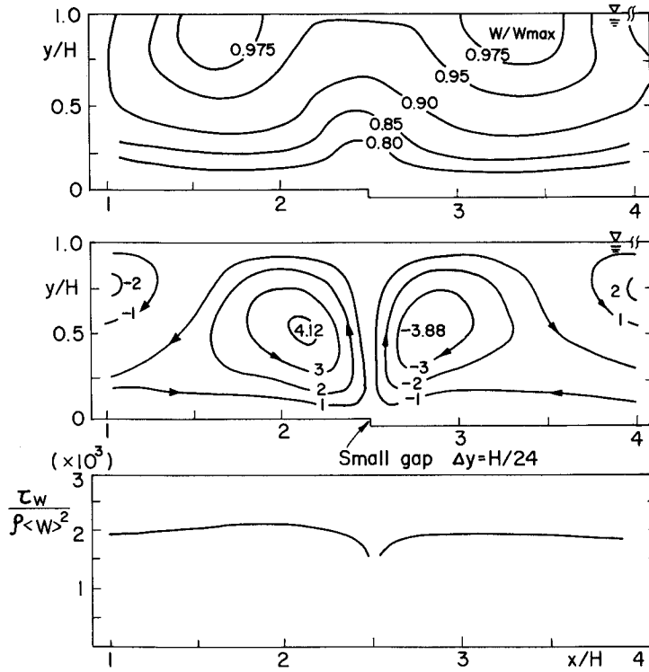
Fig. 21 The Low Flood-Plain Height Features : W/W_{max} , 10^3 \phi / \langle W \rangle H , and 10^3 \tau_w / \rho \langle W \rangle^2 . W_{max} / \langle W \rangle = 1.20 and h/H = 23/24 .
