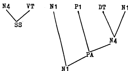
Fig. 3.3.4 An imcomplete tree by left-to-right parsing.
