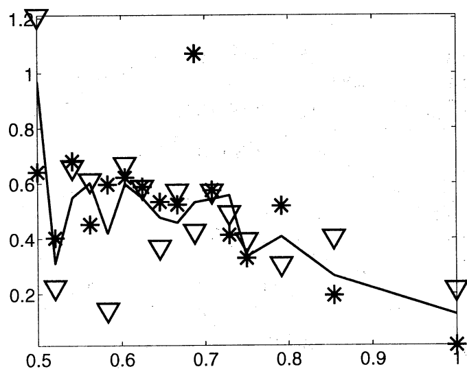
Figure 10: Pressure distribution for glass beads with 463 \mu\text{m} average diameter, monodisperse (425-500 \mu\text{m} ). Two different measurements at the same position, the line is drawn through the average of the dots to guide the eye.
