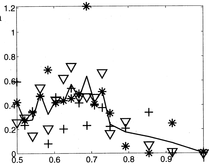
Figure 9: Pressure distribution for small glass beads and an average grain diameter of about 230 \mu\text{m} diameter, monodisperse (210-250 \mu\text{m} ). Three different measurements at the same position, the line is drawn through the average of the dots to guide the eye.
