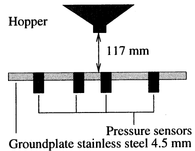
Figure 19: Experimental setup for the determination of the ground pressure.
