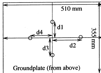
Figure 19: Experimental setup for the determination of the ground pressure.
