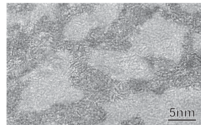
FIG. 2. Typical HREM image of Pd 42.5 Ni 7.5 Cu 30 P 20 metallic glass after annealing at 290^\circ\text{C} (below or near T_g ) for 10 h under ultrasonic vibrations of 0.35 MHz. The remaining amorphous fraction was estimated to be about 80% from the crystallization heat measured by differential scanning calorimetry. It can be clearly recognized that the amorphous domains are surrounded by crystallized walls that show lattice fringes. Ultrasonic vibrations are considered to accelerate crystallization of WBRs via \beta relaxation. The crystallized walls would be thin if annealing time is shortened. The sample for HREM was prepared by ion milling with cooling using liquid N 2 to prevent crystallization due to ion irradiation. For the sake of conspicuity of the boundaries, the amorphous-like regions are colored grey.
