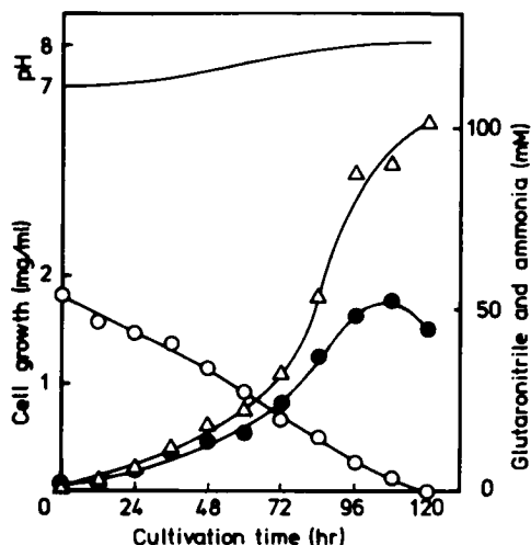
Fig. 1. Time Course of Growth of Pseudomonas sp. K-9.
