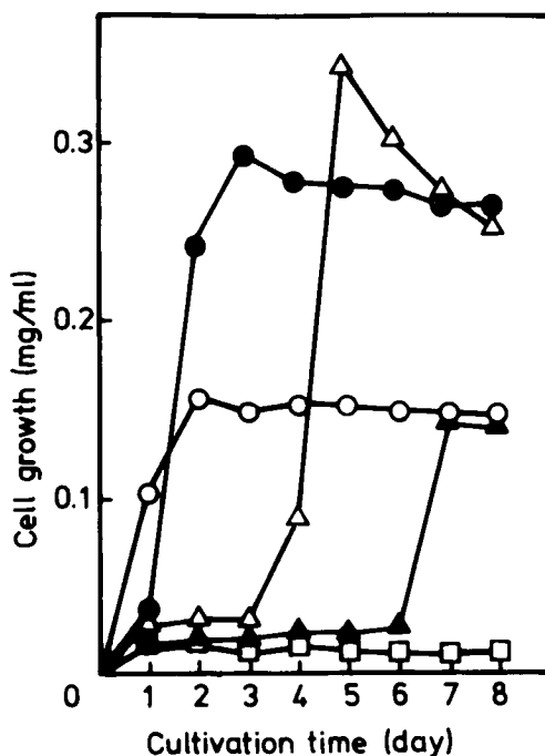
Fig. 2. Effect of Acrylonitrile Concentration on the Growth of Arthrobacter sp. I-9.
