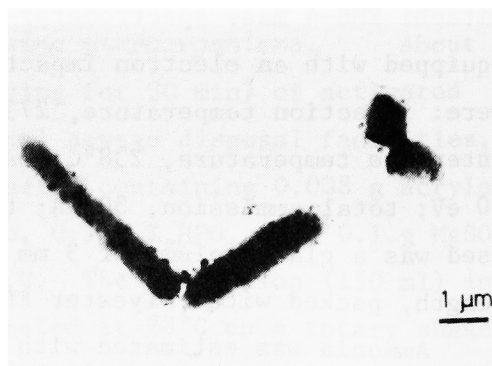
Fig. 1. Electron Micrograph of Strain I-9.
