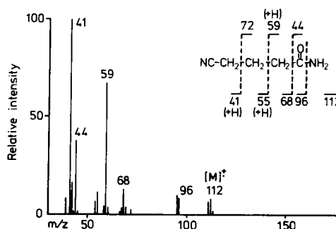
Fig. 5. Mass Spectrum of Compound C.
