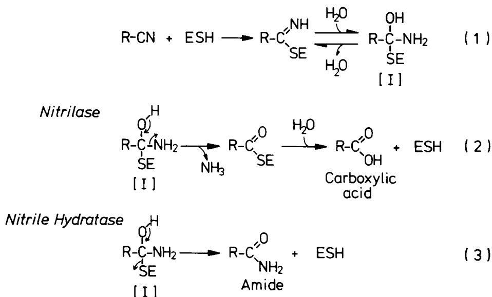
Fig. 7. Proposed Reaction Mechanisms of the Enzyme.
