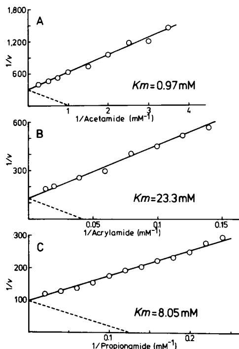
Fig. 6. Double Reciprocal Plots by the Enzyme.
