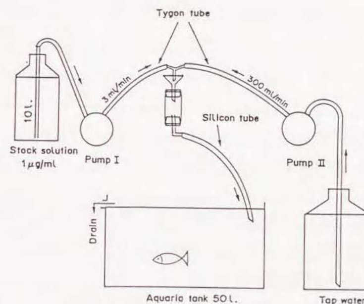
Fig.1 Experimental arrangement .
