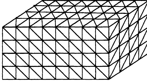
Figure 2: Tetrahedrization of domain \Omega .
