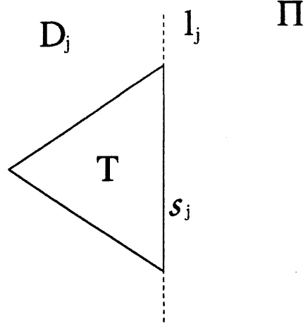
Figure 3: Half-plane D_j , triangle T , side s_j and line l_j .
