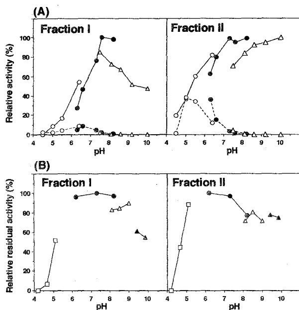
Fig. 2. Effects of pH on the activity (A) and stability (B) of the two cyclic ureide-hydrolyzing enzymes.
