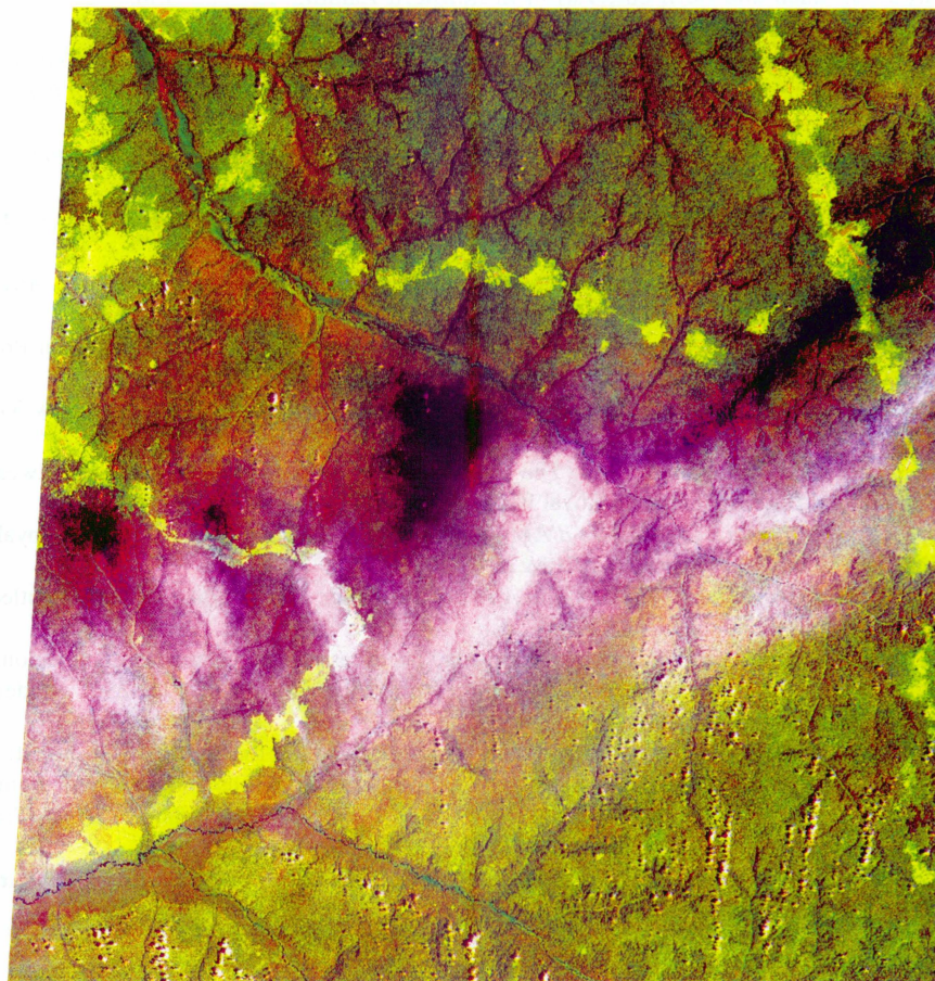
Fig. 11. Landsat image of the study area. Bands 5, 4, 3 (mid-infrared [ 1.55\text{--}1.74\ \mu\text{m} ], reflective-infrared [ 0.76\text{--}0.09\ \mu\text{m} ], and red [ 0.63\text{--}0.69\ \mu\text{m} ], respectively) are synthesized. These bands are indicated by red, green and blue in the picture.
